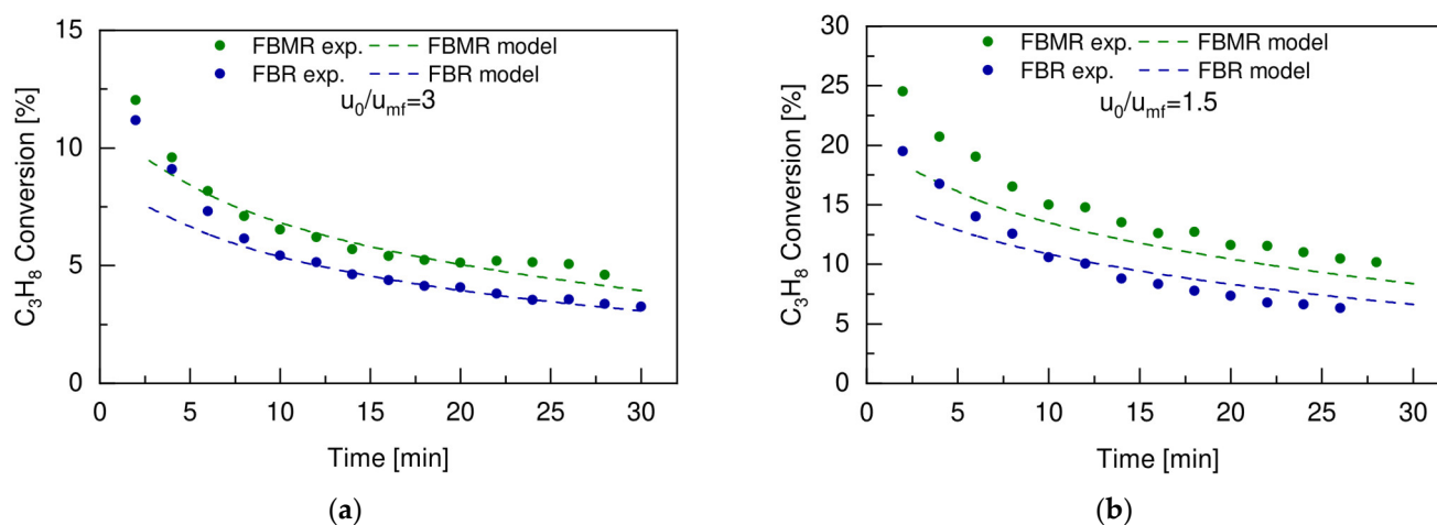
Figure 9. Propane conversion versus time obtained experimentally (dots) and with model simulation (dashed lines) for the FBR and the FBMR, working at 500 °C, 2 bar, with a feed composition of 30vol% C 3 H 8 -70vol% N 2 , with (a) u_0/u_{mf} = 3 and (b) u_0/u_{mf} = 1.5 .
