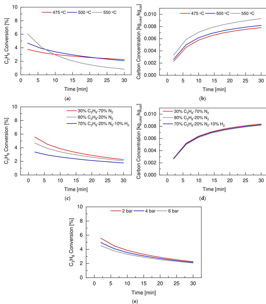
Figure 5. Effect of reaction temperature on (a) propane conversion and (b) carbon concentration, at 2 bar, u/u_{mf} = 3.75 and feed composition of 80vol% \text{C}_3\text{H}_8 and 20vol% \text{N}_2 . Effect of feed composition on (c) propane conversion and (d) carbon concentration, at 500 °C, 2 bar, u/u_{mf} = 3.75 . Effect of operating pressure (e) on propane conversion, at 500 °C, u/u_{mf} = 3.75 and feed composition of 30vol% \text{C}_3\text{H}_8 and 70vol% \text{N}_2 .
