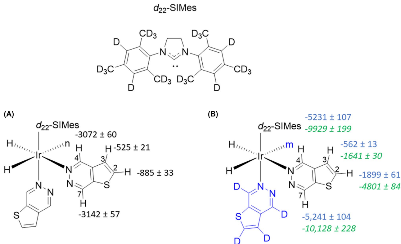
FIGURE 7 Comparison of hyperpolarization levels under (A) standard conditions of [\text{IrCl}(\text{COD})(\text{IMes})] and \text{T}[2,3\text{-}d]\text{P} in a 1:4 catalyst : substrate ratio (B) using a co-ligand with standard shake and drop (blue numbers) and using a co-ligand and shaking with a 60 G handheld shaker (green numbers). When the co-ligand was used it was in a 1:1:3 catalyst : substrate : deuterated co-ligand with [\text{IrCl}(\text{COD})(\text{IMes})] as catalyst, \text{T}[2,3\text{-}d]\text{P} as substrate and d_4\text{-T}[2,3\text{-}d]\text{P} as deuterated co-ligand. n = in plane \text{T}[2,3\text{-}d]\text{P} , m = in plane d_4\text{-T}[2,3\text{-}d]\text{P} (removed to aid the reader).
