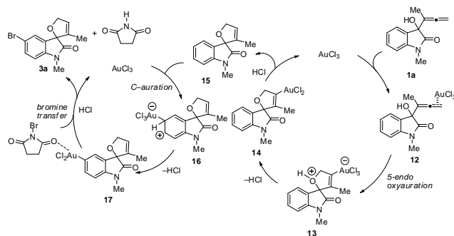
Scheme 5 Mechanistic explanation for the Au(III)-catalyzed arene bromination/spirocyclization reaction sequence of 3-allenyl 3-hydroxyindolin-2-one 1a .
