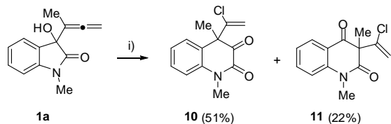
Scheme 4 Preparation of chlorinated lactams 10 and 11 in presence of NCS and [Ag(phen)OTf] . Conditions: (i) 10 mol % [Ag(phen)OTf] , NCS, MeCN, 75°C, 20 h. NCS = N -chlorosuccinimide.
