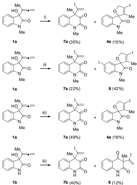
Scheme 3 Preparation of iodinated lactams 4 , 7 , 8 , and 9 in presence of I_2 , PhI(OAc)_2 , IPy_2BF_4 and AuCl_3 . Conditions: (i) I_2 , PhI(OAc)_2 , CH_2Cl_2 , RT, 12 h. (ii) 5 mol % AuCl_3 , I_2 , PhI(OAc)_2 , CH_2Cl_2 , RT, 1 h. (iii) 5 mol % AuCl_3 , IPy_2BF_4 , CH_2Cl_2 , RT, 1a : 1 h; 1b : 4 h.
