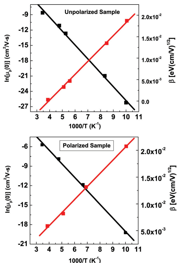
FIG. 4. (Color online) Temperature dependence of zero field mobility ( \mu_0 ) and \beta estimated from the TCLC model with Poole-Frenkel-type mobility for hole only devices for the (a) unpolarized sample and (b) polarized sample.
