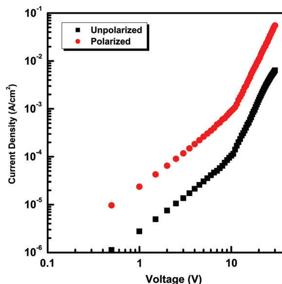
FIG. 1. (Color online) Room temperature J - V for single layer hole only PFO device with thickness of 120 nm: (a) unpolarized sample and (b) polarized sample.
