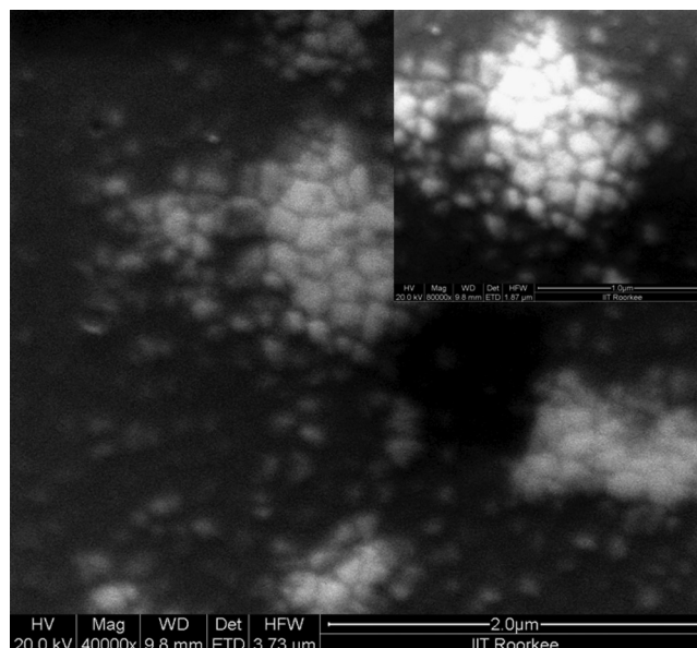
FIG. 6. SEM micrograph of charged thin film of PFO (inset shows magnified view).
