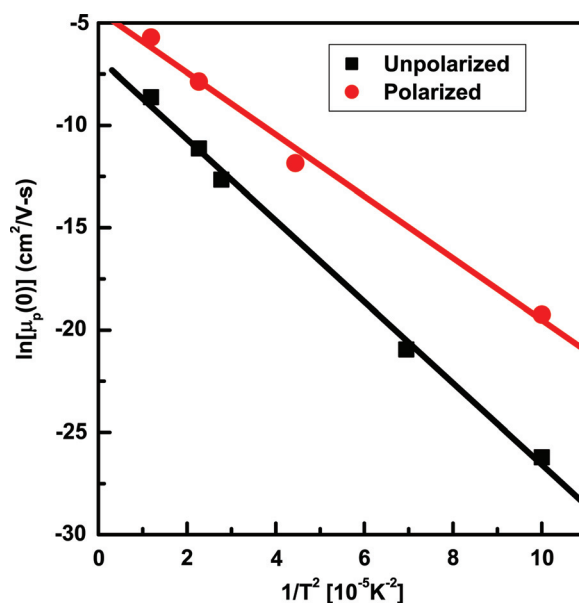
FIG. 5. (Color online) Temperature dependence of zero field mobility ( \mu_0 ) according to GDM for hole only devices for both samples, i.e., unpolarized sample and polarized sample.
