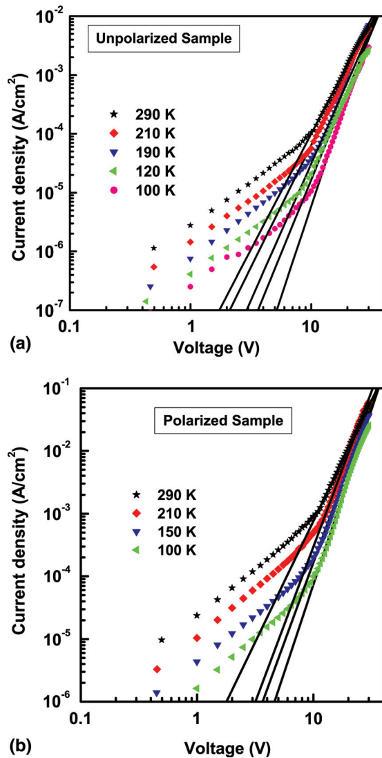
FIG. 2. (Color online) J - V characteristics of bulk limited current in ITO/PEDOT:PSS/PFO/Au at different temperatures. Experimental data are shown by symbols and solid lines represent the theoretical fits for (a) unpolarized sample and (b) polarized sample.
