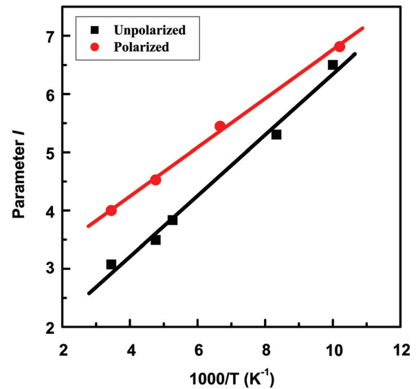
FIG. 3. (Color online) Temperature dependence of l obtained from theoretical fit according to the TCLC law to the experimental data (shown in Fig. 1) for the unpolarized sample and polarized sample.
