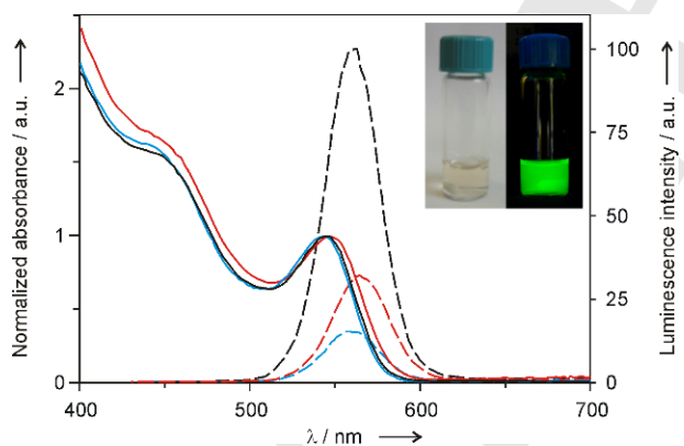
Figure 4. Absorption (full lines, left scale) and emission ( \lambda_{\text{exc}} = 420 nm; dashed lines, right scale) spectra of TOP/TOPO CdSe-5ZnS QDs (entry 5 in Table 1) in \text{CHCl}_3 (black), and of the same QDs in aqueous solution after cap exchange with DHLA - Na + (red) or DHLA - TMA + (blue). Inset: photograph of the DHLA - Na + capped QDs in water under ambient light (left) and upon UV excitation (365 nm).
