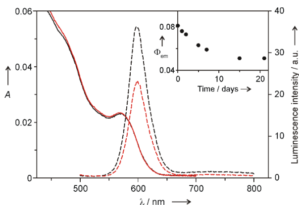
Figure 6. Absorption (full lines, left scale) and emission ( \lambda_{exc} = 480 nm; dashed lines, right scale) spectra of CdSe-5ZnS QDs (entry 7 in Table 1, 130 nM) capped with DHLA - Na + in water, freshly prepared (black) and after 21 days of storage at 5 °C (red). The inset shows the evolution of the luminescence quantum yield over time. Adapted by permission of the Royal Society of Chemistry. [26a]
