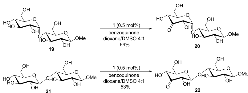
Scheme 2. Selective oxidation of methyl \beta -D-maltoside and methyl \beta -D-cellobioside.
