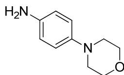
Figure 3. Chemical structure of 4-morpholinoaniline
