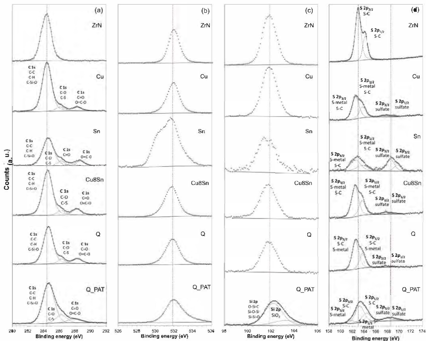
Fig. 5. XPS core levels of the characteristic PropS-SH elements on the different substrates (thin coatings on Cu, Sn, Cu8Sn, and Q): (a) C 1s, (b) O 1s, (c) Si 2p and (d) S 2p.
