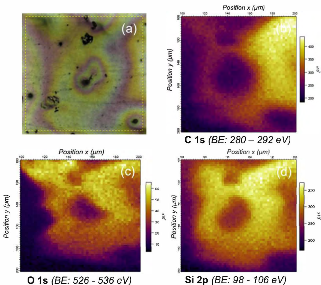
Fig. 3. PropS-SH on bare quinary bronze, free surface: optical image (a) and HR-SRPES maps for C 1s, O 1s and Si 2p (b-d). The optical image (a) shows the analysed area, corresponding to the same location of Fig. 2: the yellow dashed square indicates the area covered by HR-SRPES maps (side of the square = 100 \mu\text{m} ) (b-d). (For interpretation of the references to colour in this figure legend, the reader is referred to the web version of this article.)
