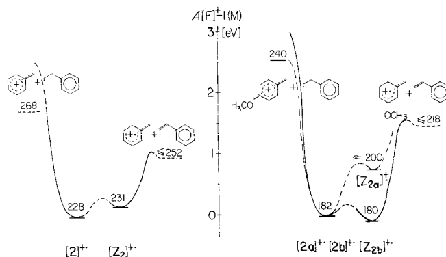
Figure 3. Enthalpy diagram for isomerization and fragmentation of the molecular ions of 2 (left) and of 2a (dashed lines --) and 2b (full lines —), in kcal mol -1 .
