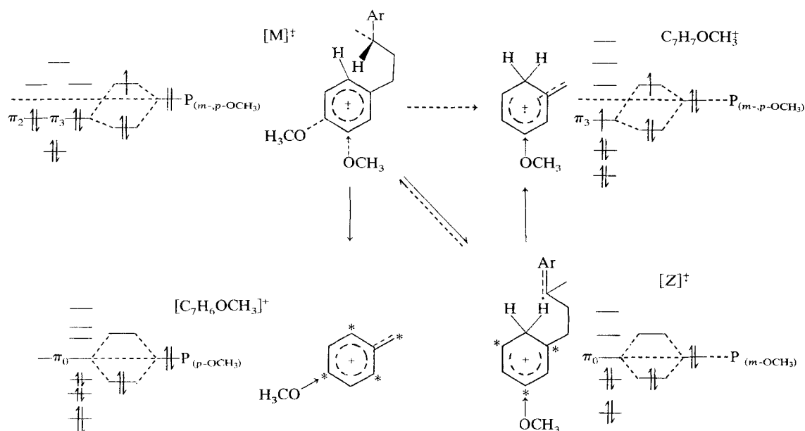
Scheme 4. Influence of p - and m -OCH 3 substituents on the formation of the C 7 ions, as considered in terms of PMO theory. Asterisks refer to 'active' positions in the odd AH cations.
