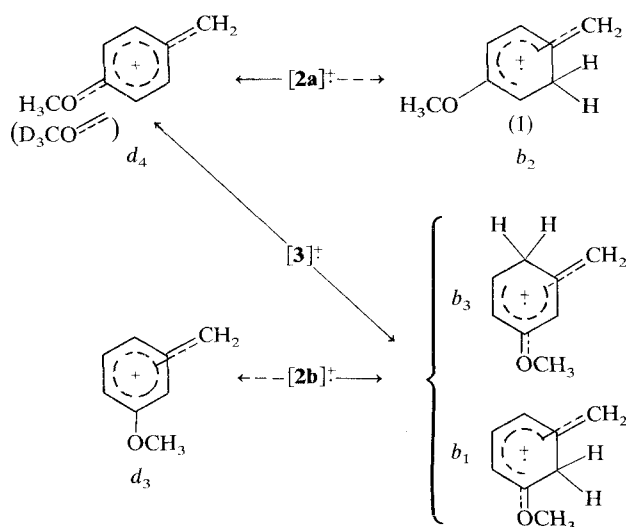
Scheme 3. Major fragmentation pathways (full arrows) of the 70 eV 'unstable' molecular ions of the methoxy substituted 1,3-diphenylpropanes.
