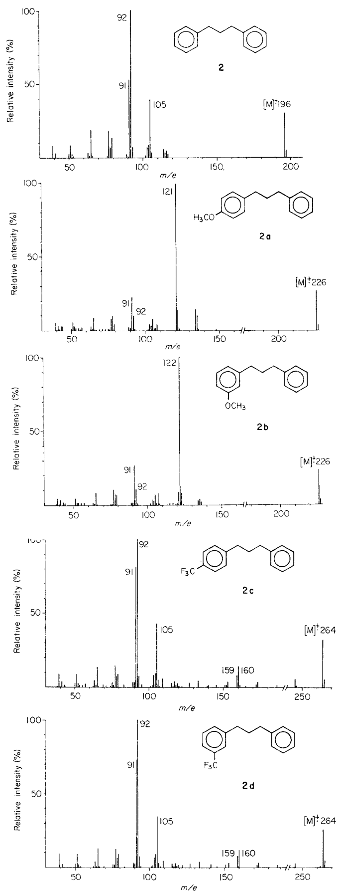
Figure 1. 70 eV mass spectra of 1,3-diphenylpropane (2) and substituted 1,3-diphenylpropanes (2a-2d).
