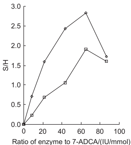
Fig. 4. Effects of the ratio of enzyme to substrate and substrate concentrations on the S/H. Reaction conditions: 25 °C, 20 mM phosphate buffer (pH=6.5) and molar ratio of PGME/7-ADCA=2:1. (□) 50 mM 7-ADCA, (◇) 150 mM 7-ADCA
