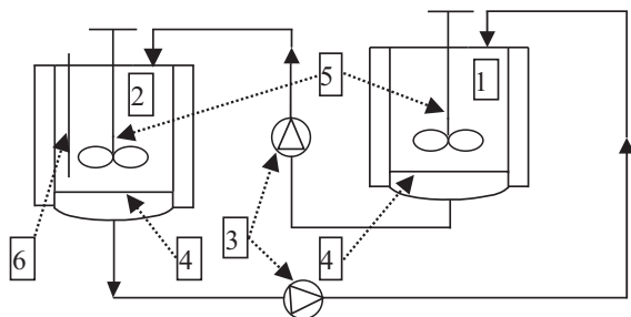
Fig. 2. Diagram of PGA-catalyzed synthesis of cephalexin with in situ product removal. 1. complexing reactor, 2. enzyme reactor, 3. peristaltic pump, 4. sintered glass, 5. mechanical stirrer, 6. pH controller
