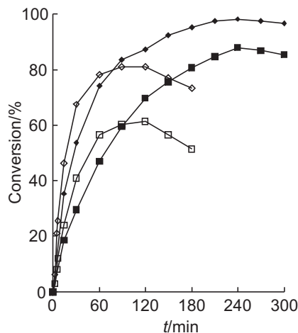
Fig. 5. 7-ADCA conversion at different substrate concentrations with or without ISPR. Reaction conditions: 25 °C, 20 mM phosphate buffer (pH=6.5) and molar ratio of PGME/7-ADCA=2:1. (□) 50 mM 7-ADCA without ISPR, (◇) 150 mM 7-ADCA without ISPR, (■) 50 mM 7-ADCA with ISPR, (◆) 150 mM 7-ADCA with ISPR
