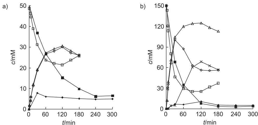
Fig. 6. Time courses of CEX and 7-ADCA at different substrate concentrations with or without ISPR. Reaction conditions: 25 °C, 20 mM phosphate buffer (pH=6.5) and molar ratio of PGME/7-ADCA=2:1. a) 50 mM 7-ADCA, b) 150 mM 7-ADCA. (□) 7-ADCA without ISPR, (■) 7-ADCA with ISPR, (◇) CEX without ISPR, (◆) CEX with ISPR; (△) CEX calculated by the conversion of 7-ADCA; (×) precipitated CEX without ISPR
