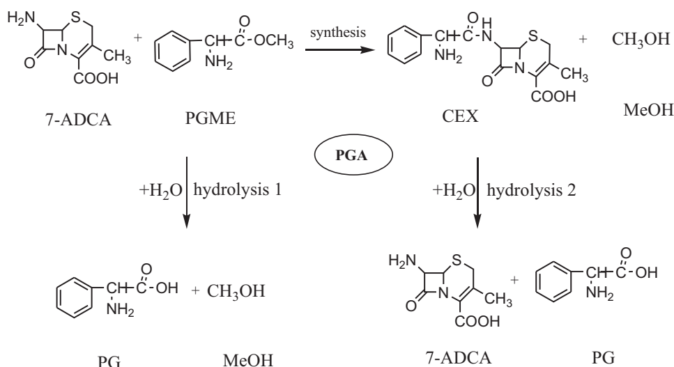
Fig. 1. Reaction mechanism of PGA-catalyzed synthesis of cephalixin. 7-ADCA=7-amino-3-deacetoxycephalosporanic acid, PGME=D(-)-phenylglycine methyl ester, CEX=cephalixin, MeOH=methanol, PG=D(-)-phenylglycine
