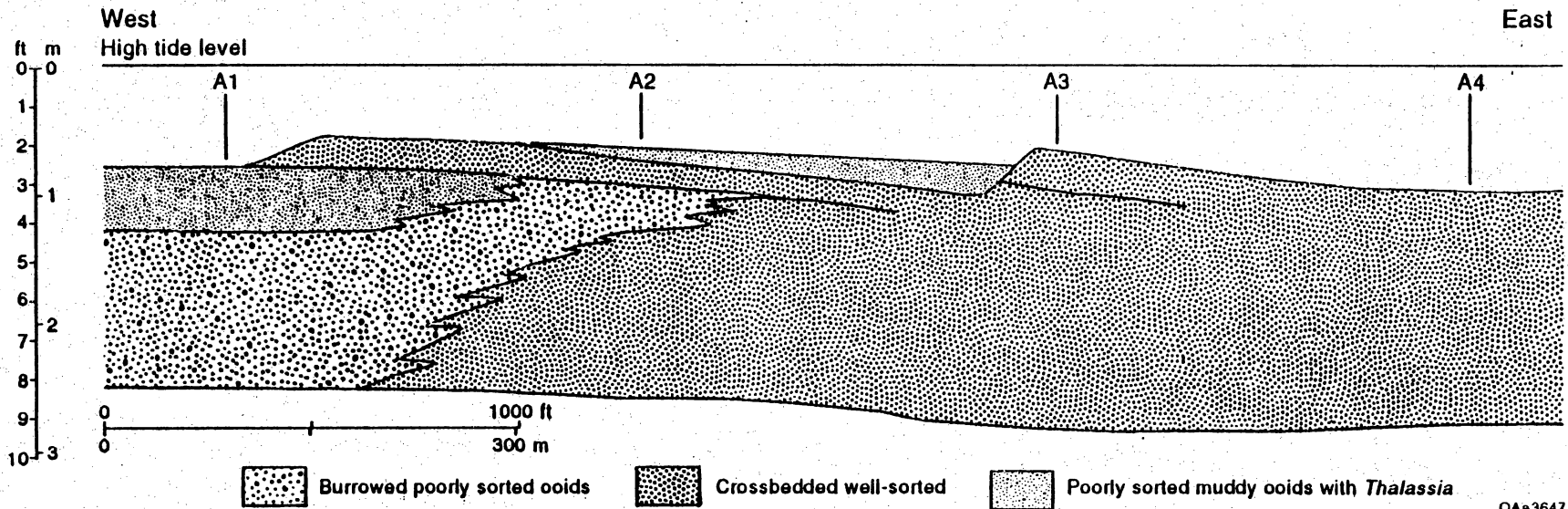
Figure 7. West-east cross section A-A' before passage of Hurricane Andrew. Location of section shown in figure 2. Core locations were leveled to a sea-level datum. At this location main part of ooid bar is 1.5 to 1.8 m (5 to 6 ft) thick and at least 760 m (2,500 ft) wide. Surface features result from two storm-washover bars, which have formed between them a low area in which some mud accumulated. Transition from crossbedded, well-sorted ooids into burrowed, poorly sorted ooids occurs on bankward side between A1 and A2. Position of seaward transition from crossbedded, well-sorted ooids into burrowed, poorly sorted ooids was not reached by this transect.
