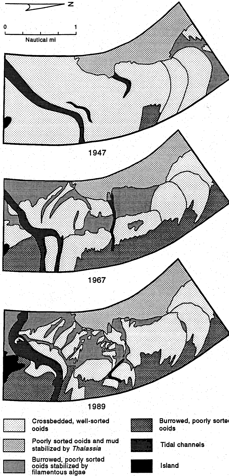
Figure 17. Surface sediment-distribution maps of the Joulter ooid shoal in (a) 1947, (b) 1967, and (c) 1989. Maps derived from aerial photographs (fig. 16) and cross sections (figs. 7, 8, and 9). Perspectives of 1947 and 1967 maps have been adjusted to oblique view of 1989.
