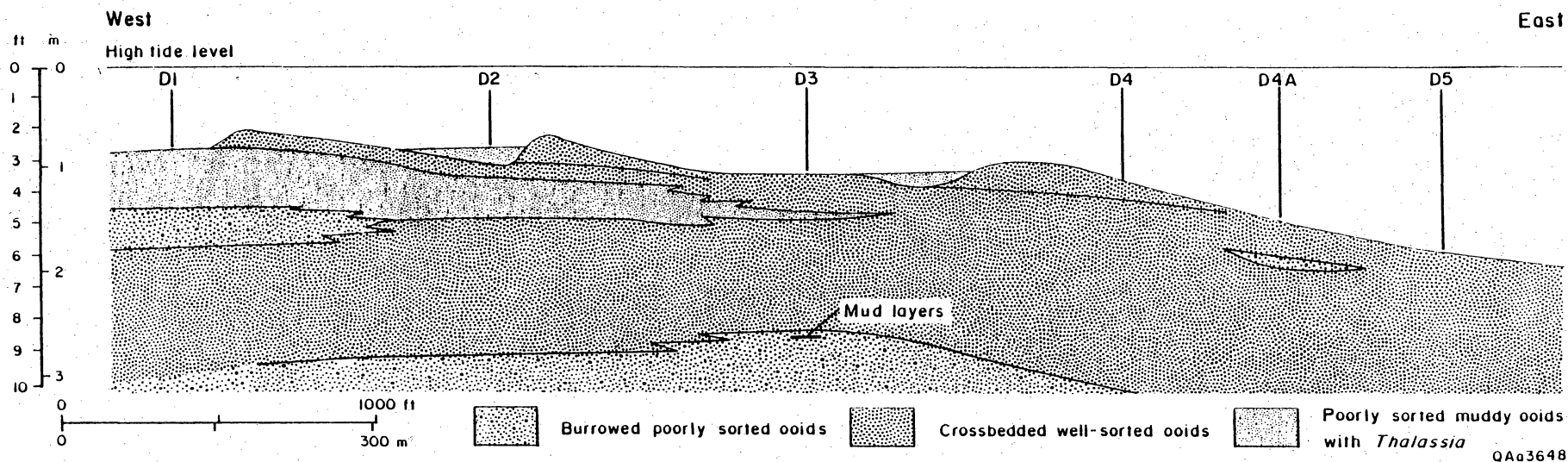
Figure 8. West-east cross section D-D' before passage of Hurricane Andrew. Location of section shown in figure 2. Ooid bar at this location is at least 1,220 m (4,000 ft) wide, and transition into burrowed, poorly sorted ooids was not reached on bankward or seaward side. Three storm-washover bars dominate the surface topography and form lows between that have served as sites of accumulation of carbonate mud along with the ooids. Mud layers shown in figure 13 lie at top of lower burrowed, poorly sorted ooids zone in D3.
