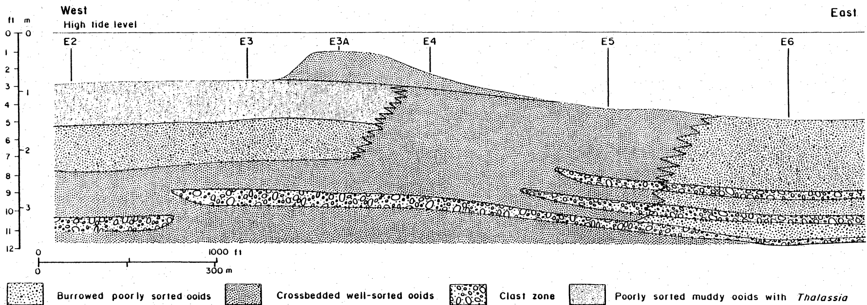
Figure 9. West-east cross section E-E' before passage of Hurricane Andrew. Location of section shown in figure 2. Ooid bar less than 610 m (2,000 ft) wide at this location. Transition from crossbedded, well-sorted ooids into burrowed, poorly sorted ooids occurs on bankward side between E3 and E4 and on seaward side between E5 and E6. Single large bar crest was deposited as a storm washover and consists of less than 0.6 m (2 ft) of crossbedded, well-sorted ooids that overlie poorly sorted muddy ooids containing Thalassia . Thick clast zones, shown in offlapping occurrence at base of section, are best represented on this cross section.
