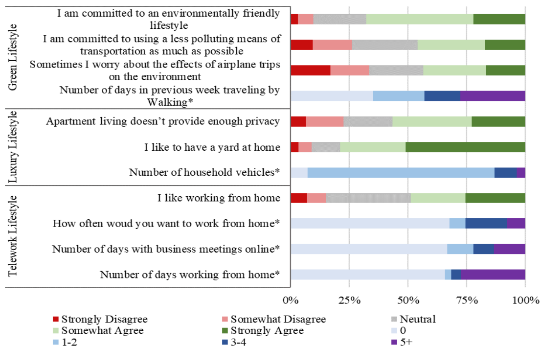
Figure 2: Distribution of Indicators of Latent Constructs
