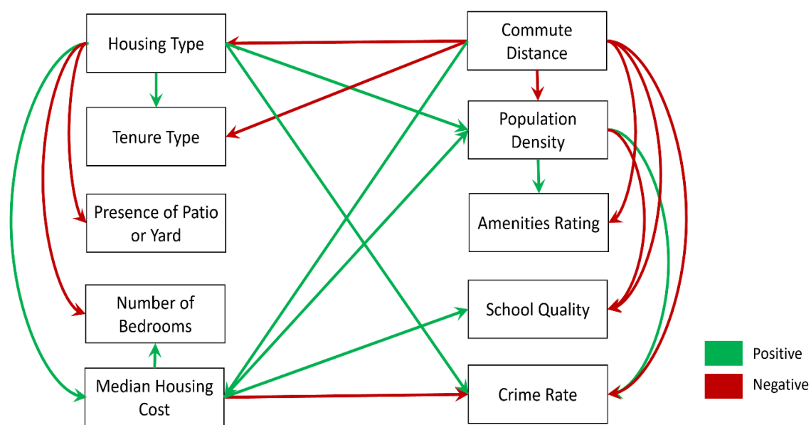
Figure 3: Structure of Endogenous Effects
