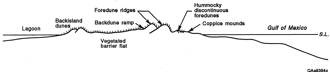
Figure 2. Generalized barrier island profile showing the locations of different dune types. Modified from White et al., 1978.
