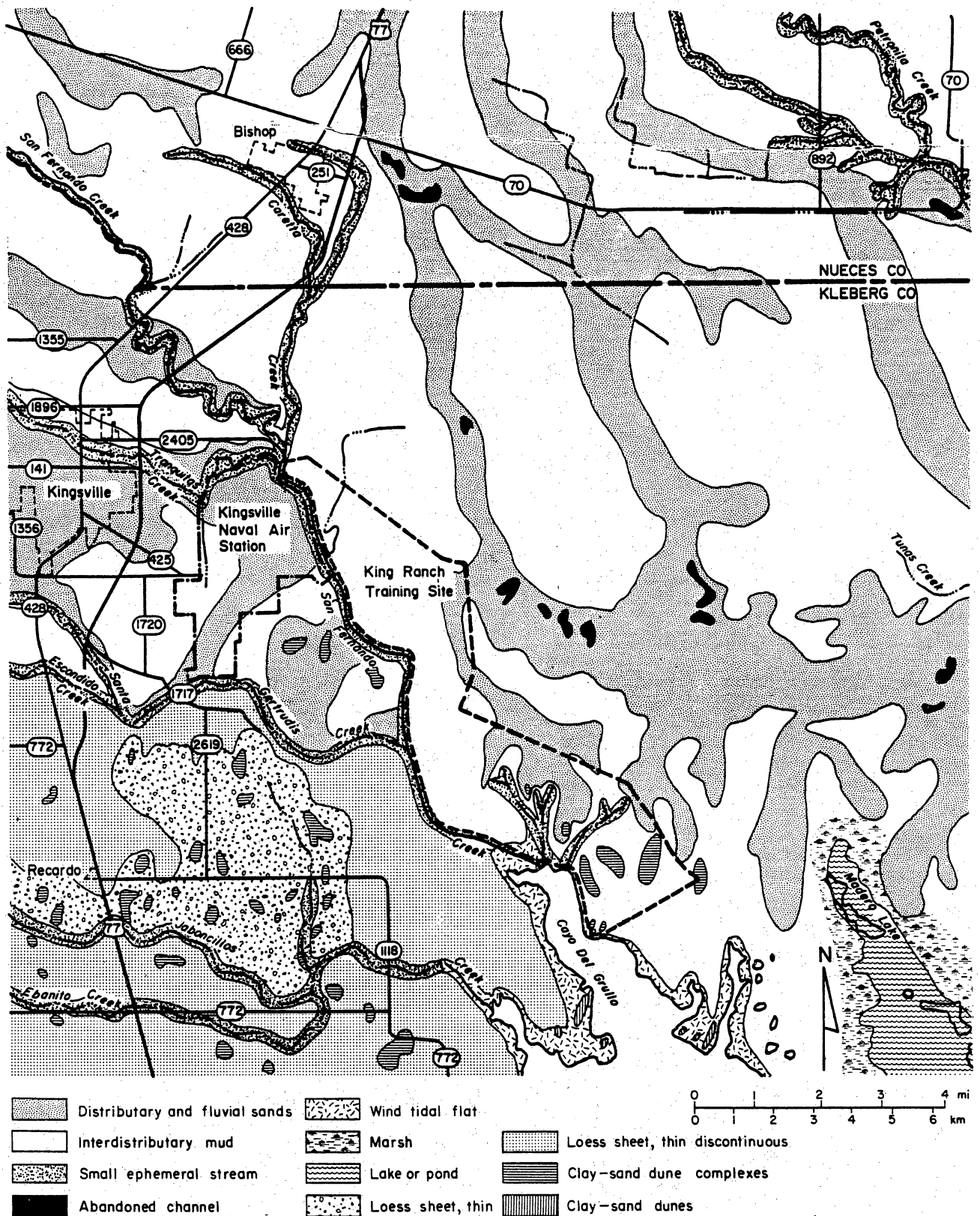
Figure 8. Surficial geologic units of the vicinity of the King Ranch training site of the Texas National Guard, modified after Brown and others (1980).
