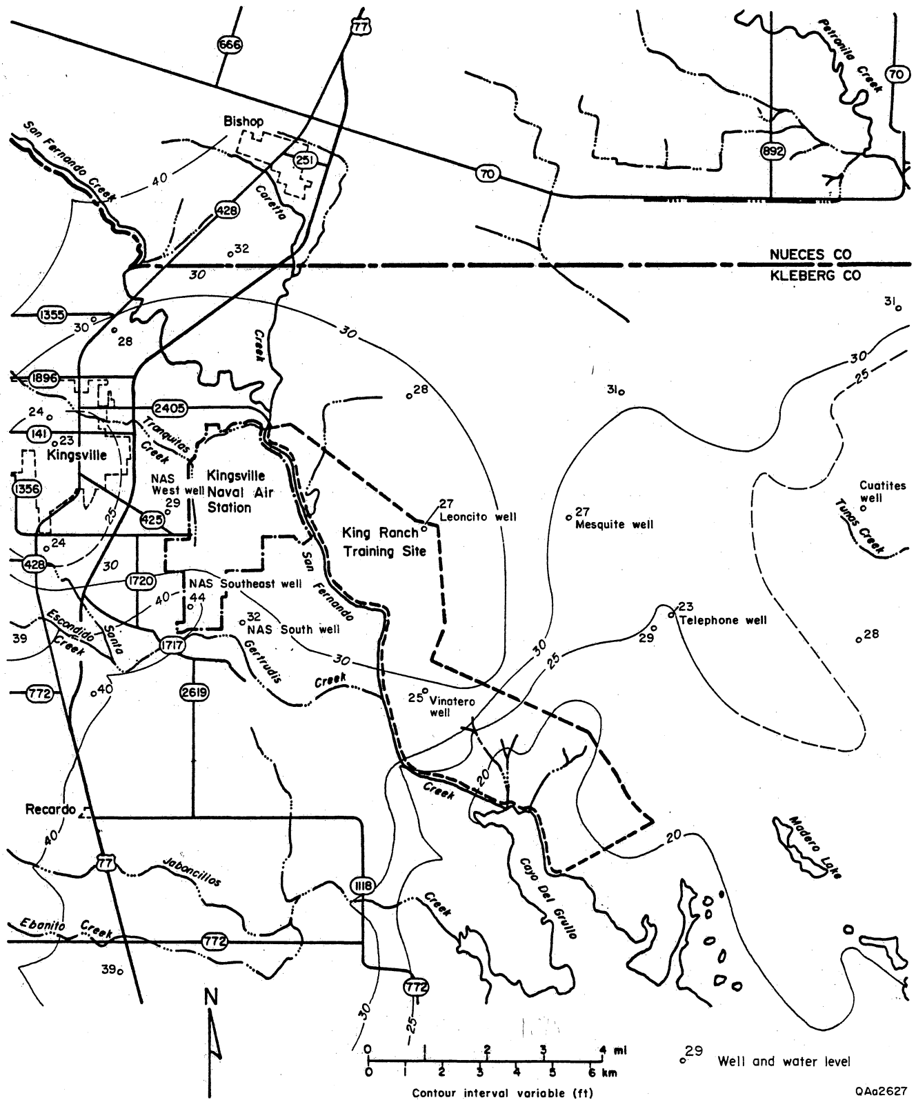
Figure 10. Potentiometric map of the Evangeline unconfined aquifer, 1933, in the vicinity of the King Ranch training site of the Texas National Guard. Data from the Texas Water Development Board.
