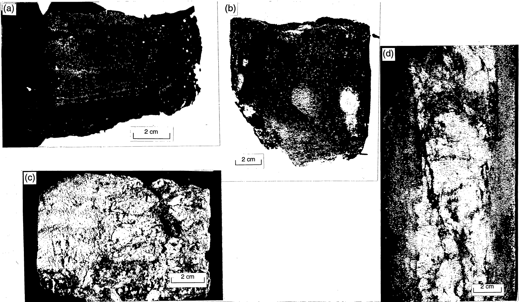
Figure 6. Unusual alteration found in sediments beneath Playa 5 and Pantex Lake. (a) Dark clay interlaminated with well-sorted silt. Playa 5, borehole 8, 7.5 ft. These sediments are interpreted as modern sediments infilling a scour pit beneath the sewage pipe outfall. (b) Dark stain in sand. Playa 5, borehole 8, 14.6 ft. This dark stain has only been observed in this borehole beneath the sewage pipe outfall and is interpreted to be staining from organic material carried by recharging fluids. (c) Limonite stain along root traces and other sedimentary structures in light-colored bleached sand. Playa 5, borehole 14, 22.5 ft. Limonite is more abundant in sediments beneath Playa 5 than in the unmodified playas examined in the preceding phase of the study. (d) Limonite and gray clay fill cracks and root traces in light-colored bleached lacustrine sand. Pantex Lake, borehole 15, 61.5 ft. Clay translocation and possibly limonite precipitation in this deep sample may reflect relict flow conditions from ancient larger, possibly more perennial lakes that have occupied this basin.
