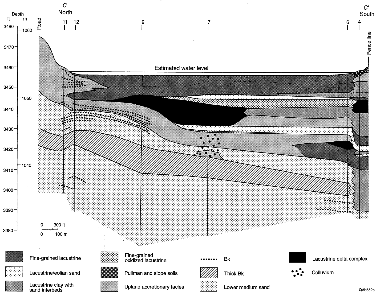
Figure 7. Pantex Lake north-south cross section C-C'. Cross section location shown in figure 3.
