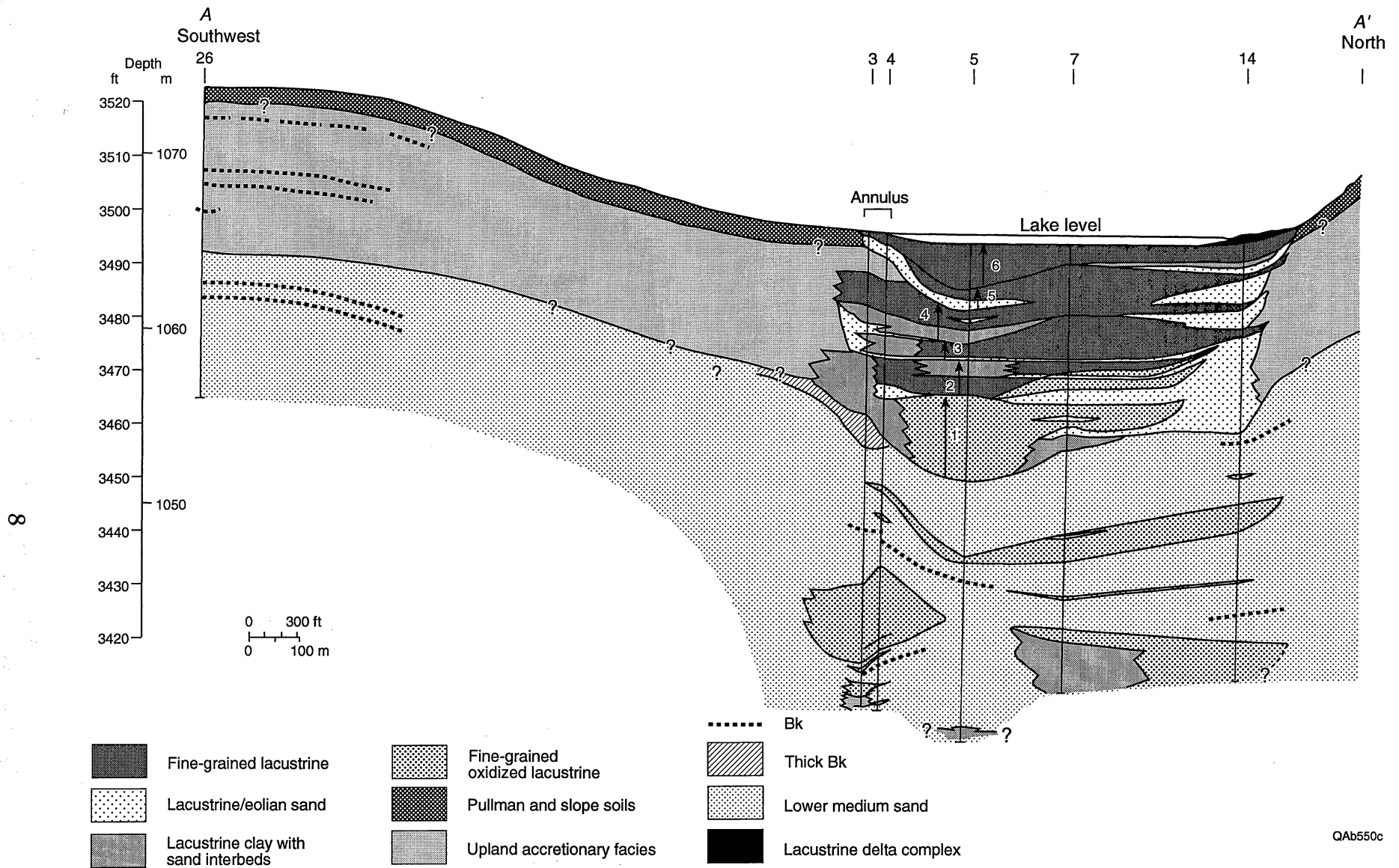
Figure 4. Playa 5 southwest-to-north cross section A-A'. Cross section location shown in figure 2. Depositional units 1 through 6 are discussed in the text.
