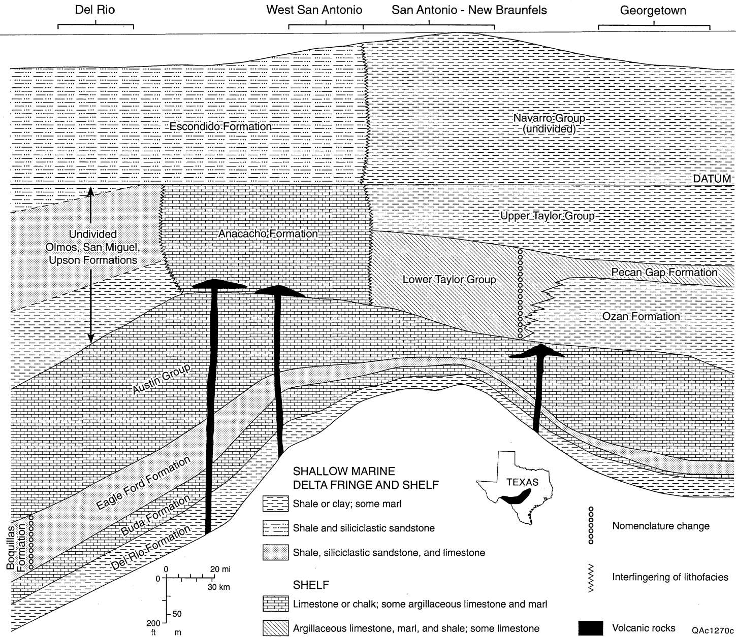
Figure 7. Diagrammatic correlation of Upper Cretaceous units across south-central Texas and subproject 1 map areas.
