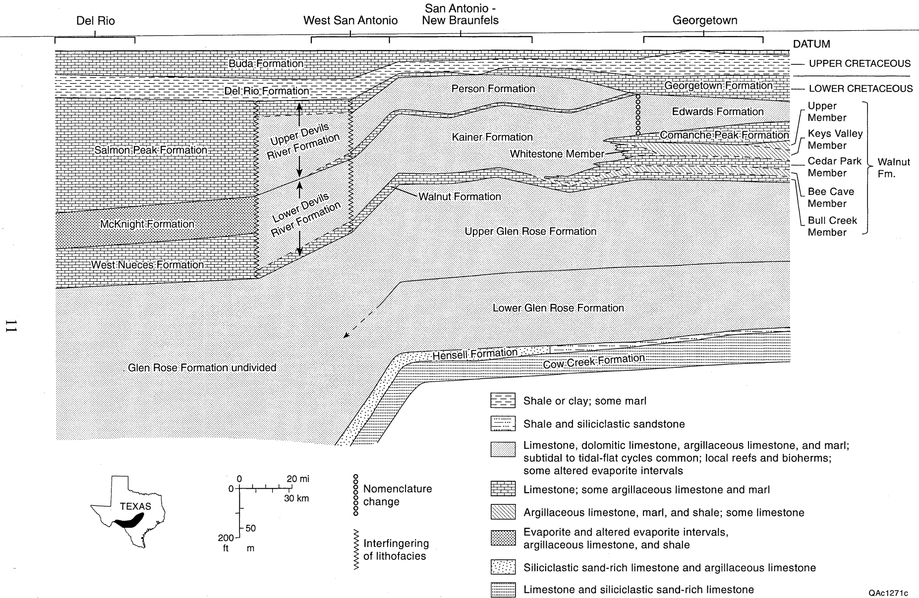
Figure 6. Diagrammatic correlation of Lower Cretaceous units across south-central Texas and subproject 1 map areas.
