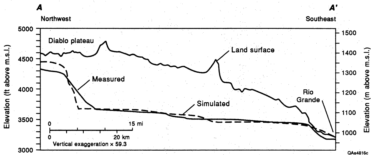
Figure 43. Comparison of measured and simulated potentiometric surface shown in cross section for model scenario 2 (horizontal to vertical anisotropy = 100:1). Simulated potentiometric surface obtained by using the simulated head value in the uppermost saturated cell in each column of the model.
