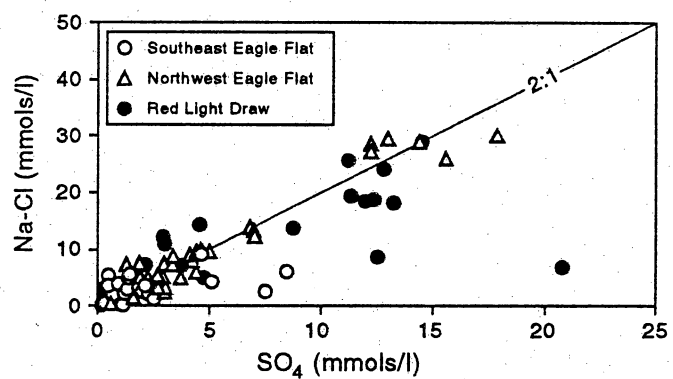
Figure 18. Binary plot of (Na-Cl) versus \text{SO}_4 for all areas. The quantity (Na-Cl) represents excess sodium, or that amount not attributable to dissolution of NaCl. The points form an upward-sloping trend with an approximate slope of 2:1. This is interpreted as an indicator of the gain of Na through exchange reaction with Ca derived from the dissolution of gypsum. The slope of 2:1 is what would be expected in a divalent/monovalent cation exchange process.
