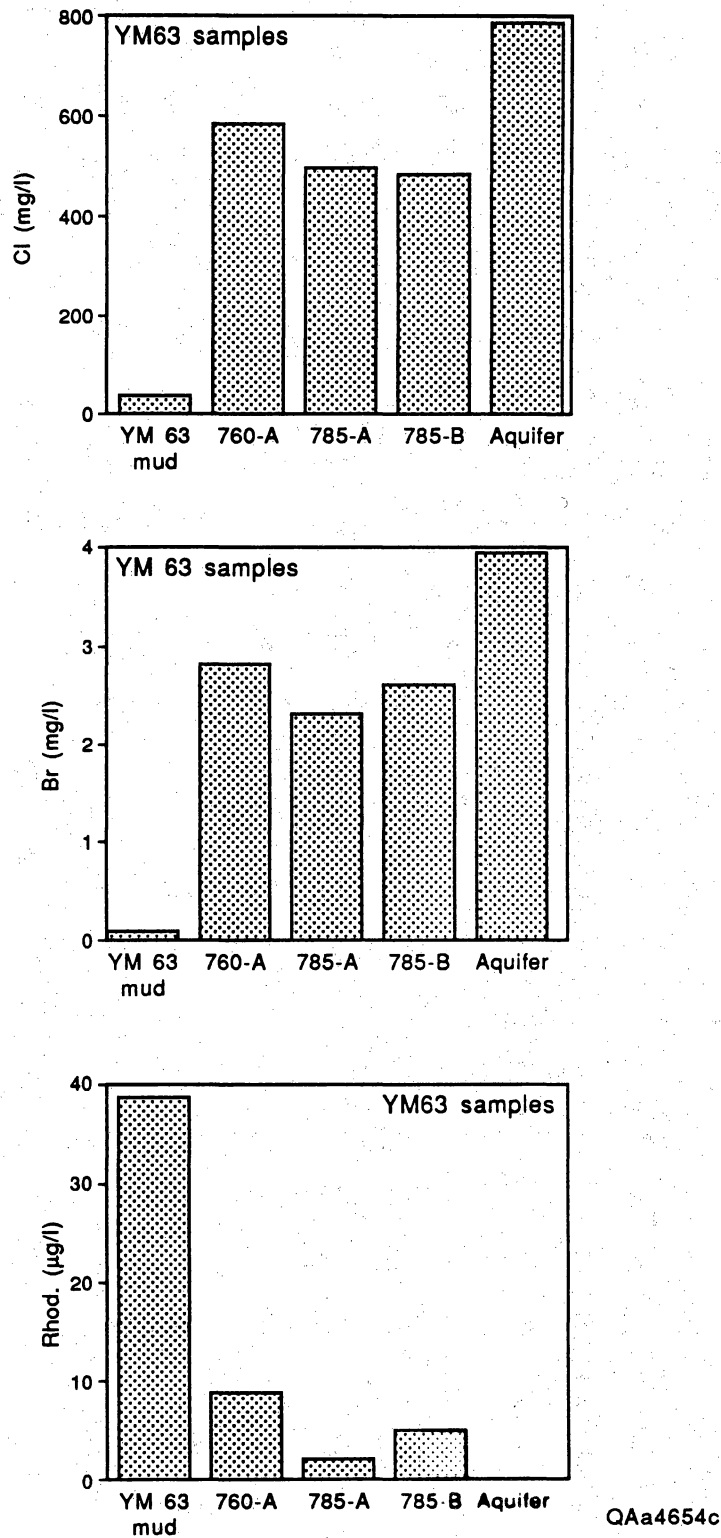
Figure 33. Comparison of conservative anions and rhodamine dye in drilling mud, recovery waters from well test intervals, and water collected from the completed well at YM-63. Two test samples collected at 785 ft (785-a and 785-b) and one test sample collected at 760 ft (760-a). Results of analysis of a drilling mud sample (YM-63 mud) and a sample from the completed well are shown. Comparisons between conservative anions and rhodamine dye indicate that almost three-fourths of recovery water is formation water at 760 and 785 ft. These results, along with recovery rates, indicate considerable storage and yield from the semiconfining unit or semiconfining interbeds at YM-63. These results imply conditions similar to conceptual models 2 or 3 (figure 31) at YM-63.
