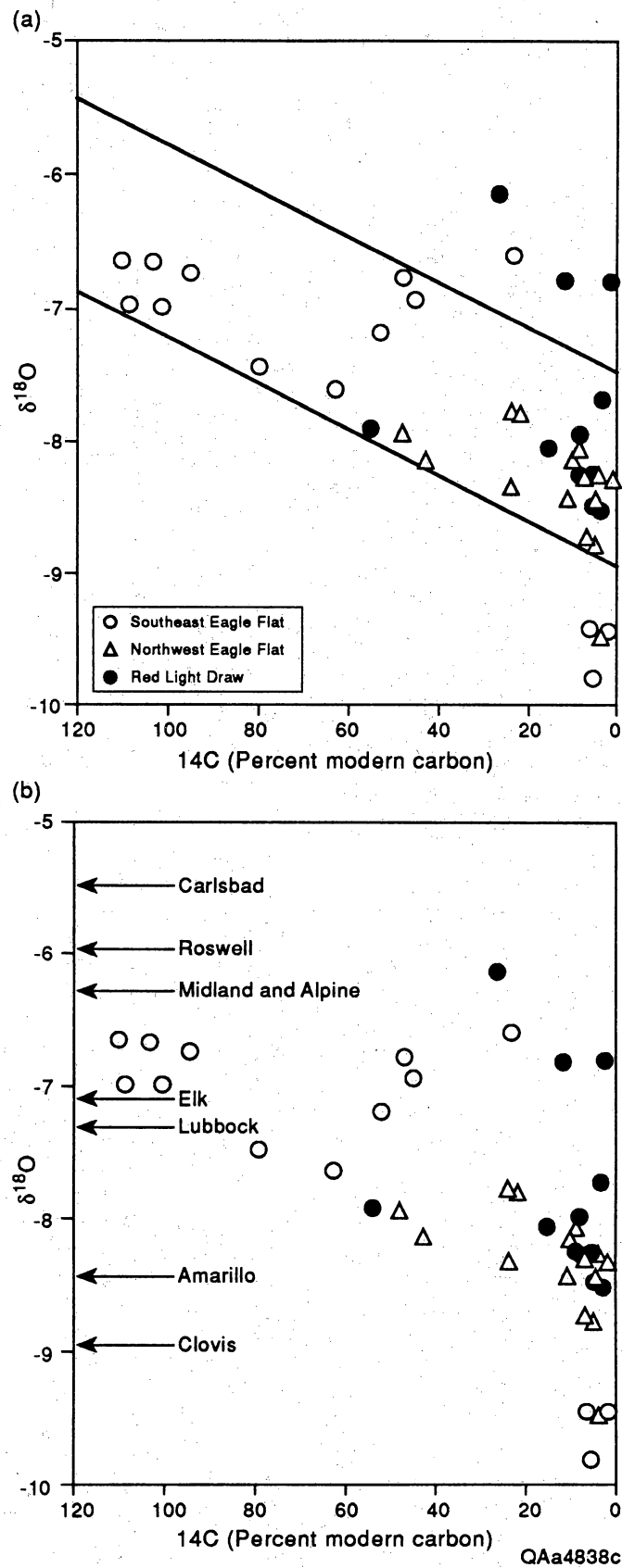
Figure 29. (a) Binary plot \delta^{18}\text{O} versus pmc in southern Hudspeth County ground water. Downward-sloping lines mark decreasing trend of \delta^{18}\text{O} values. (b) Binary plot of \delta^{18}\text{O} versus pmc in southern Hudspeth County ground water. Weighted-average \delta^{18}\text{O} values for precipitation from stations in West Texas and southeastern New Mexico are marked along the vertical axis. With few exceptions, ground-water d-values with less than 20 pmc are apparently lower than d-values from six of the eight locations.
