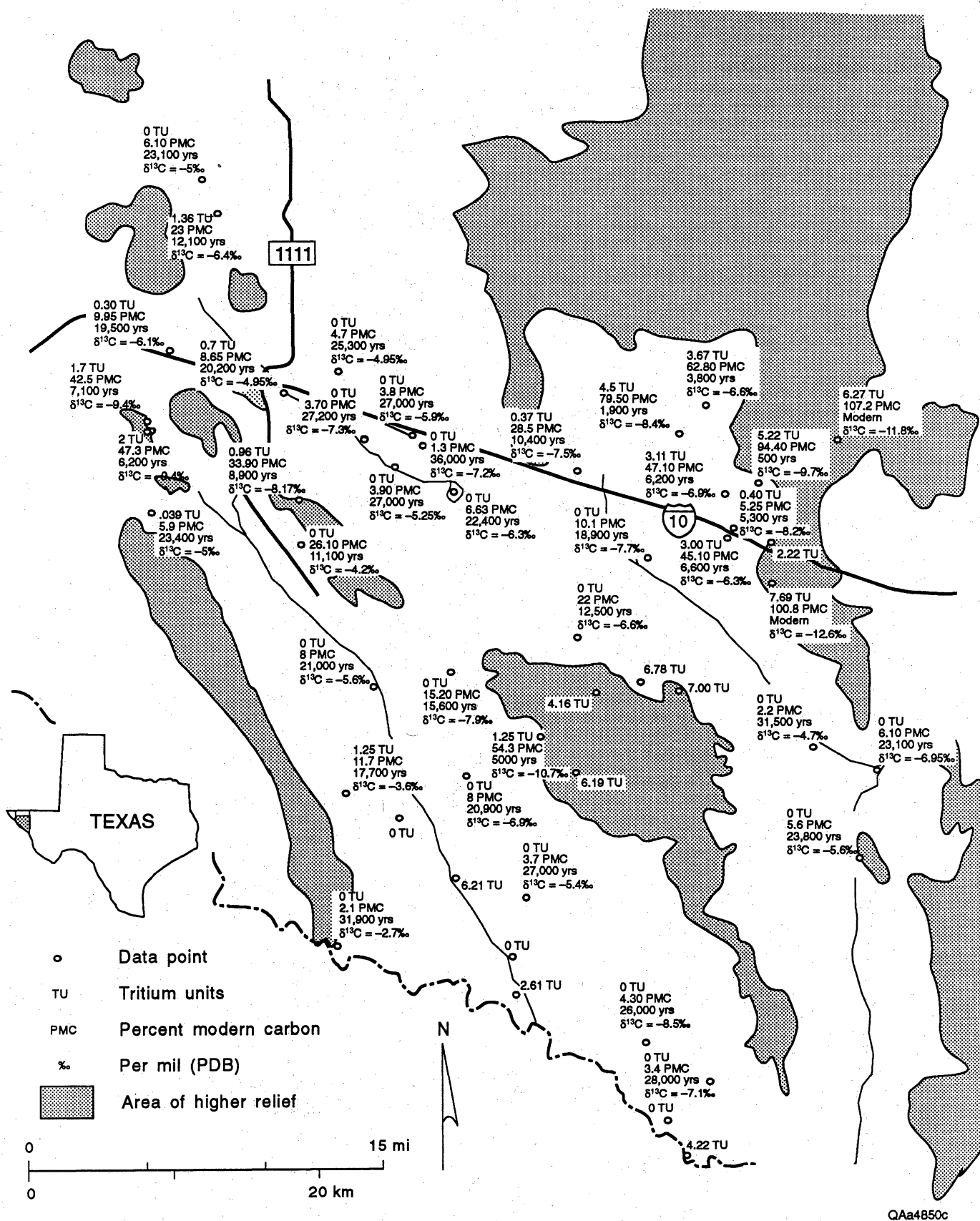
Figure 22. Map of ^3\text{H} , ^{14}\text{C} , and \delta^{13}\text{C} in southern Hudspeth County ground water. Carbon-14 is shown as pmc, along with uncorrected ages. Tritium is reported as Tritium Units (TU). \delta^{13}\text{C} is measured with respect to Peedee belemnite (PDB) standard.
