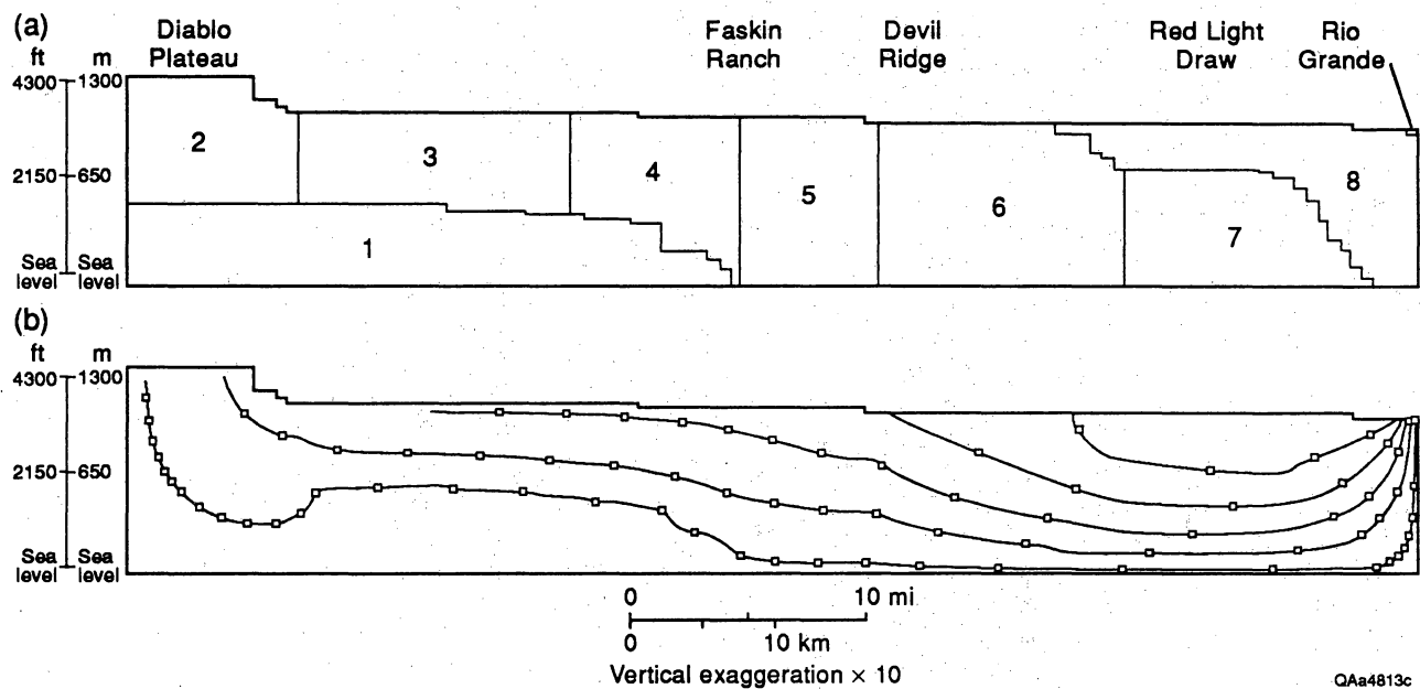
Figure 44. Particle tracking simulations showing pathlines moving underneath the Red Light Draw bolson; model scenario 2; heterogeneous, anisotropic units (horizontal to vertical anisotropy = 100:1). Each pathline marker indicates a travel time of 4,000 yr.
