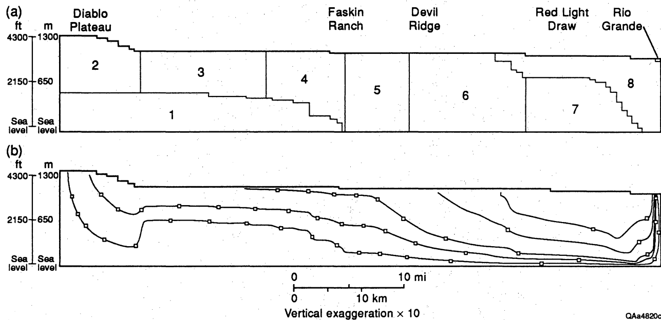
Figure 42. Particle tracking simulations showing pathlines moving underneath the Red Light Draw bolson; model scenario 1; heterogeneous, isotropic units. Each pathline marker indicates a travel time of 4,000 yr. Pathlines originating at the top of the model profile (zones 3 through 8) are representative of inflows from adjacent highlands (see fig. 41).
