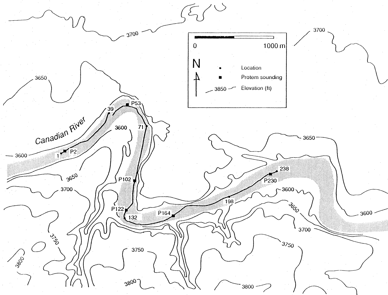
Figure 8. Topographic map of the Dunes area of the Canadian River (area D, fig. 2) showing station locations and sounding sites.
