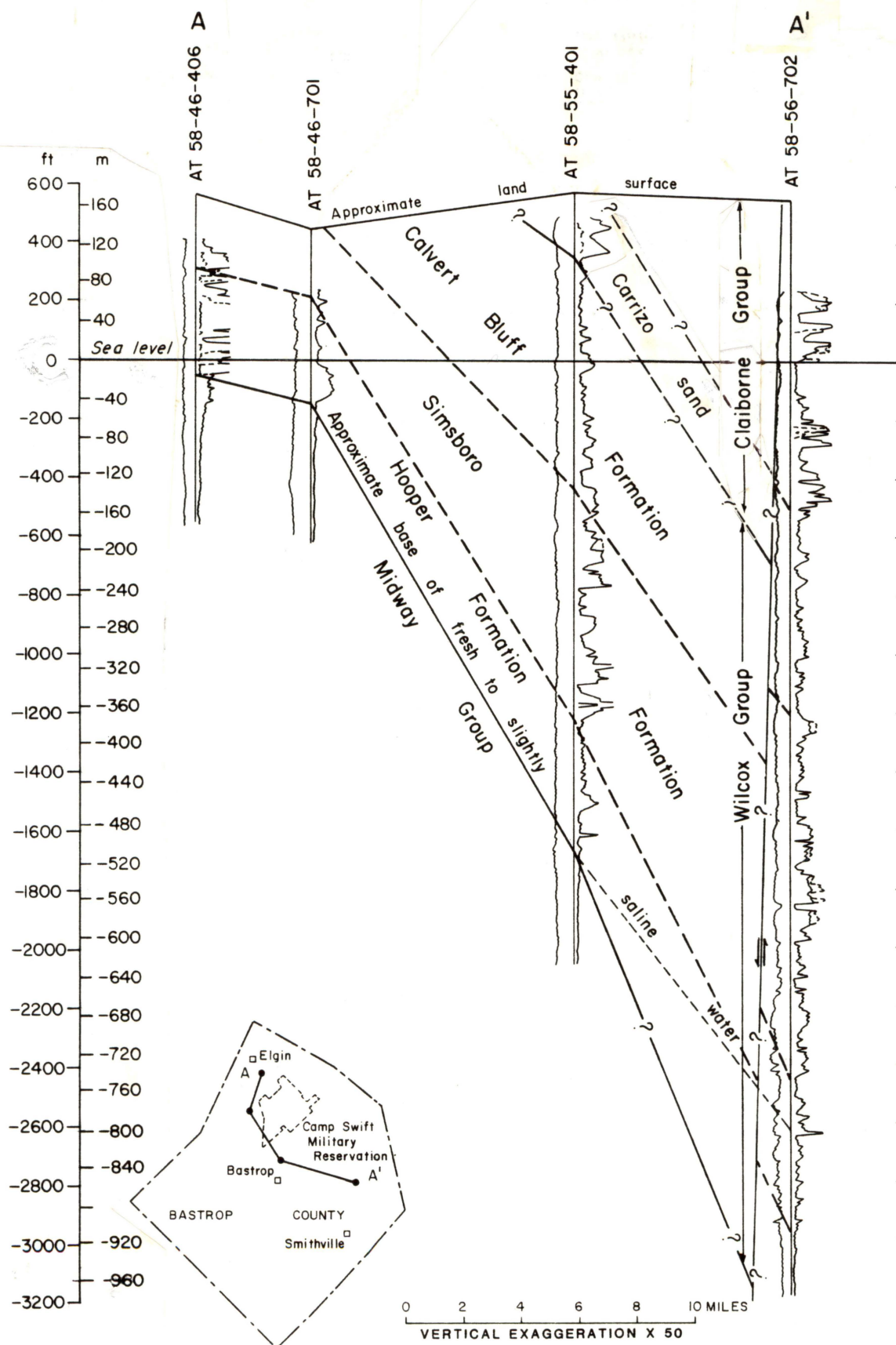
Figure 13. Schematic hydrogeologic cross section through the Camp Swift area. Ground-water flow is generally downdip and toward the south-southeast. Lines beside control wells are SP log (left side) and resistivity log (right side) curves. Modified from Follett (1970, fig. 25).
