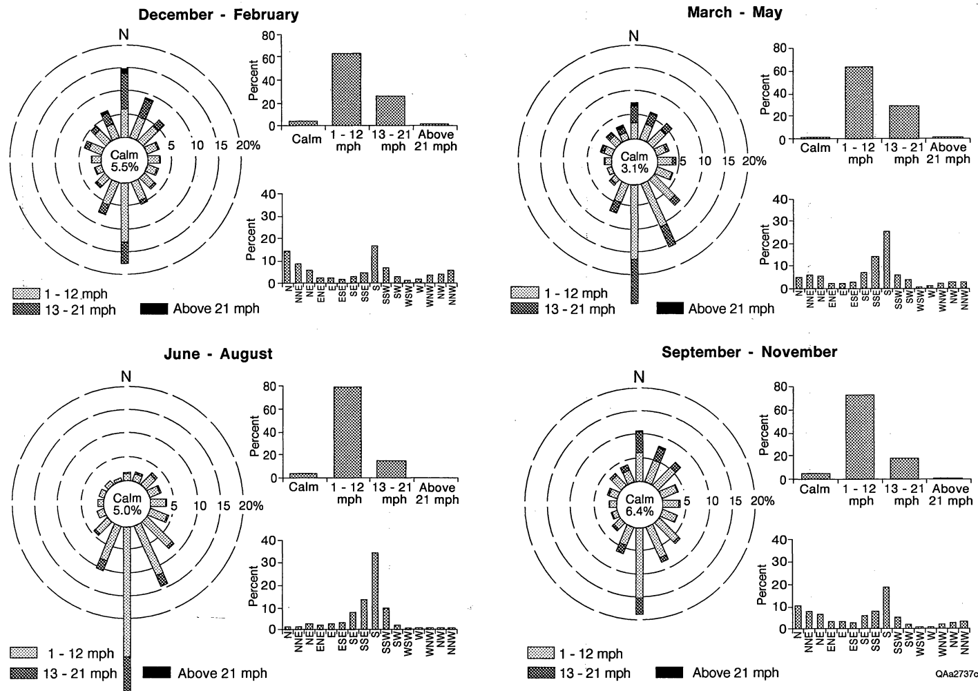
Figure 3. Average wind direction and speed at Robert Mueller Municipal Airport in Austin, 1961-1980. Arms of wind roses point in the direction from which the wind blows: for example, in the plot for December-February, the darkly shaded area on the arm pointing due south indicates that approximately 5 percent of the time the wind blew from the south at speeds between 13 and 21 mph. Data for these diagrams are given in appendix A; modified from plots presented in Larkin and Bomar (1983, p. 67-68 and 78-81). Bar diagrams beside each circular diagram indicate percentage of all winds by ranges of speed and by direction. Wind speeds of 13 mph and greater are capable of raising dust.
