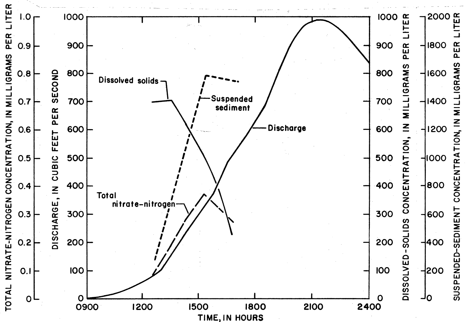
Figure 10. Changes in dissolved solids, total nitrate-nitrogen, and suspended-sediment concentrations with stream discharge at eastern gauging station on Big Sandy Creek, March 27, 1980. Plot shows that concentrations of major inorganic constituents are initially high, remain high during the earliest stages of storm runoff (due to leaching of soluble weathered material that has accumulated at the land surface since the last storm), and then decrease once they have been flushed; concentrations of suspended sediment and of nitrogen species increase dramatically during the early stages of storm runoff and then decrease as the supply of these materials is depleted. From Gaylord and others (1985, fig. 7.1-1).
