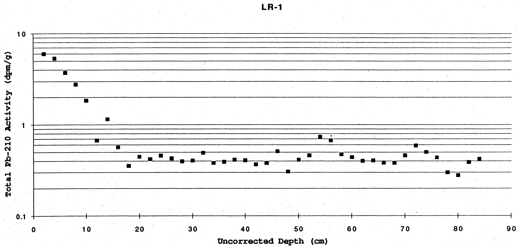
Figure 18. Profile of total ^{210}\text{Pb} activity in core LR-1. The profile shows a steep decline in activity in the upper few centimeters of sediments and then flattens out at depth.
