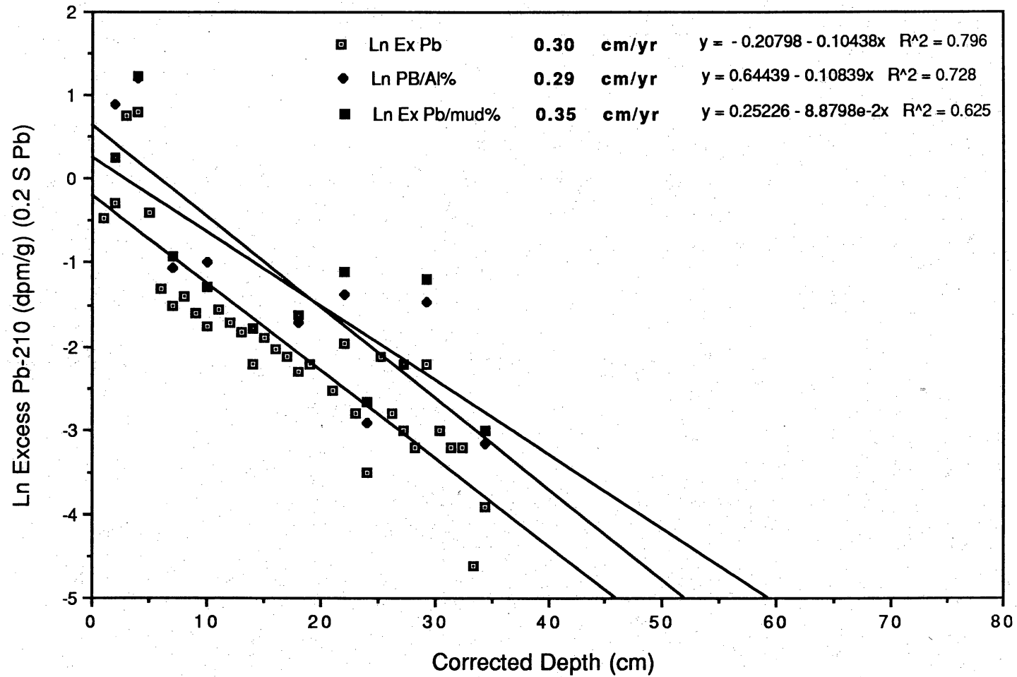
Figure 12. Effect of sand on the sedimentation rate in core LR-5. The relative high percentage of sand in this core causes a variation of approximately 0.5 mm/yr in the sedimentation rate .
