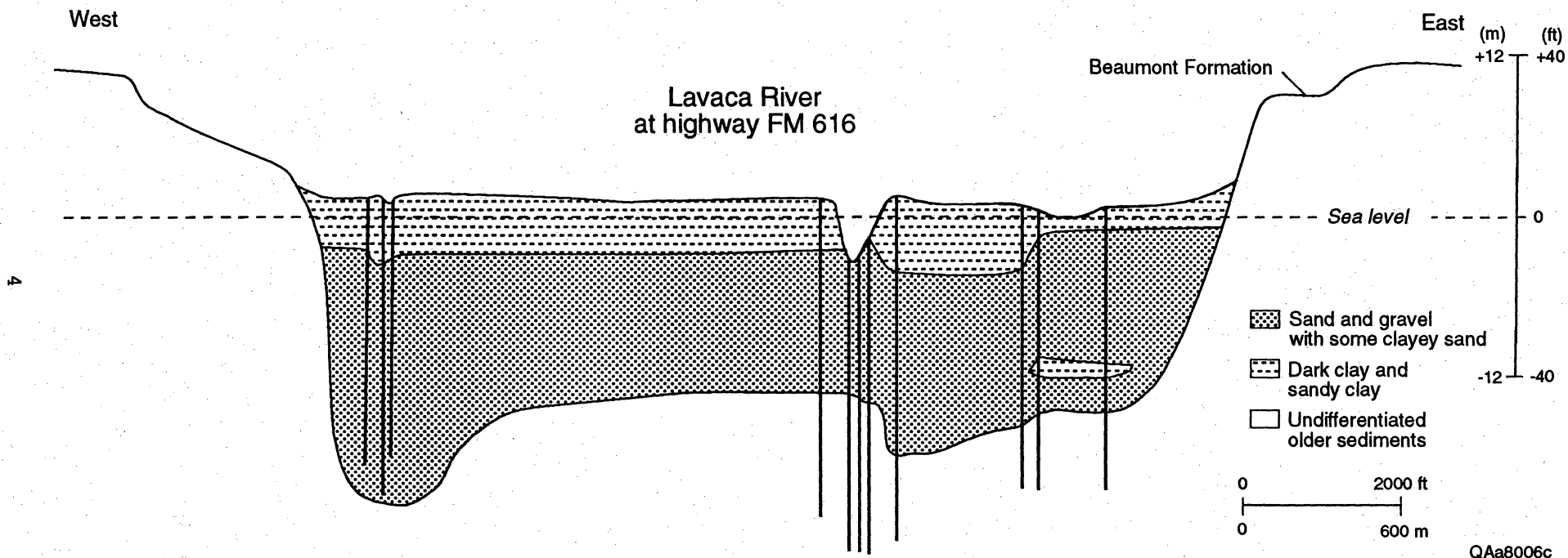
Figure 2. Cross section of Holocene sediments in the Lavaca River entrenched valley at FM 616. The lithology and thickness of sediments are based on geotechnical surveys made by the Texas Department of Transportation along FM 616.
