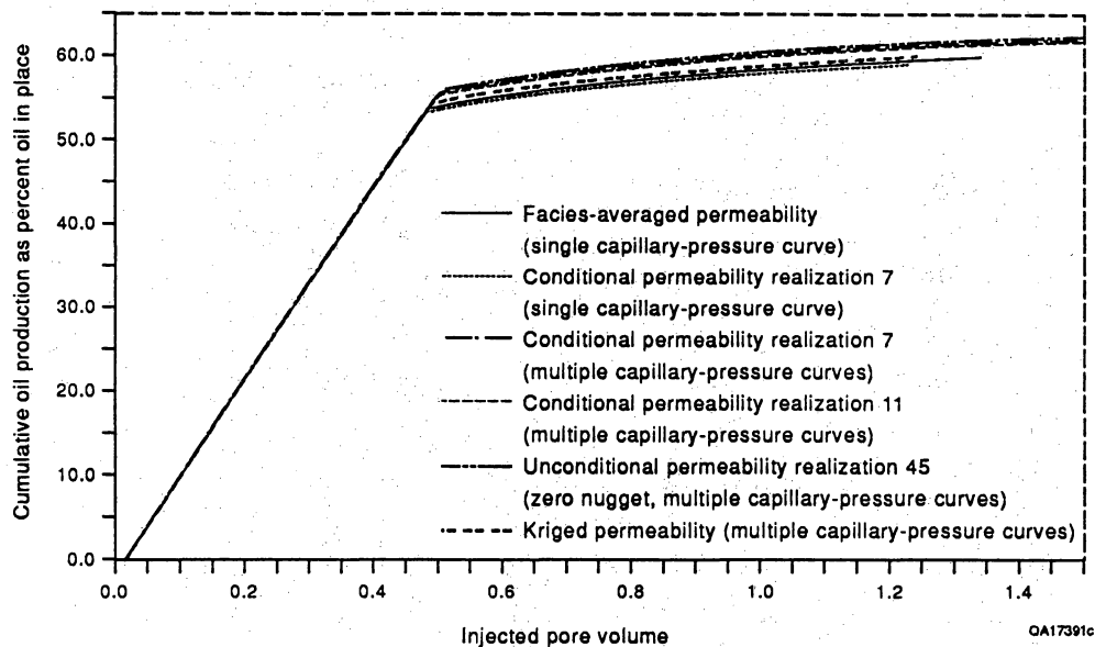
Figure 25. Cumulative oil production as percentage of original oil in place for waterflood simulations in parasequence 1.
