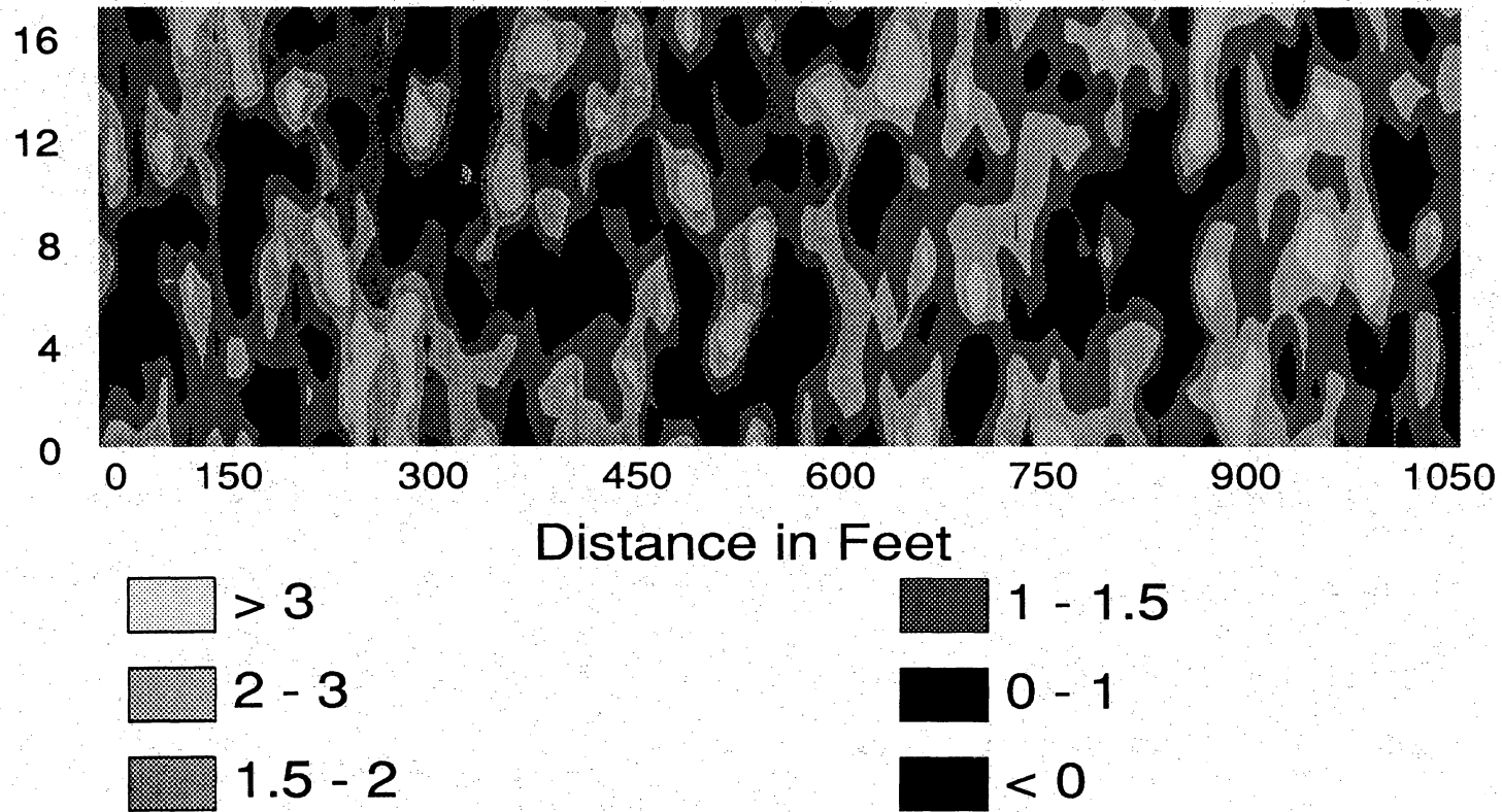
Figure 18. Unconditional permeability distribution of realization 45, representing low continuity of high-permeability zones.
