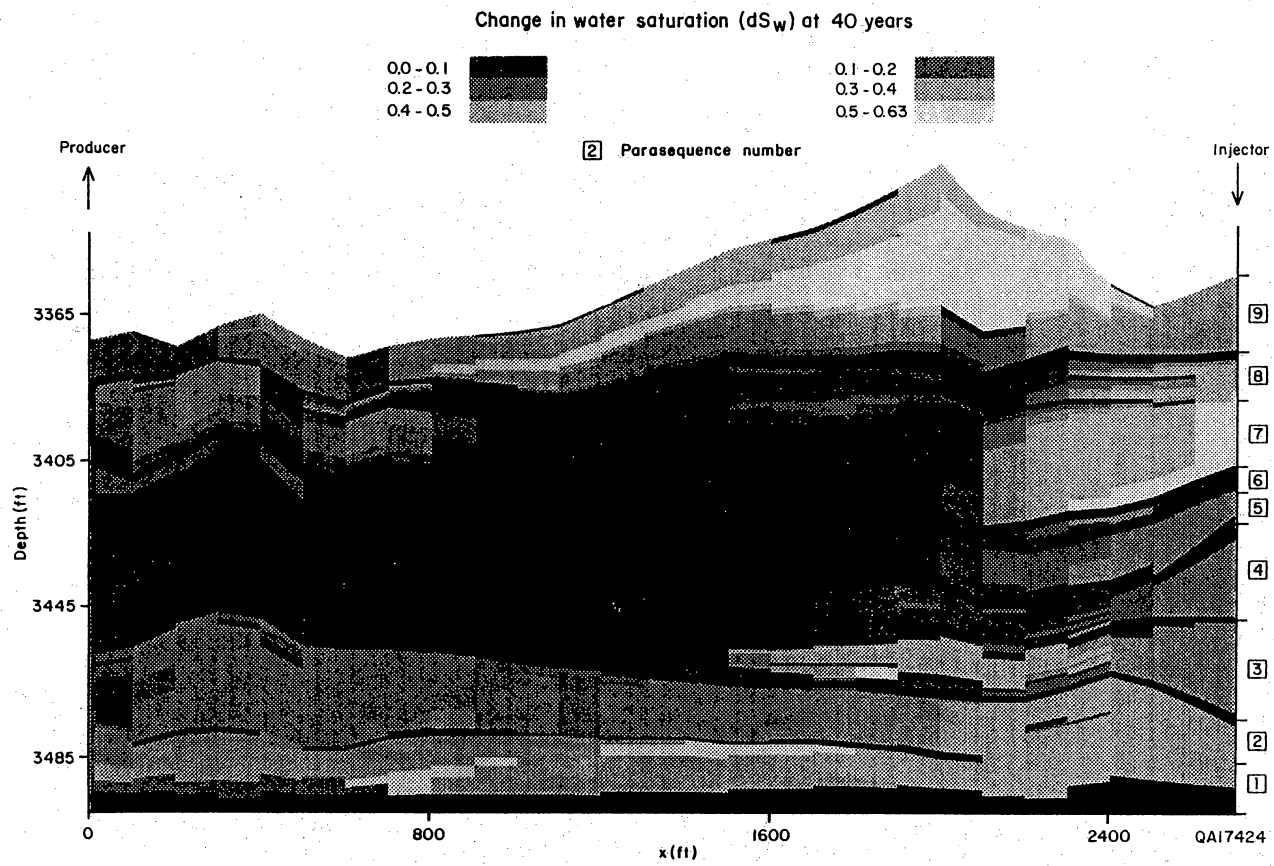
Figure 32. Computed changes in water saturation after 40 yr of waterflooding for simulation EC-R with inverse-injection pattern.
