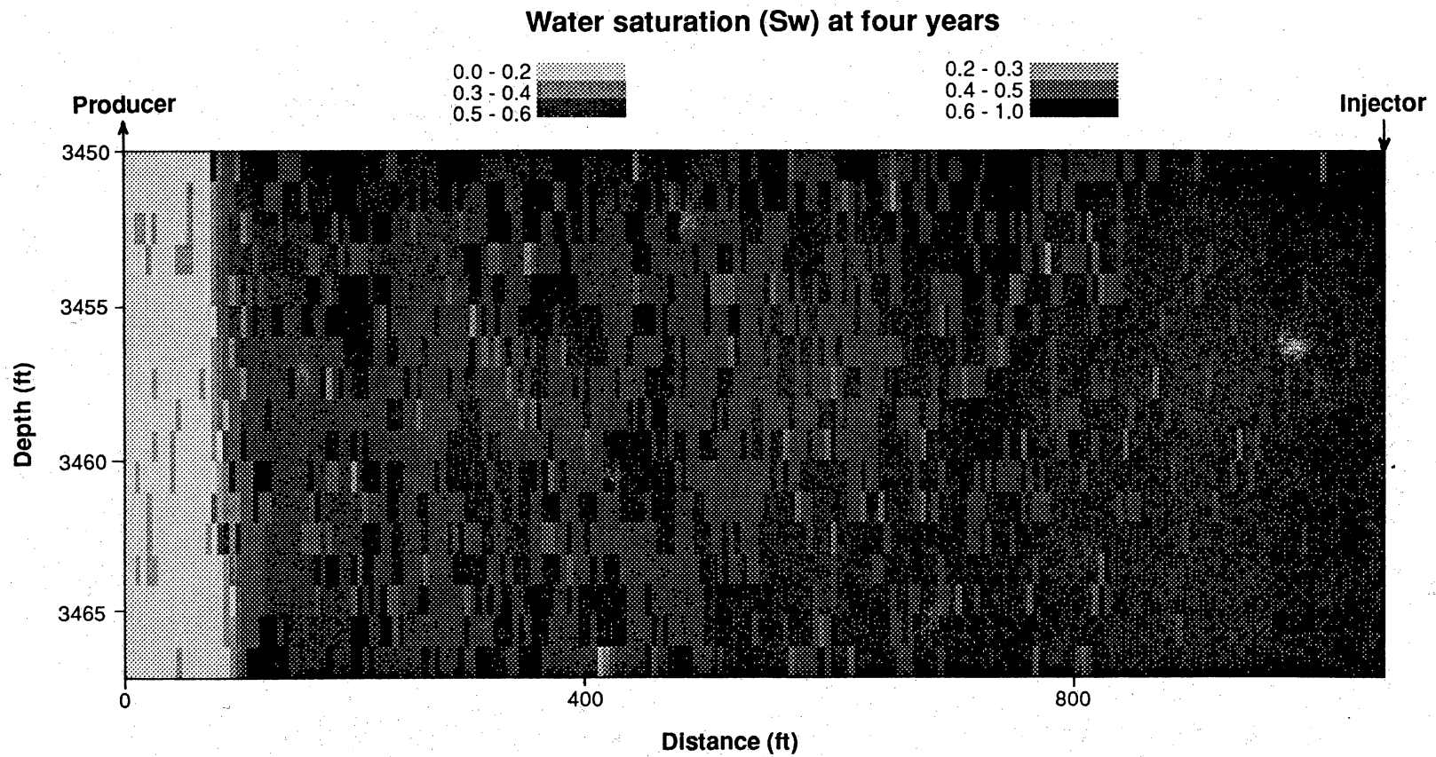
Figure 22. Computed water saturations for simulation 2 after injecting water for 4 yr, incorporating the permeability realization 7 (with relative-permeability curves and capillary-pressure curves dependent on porosity).
