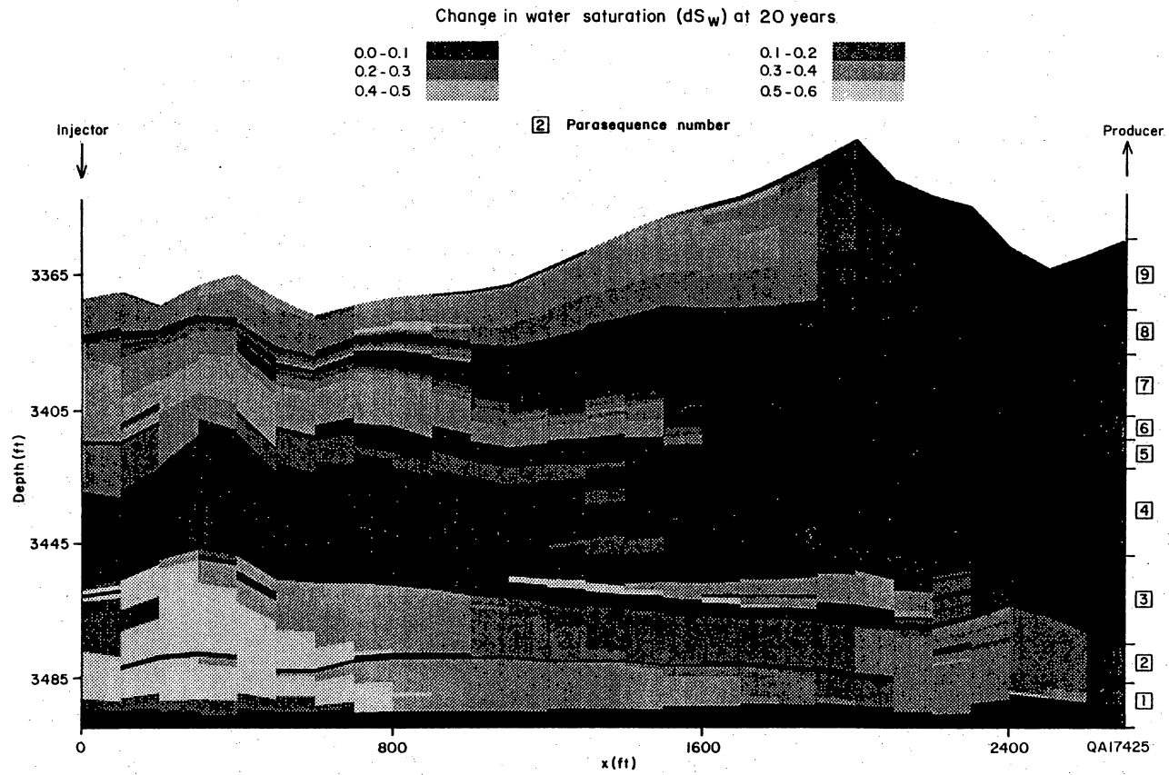
Figure 27. Computed changes in water saturation for simulation EC-A after waterflooding of (a) 20 yr, (b) 40 yr, (c) 60 yr.
