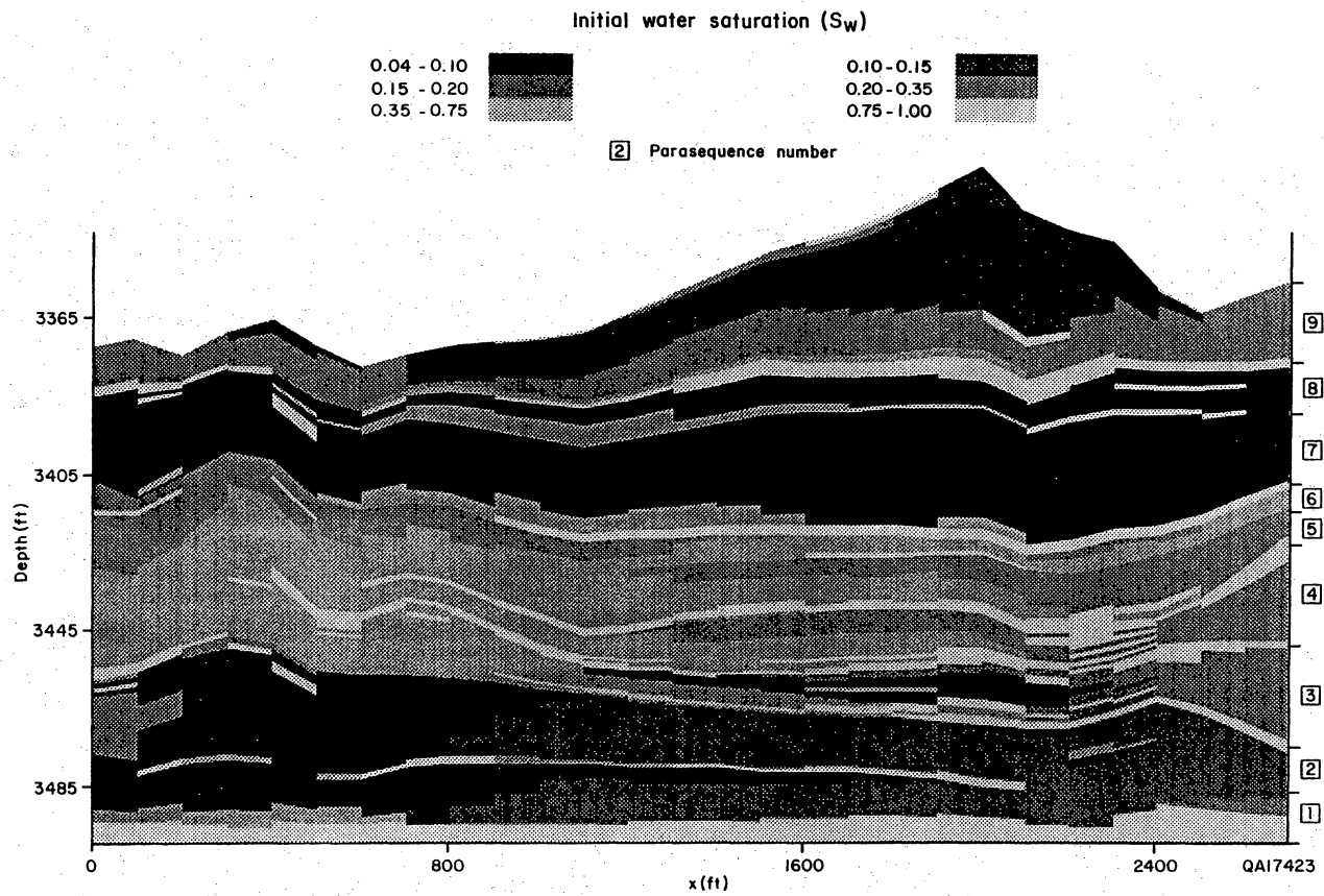
Figure 26. Initial water saturation of the flow units of the outcrop model.
