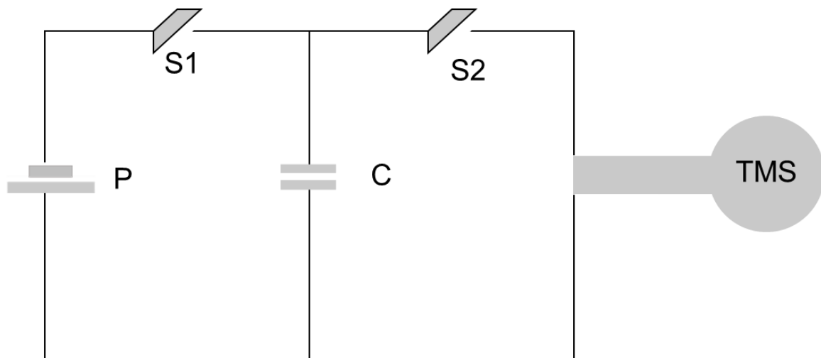
Figure 1.2. Schematic representation of a basic magnetic stimulator showing an electrical power source (P) that charges the capacitor (C) upon closure and reopening of the switch (S1). The capacitor (C) will discharge into the TMS coil (TMS) once the switch (S2) is closed.
