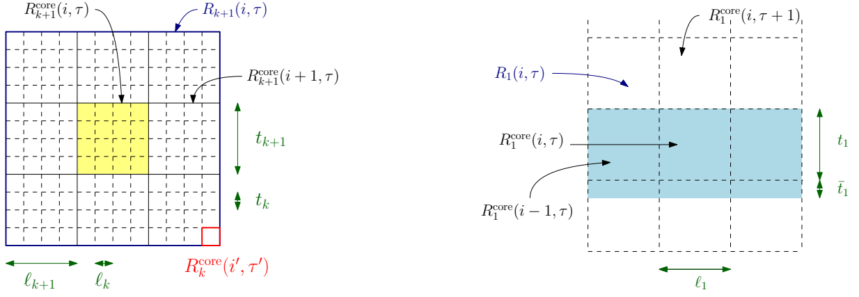
Figure 1: On the left a space-time box R_{k+1}(i, \tau) represented by a blue square, its core highlighted in yellow, its partition into cores of scale k + 1 represented by solid black lines, and its partition into cores of scale k in dashed lines. The horizontal axis represents space and the vertical axis represents time. On the right a space-time box of scale 1 (highlighted in blue), and space-time cores of level 1 in dashed lines.
