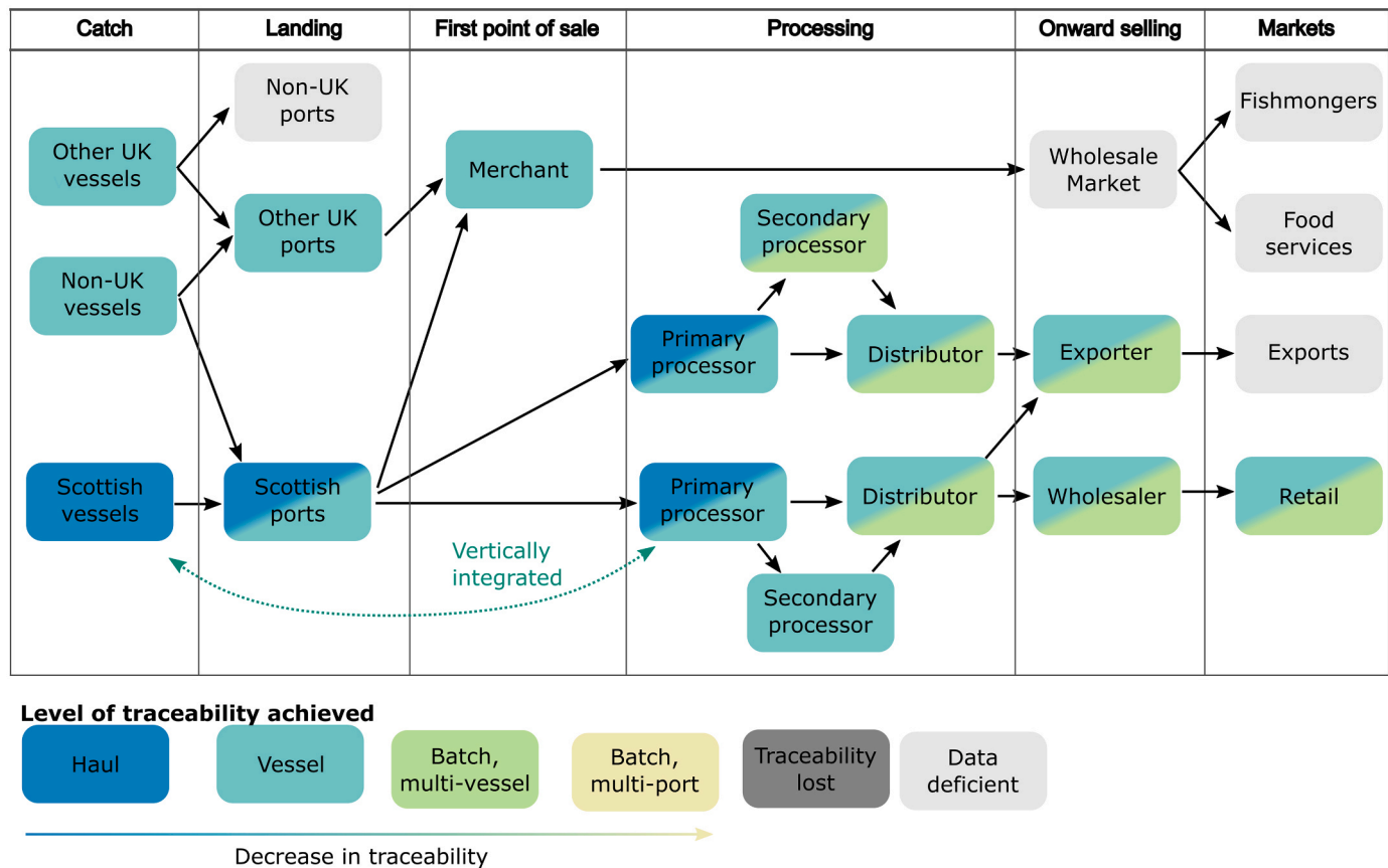
Fig. 2. North-East Atlantic (NEA) mackerel supply chain showing high level (haul and vessel) traceability through much of the chain because of vertical integration early in the chain and little mixing between network nodes.
