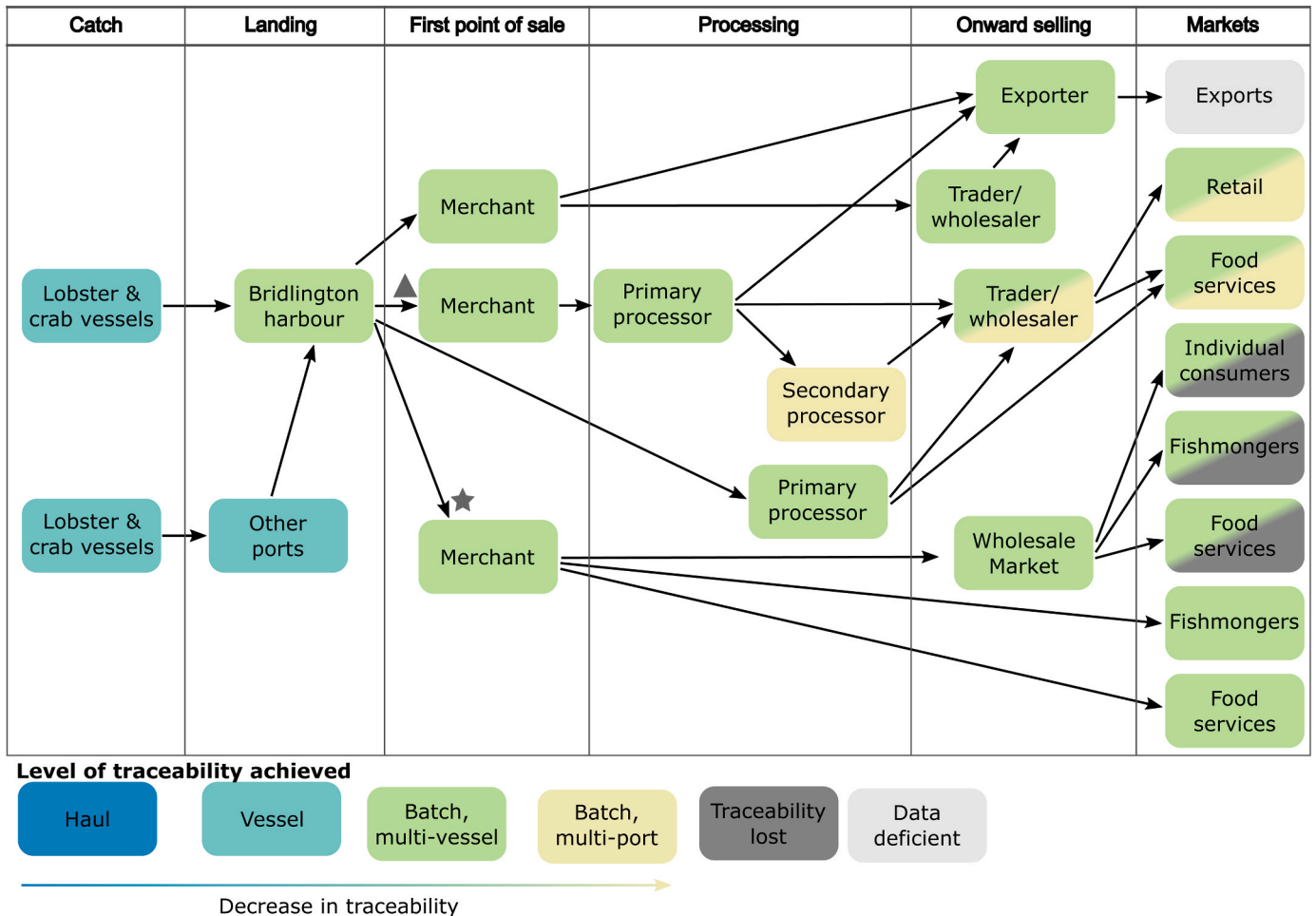
Fig. 3. Brown crab and European lobster supply chain showing the initial breakdown in traceability during post-mortem batch mixing of crab and live batch mixing of lobster at landing and first point of sale stages. Further loss of traceability can be seen to occur during processing. The grey triangle shows a link dominated by brown crab and the grey star shows a link dominated by European lobster.
