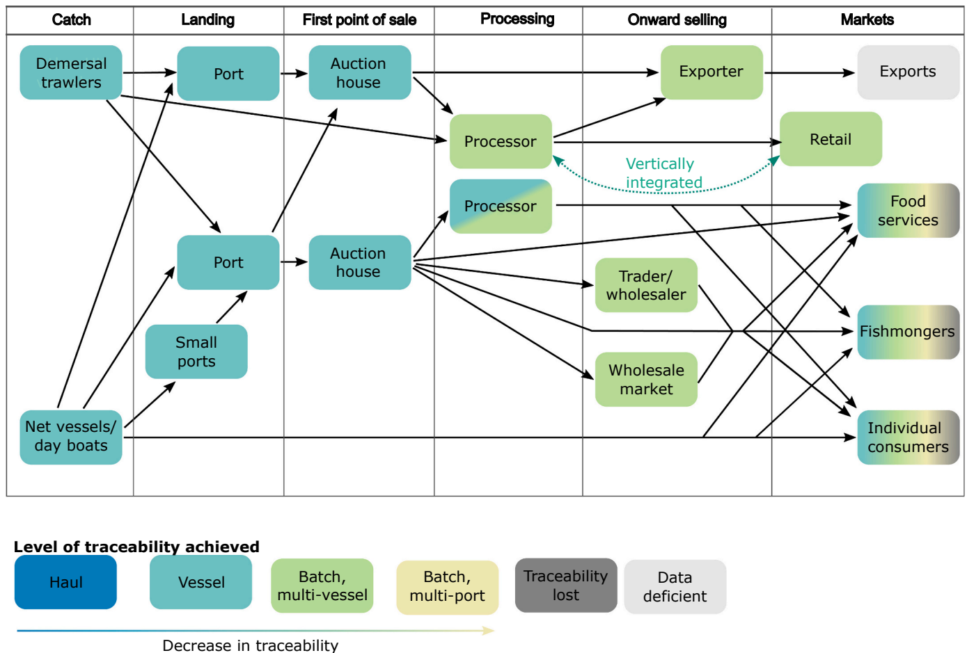
Fig. 1. Dover sole supply chain showing the first point of traceability loss during processing and then the further loss in traceability after substantial mixing from onward selling to final markets.
