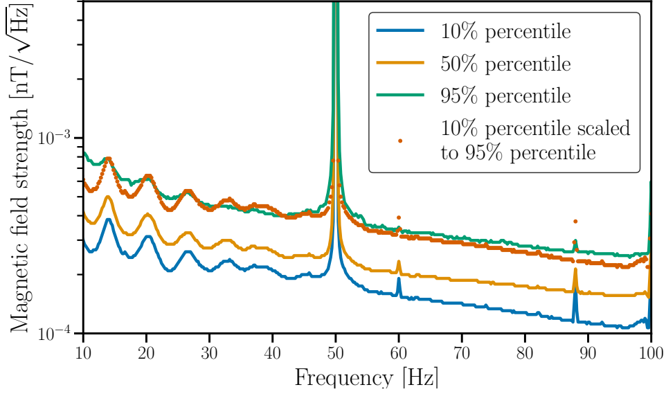
Figure 2.12: Sos Enattos magnetic ASD constructed using 48 days of data from Nov 14 2019 to Dec 31 2019. A one-directional magnetometer was employed to collect the data in the mine approximately 200 m below ground level. The line at 50 Hz is coming from the power mains.
