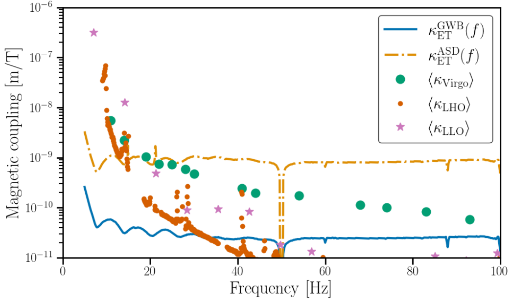
Figure 2.14: “ASD” and “GWB” magnetic coupling function upper limits for ET – X design sensitivity. Also included are the average of the measurements of the coupling functions at LIGO Hanford, LIGO Livingston and Virgo during the O3 run for comparison.
