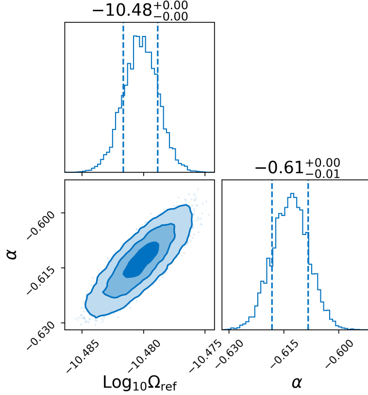
Figure D.1: Varying- \alpha PL fit to residual GWB spectrum of pop I+II+III from the StarTrack simulation. We see that the \alpha estimate is not 2/3 which would be expected for pop I/II.
