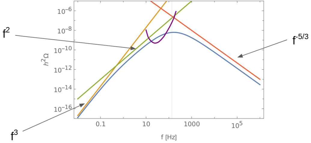
Figure 4.10: GWB spectrum from turbulence in the plasma during a FOPT as a function of frequency.
