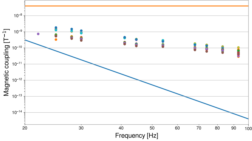
Figure 2.11: Measurements of the Virgo magnetic coupling function recorded throughout the O3 run. The two lines plotted show the lower and upper limit for the coupling function used as prior knowledge in our Bayesian analysis.
