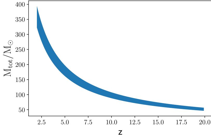
Figure D.3: M_{\text{tot}}^z = 1076 M_{\odot} constraint shown in the M_{\text{tot}}-z plane, including 10% error bars accounting for the uncertainty of the estimate of M_{\text{tot}}^z from f_{\text{peak}} .
