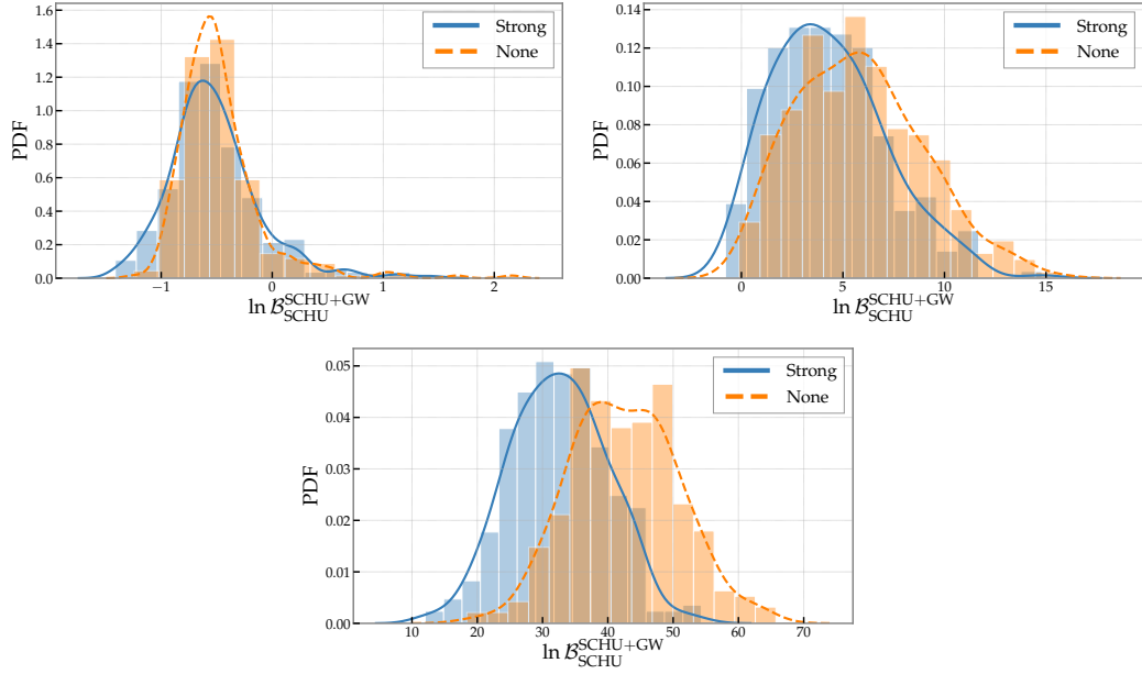
Figure 2.5: We show the distribution of \ln \mathcal{B}_{\text{SCHU}}^{\text{SCHU}+\text{GW}} for the strong (blue, solid) and none (orange, dashed) injection parameters, and \Omega_{2/3} = 0 (top left), \Omega_{2/3} = 3 \times 10^{-9} (top right) and \Omega_{2/3} = 10^{-8} (bottom). In the top left panel we see no evidence for a GW detection. In the top right and bottom panels we see evidence the presence of a GWB in both cases (although that evidence is marginal in the top right panel). The presence of correlated magnetic noise has clearly shifted the Bayes factor distributions downward.
