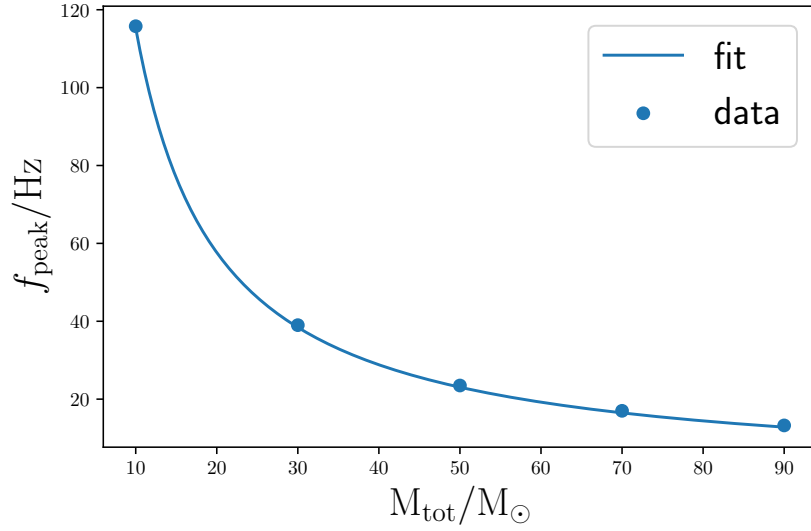
Figure D.2: StarTrack merger rate evolved, equal-mass binaries. We find a relationship between peak frequency and total intrinsic mass of the merger. This is a model-dependent statement.
