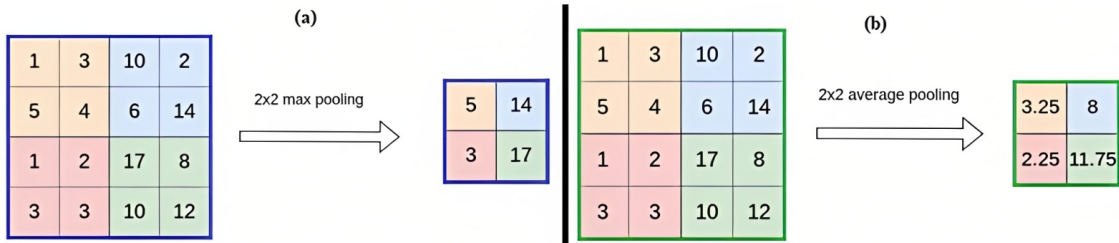
Fig. 3.8 Max and average pooling operations. Figure adapted from Vasilev et al. [90].
