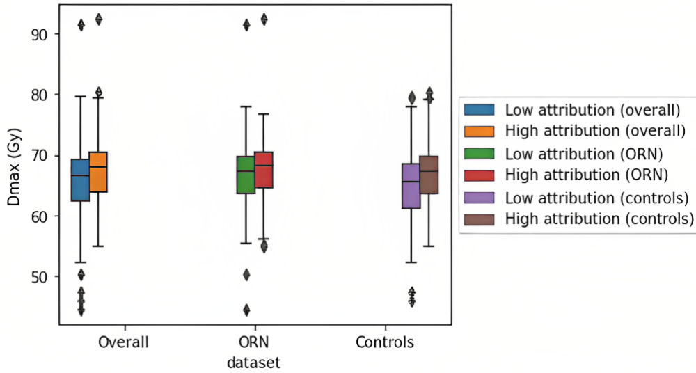
Fig. 8.8 Boxplots of the maximum radiation dose value in the dose distribution maps masked with low and high attribution levels for the entire cohort and the ORN and control groups separately. High attribution regions generally contain higher doses. The ORN group shows generally higher doses than the controls group but the difference in median D_{max} between high and low attribution masks is larger in the controls group.
