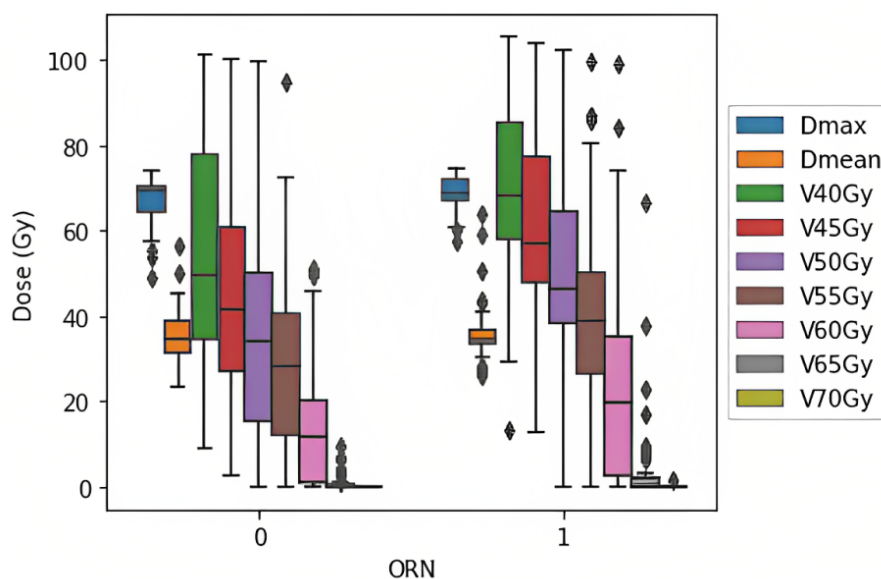
Fig. 5.1 Boxplots showing the distribution of the DVH-based variables used in this Chapter, where 0 and 1 in the x-axis correspond to the controls and cases, respectively.
