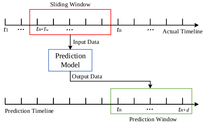
Fig. 2.10 Sliding window.
