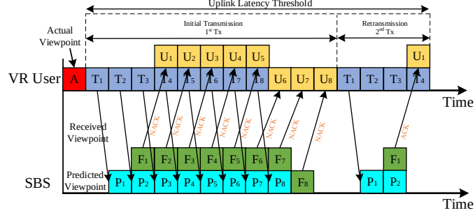
Fig. 2.9 Proactive retransmission scheme.
