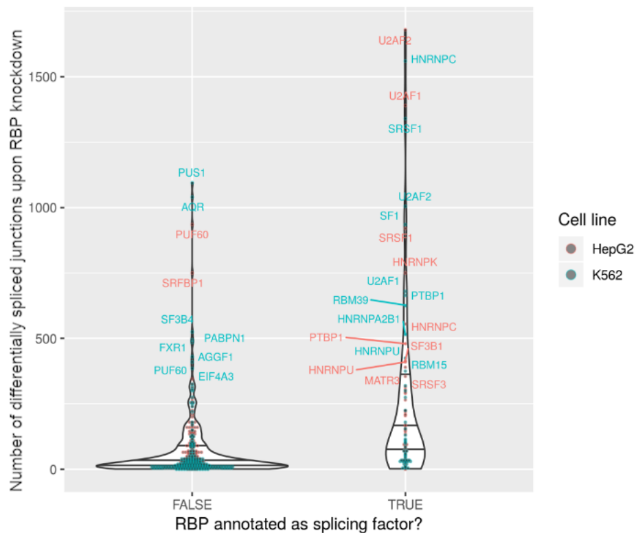
Figure 3-5. Effects of RNA-binding protein knockdowns on splicing in HepG2 and K562 cells. Knockdowns producing altered splicing of more than 300 splice junctions are labelled with the target RNA-binding protein.
