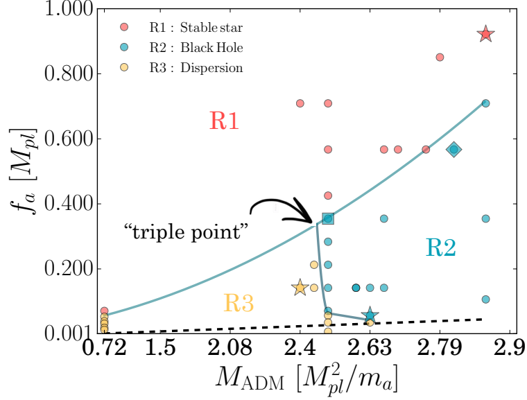
Figure 1.8: The “axion stability diagram” which shows 3 regions parametrised by the initial ADM mass of the star, M_{ADM} , and the axion decay constant f_a . These regions are: R1 - stable star, R2 - black hole collapse, and R3 - dispersion region. The dashed line indicates where the axion mass is negligible. Other symbols on the graph indicate [114] choose to explain these simulations in more depth. Image from [114].
