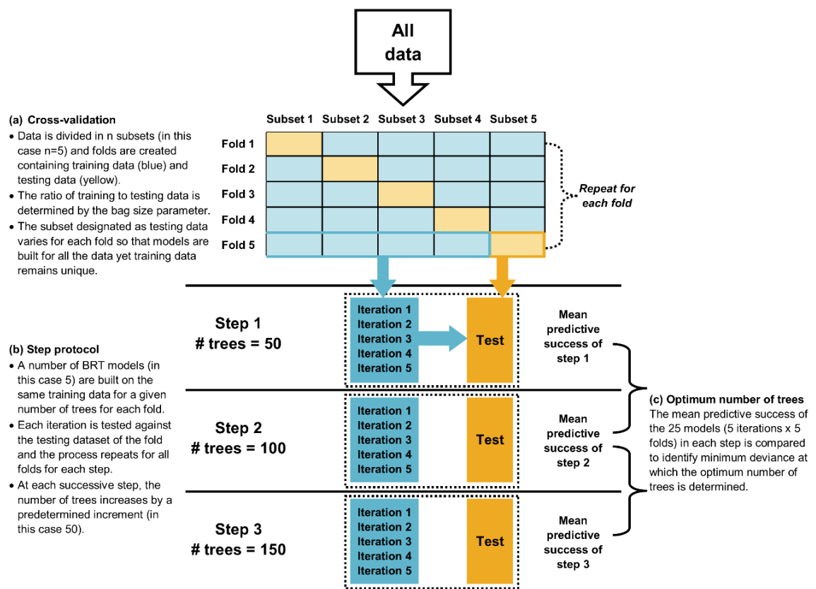
Figure 6.3. Schematic of Elith et al. 's (2008) cross-validation (CV) protocol to determine the optimum number of trees in three steps: (a) cross-validation; (b) step protocol; and (c) determining the optimum number of trees.
