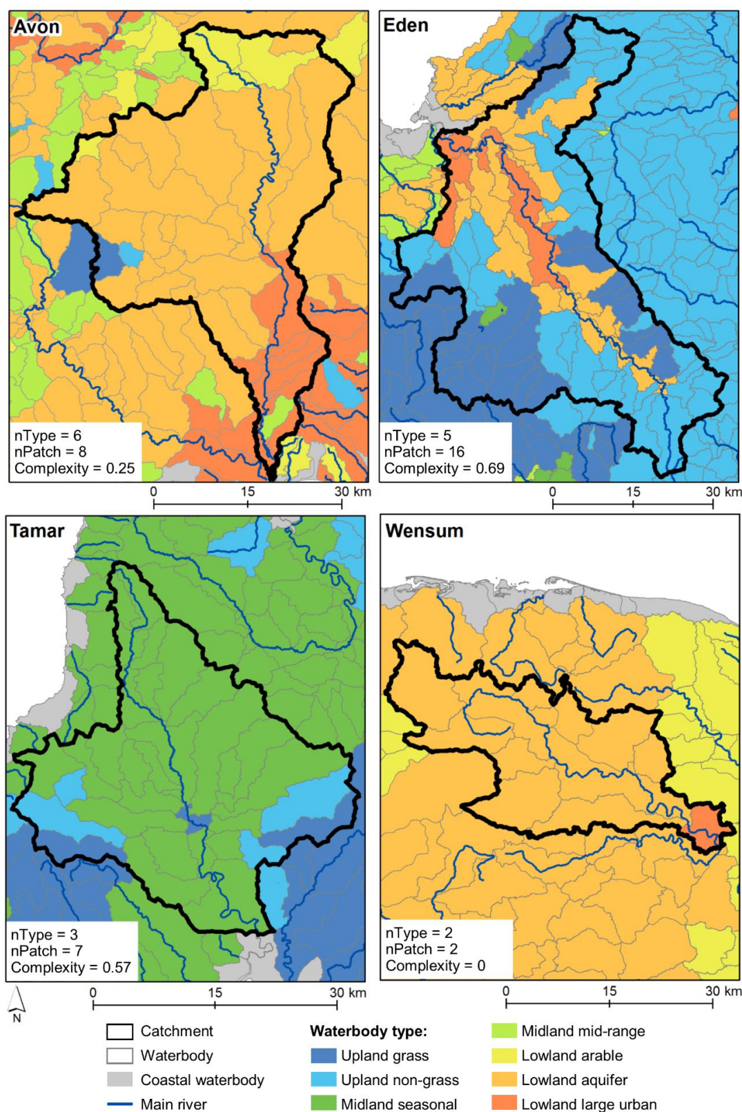
Figure 3.10. Waterbody types in each Demonstration Test Catchment. Number of waterbody types (nType), the number of patches (nPatch) and the complexity index for each catchment are in the corner of each pane.
