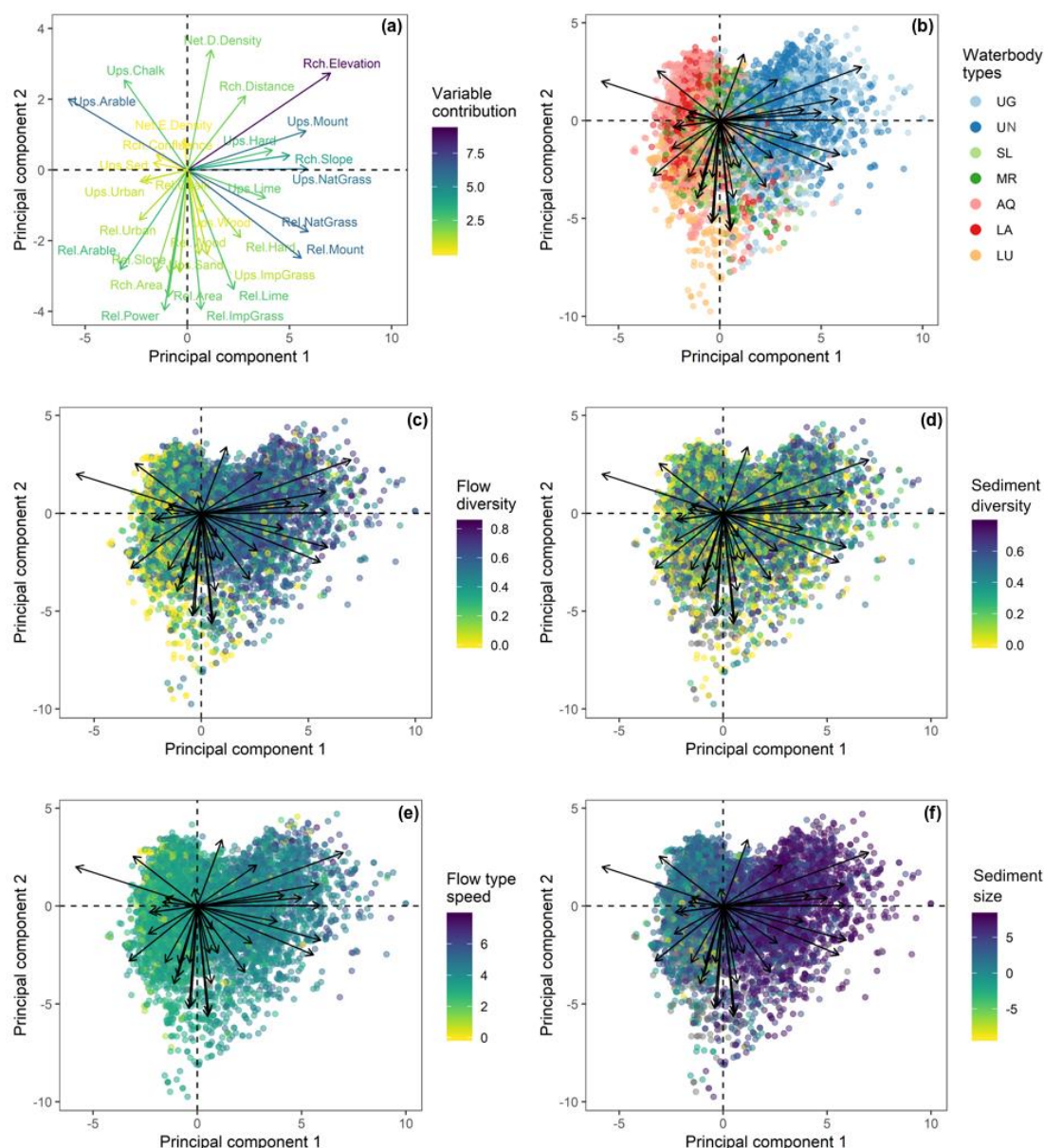
Figure 6.4. PCA results on all control variables: (a) PCA loading plot of 34 variables, distribution of RHS sites on PCs 1 and 2 coloured by (b) waterbody type and (c-f) habitat indices.
