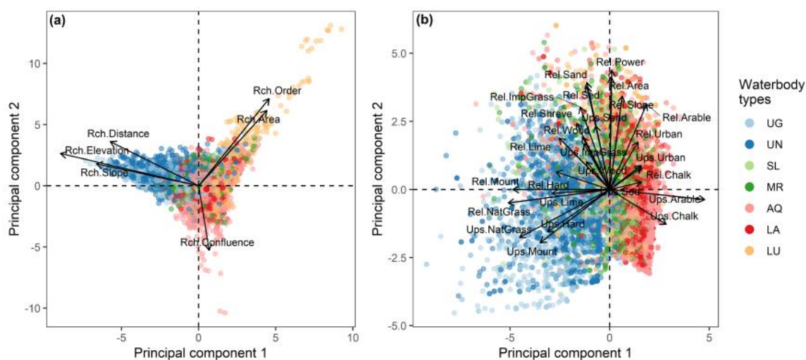
Figure 6.5. Biplots of PCA results on (a) reach and (b) upstream and confluence control variables. Colours indicate waterbody types (see Table 6.2 for abbreviations).
