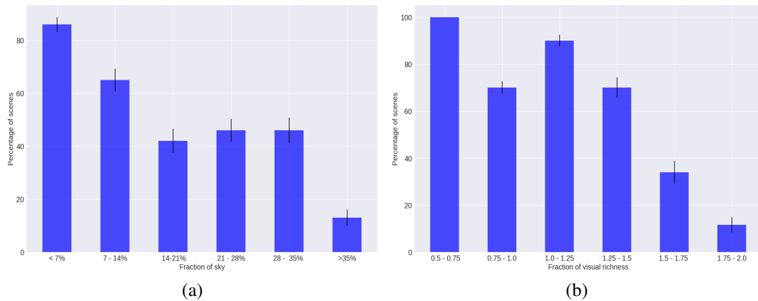
Fig. 6.5 The percentage of beautified scenes (y-axis): (a) having an increasing presence of sky (on the x -axis); and (b) having an increasing level of visual richness (on the x -axis). The error bars represent standard errors obtained by random re-sampling of the data for 500 iterations.
