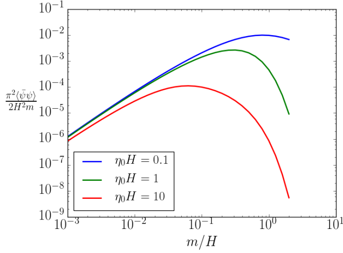
Figure 3.2: Plot of the product \frac{\langle \bar{\psi} \psi \rangle \pi^2}{2H^2 m} as a function of the mass m/H . The speed of the transition ( \eta_0 ) from de-Sitter to Minkowski only affects the production of heavy fermions. Production of light fermions can be seen to be unchanged regardless of the value of \eta_0 .
