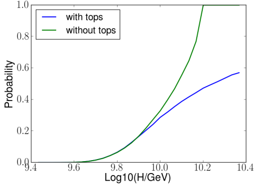
Figure 3.6: Probability of going over the barrier after 60 e -folds for a renormalisation scale \mu^2 = h^2 + H^2 .
