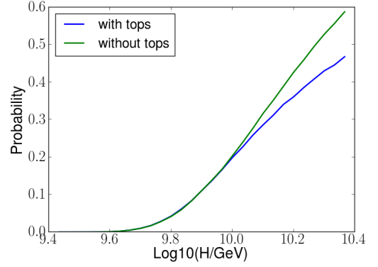
Figure 3.7: Probability of going over the barrier after 60 e -folds for a renormalisation scale \mu = h .
