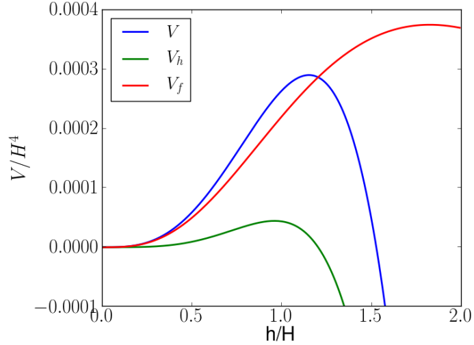
Figure 3.5: Plot of V/H^4 as a function of h/H for H = 10^{10} \text{ GeV} . With the additional effect of the fermionic contribution to the potential V_f , the total potential V = V_h + V_f has a barrier which is five times higher.
