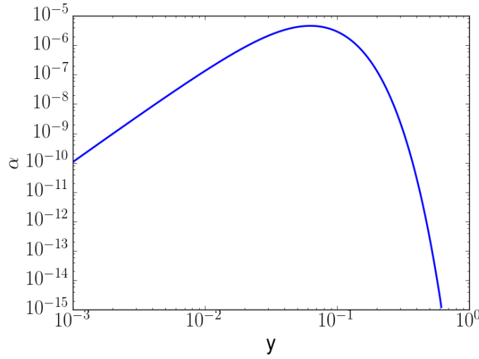
Figure 3.8: The effect of the fermions on the stability of the EW vacuum, parametrized by \alpha as a function of the Yukawa coupling y(\mu = h_{\text{max}}) . It peaks at y = 0.062 , close to the value for the bottom quarks. Larger Yukawa couplings have a smaller effect on the stability of the EW vacuum.
