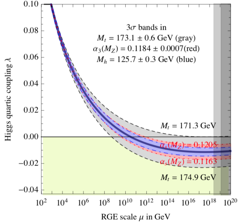
Figure 1.4: Running of the Higgs self-interaction coupling from [34]. The instability scale is at about 10^{10} GeV for SM central values. It shows how much depends on the mass of the top quark, the Higgs mass and \alpha_s .
