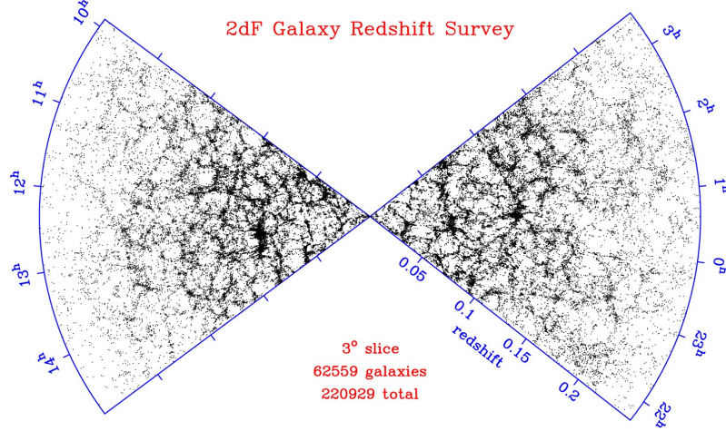
Figure 1.1: Each dot is a galaxy with the Earth in the center of the map. It shows the spatial distribution of galaxies as a function of redshift from the 2dF Galaxy Redshift Survey [12]. On small scales the distribution is inhomogeneous but becomes more homogeneous on large scales.
