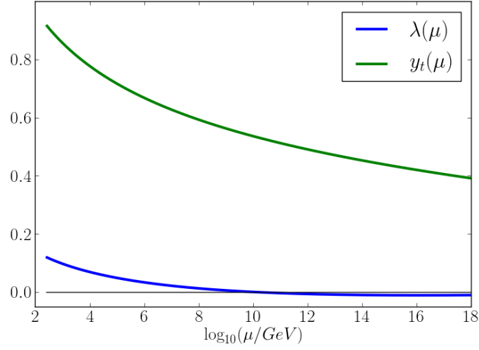
Figure 3.1: Running of the Higgs self-interaction and the top yukawa coupling as a function of the energy scale \mu up to 3-loops. The instability scale is at 10^{10} GeV, when \lambda < 0 and y_t = 0.5 . To make this plot we have used m_t = 173 GeV, \alpha_s = 0.1181 , m_h = 125.18 GeV.
