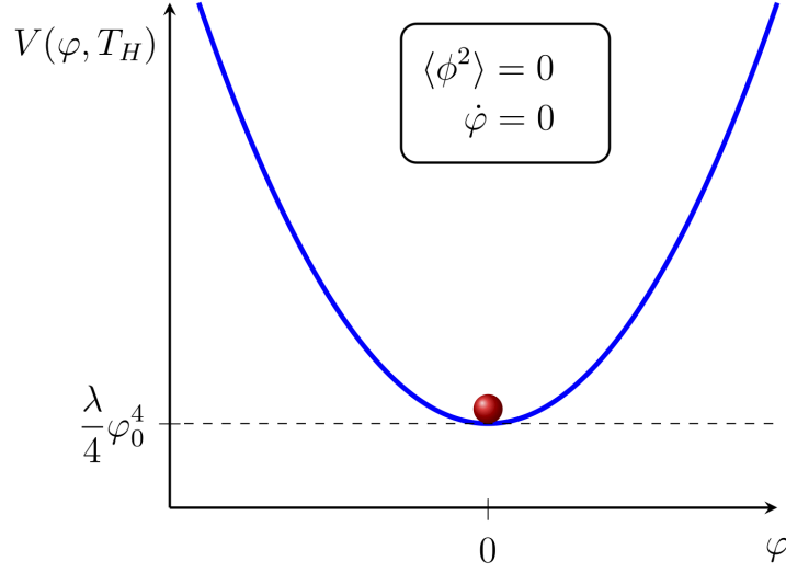
Figure 2.2: In the unbroken phase the field is at rest at \varphi = 0 with practically no quantum fluctuations, \langle \phi^2 \rangle \sim 0 . The suppression of the quantum fluctuations is caused by the large effective mass making the field heavy with respect to the background curvature.
