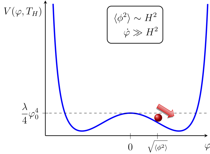
Figure 2.4: The onset of classical rolling occurs when the steepness of the potential has increased enough. The initial value for the field is determined by the preceding random-walking epoch when |m^2| \lesssim H^2 .
