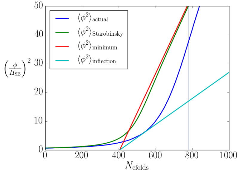
Figure 2.5: Field dynamics with \lambda = 10^{-3} , N = 10^{5.5} , \varphi_0 = 10^{-1.27} M_P and g = 0.7 . We plot the evolution of the field expectation vs. the Starobinsky estimate in units of H_{SB}^2 to show that they are different. We also show the time evolution of the minimum and the inflection point (which the field must remain beyond in order to obtain a red spectrum). N_e = 780 is the epoch when the spectrum of perturbations and the tilt match the observed values by Planck.
