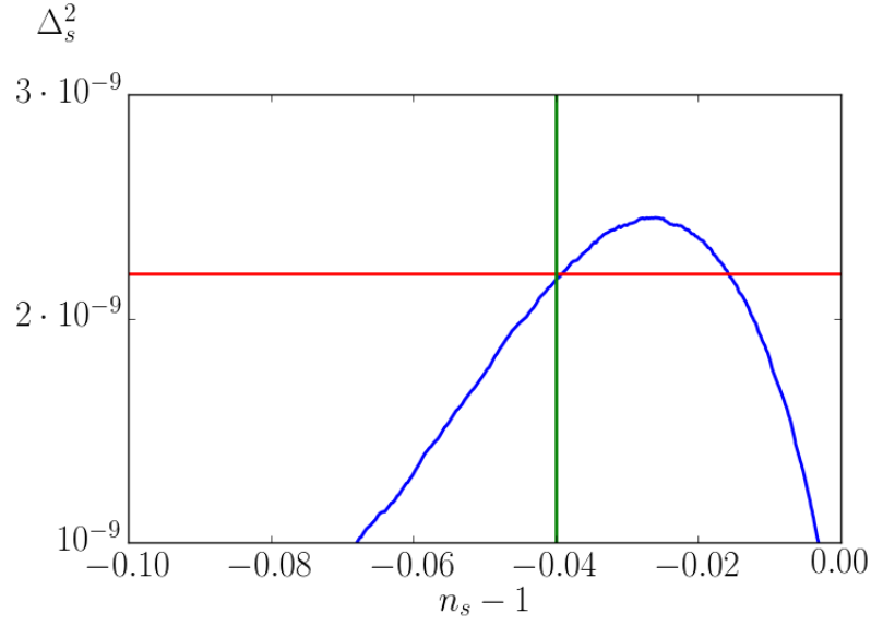
Figure 2.6: Amplitude of the spectrum of perturbations versus the tilt with \lambda = 10^{-3} , N = 10^{5.5} , \varphi_0 = 10^{-1.27} M_{\text{P}} and g = 0.7 . The blue line is the simulation (average over 10^4 realisations) and the green and red lines are the cosmologically observed value of the spectrum and amplitude of perturbations respectively.
