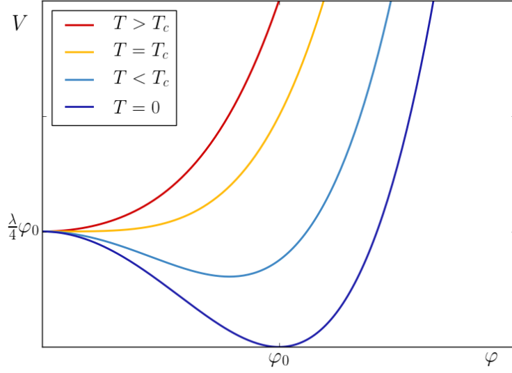
Figure 2.1: Initially for a high temperature the field is located at the origin in the symmetric phase. As the temperature drops a new minimum is generated and the symmetry is broken.
