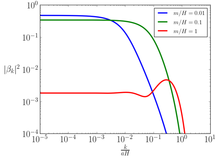
Figure 3.3: Plot of |\beta_k|^2 as a function of k/aH for different masses. If the fermions are light, the spectrum can be approximated as 1/2 up to k/a = m ; for the heavy fermions the spectrum is suppressed as 1/(1 + e^{2\pi m/H}) .
