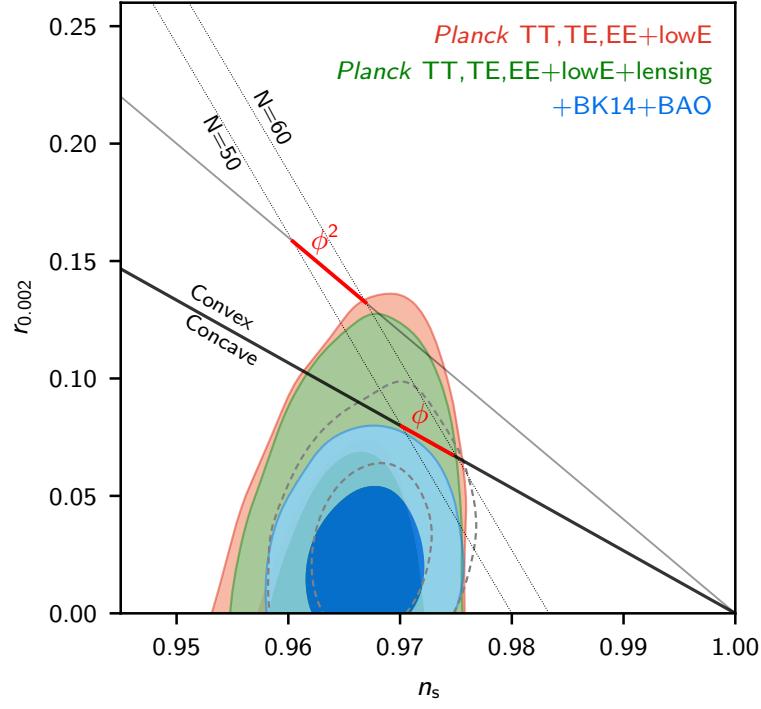
Figure 1.3: Plot by Planck [23] showing the current bound on the tensor to scalar ratio for a pivot scale of k^* = 0.002 \text{Mpc}^{-1} , r < 0.1 and the spectral tilt n_s - 1 = 0.97 . Current measurements disfavour a monomial inflaton potential with exponent larger than one for a duration in between 50 to 60 e-folds. It also favours a concave inflaton potential.
