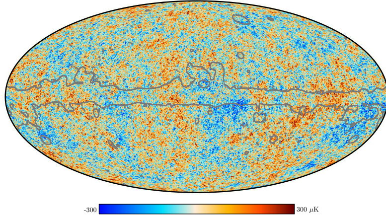
Figure 1.2: The temperature of the CMB is on average T_{CMB} = 2.7K . In this map by Planck [1] we can see the anisotropies on top of T_{CMB} . The scale of this inhomogeneities is \mathcal{O}(100)\mu K , five orders of magnitude smaller than T_{CMB} , from which we can assume that the universe is homogeneous on large scales.
