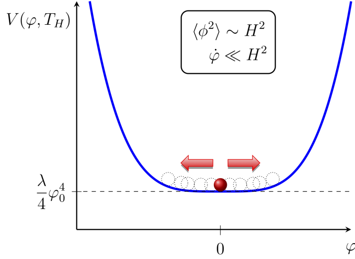
Figure 2.3: Close to symmetry breaking the classical (mean) field \varphi is almost stationary, but the quantum fluctuations \langle \phi^2 \rangle very large since the field is effectively light |m^2| \lesssim H^2 .
