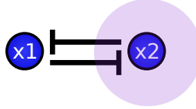
Figure 4.1: Network illustrating the bistable switch system defined using cross-repressive Hill functions, see (4.47). Blunt arrows indicate repression, purple shading indicates the species placed in the bulk.
