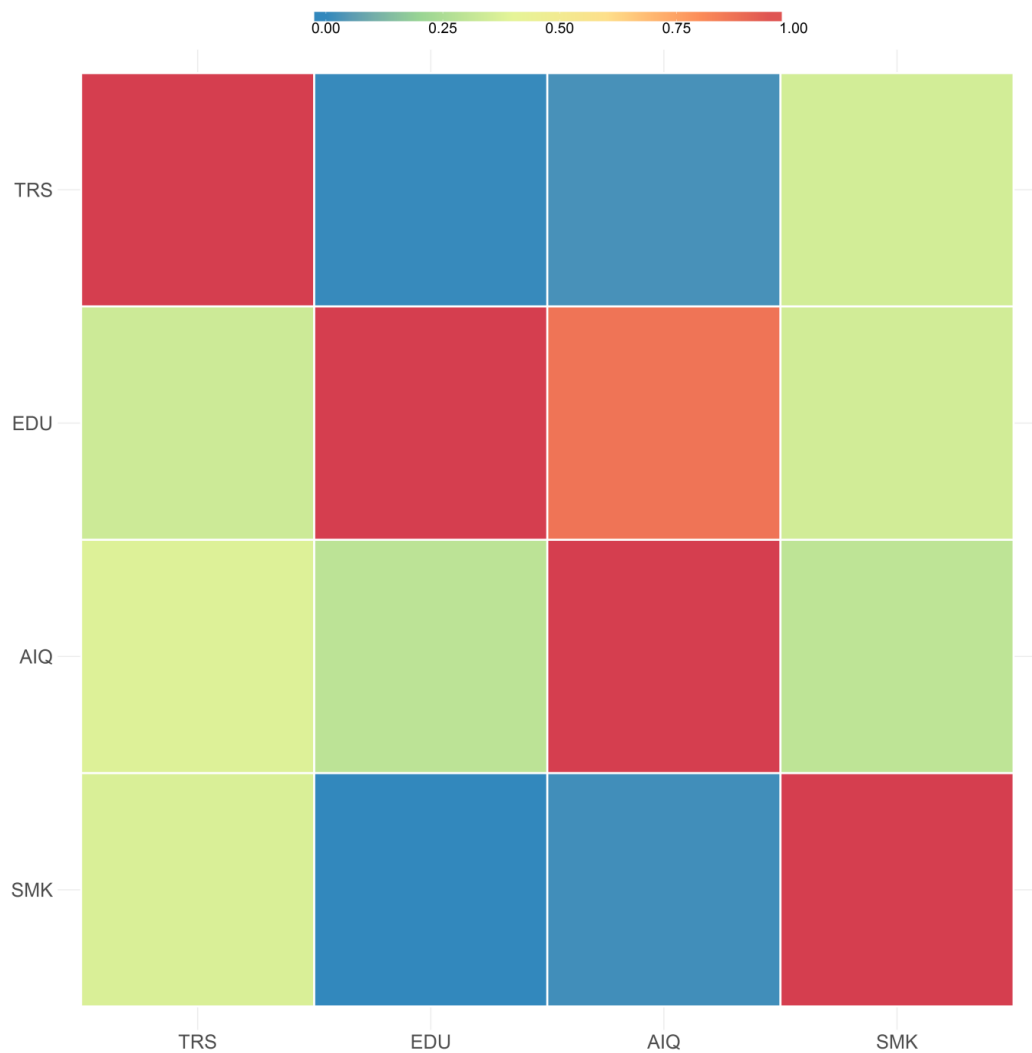
Figure 13. Pairwise matrix of GWAS-pw maximum a posteriori (MAP) estimates of shared variants between traits (TRS = Treatment-resistant schizophrenia; EDU
