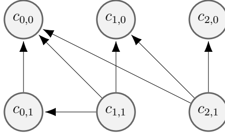
FIGURE 7.5.4. The dependency graph of a character \chi with tame signature (a_0, 1, 1) for any 2 < a_0 < p assuming e = 2 .
