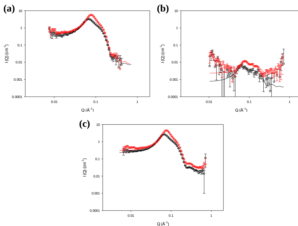
Figure 4. 10 SANS profiles and model fits (solid line) for 3 wt % (black) and 5 wt % (red) d_{25} LDS in H_2O (a), d_{25} LDS in D_2O (b) and h_{25} LDS in D_2O (c).
