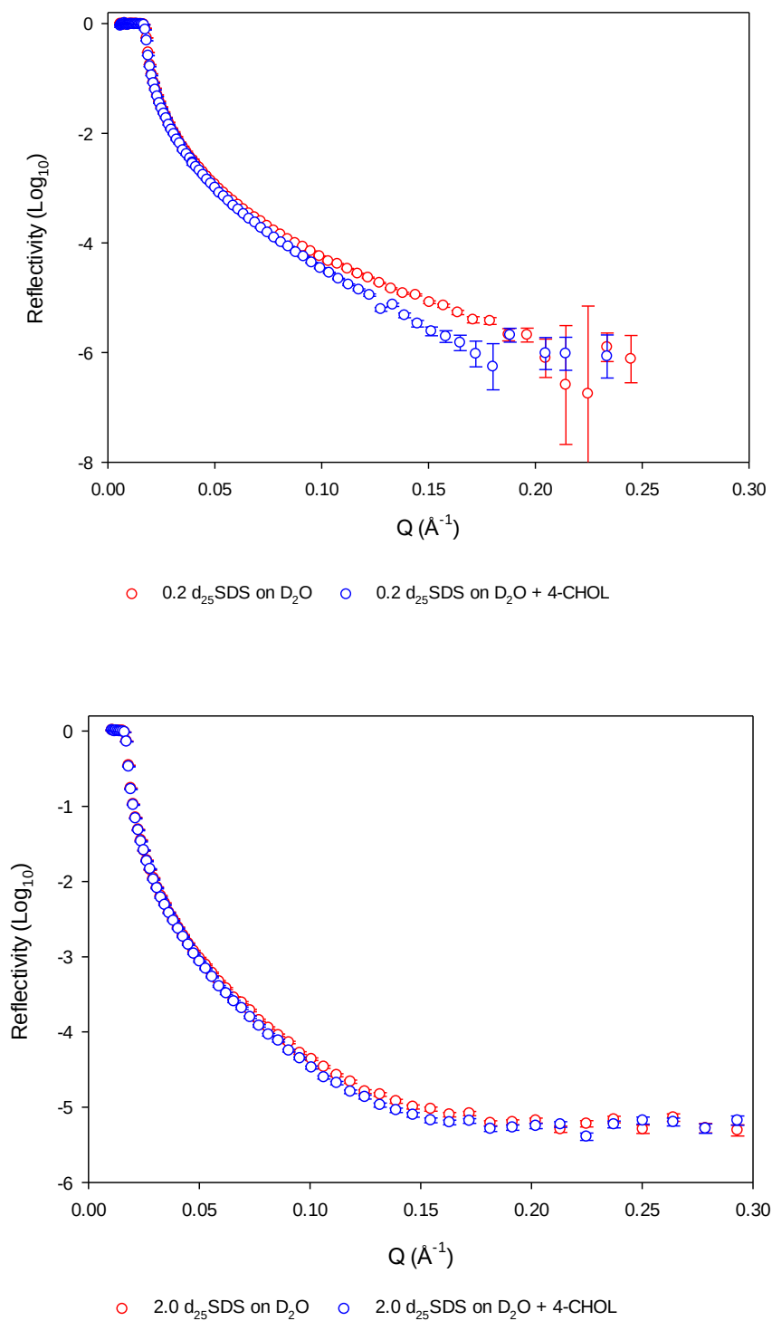
Figure 3. 8 NR profiles for d_{25} SDS monolayers formed in the presence of 4-cholesten-3-one on sub-phases of ACMW (previous page) and D_2O (this page), with SDS concentrations below the CMC (upper panels) and above the CMC (lower panels).
