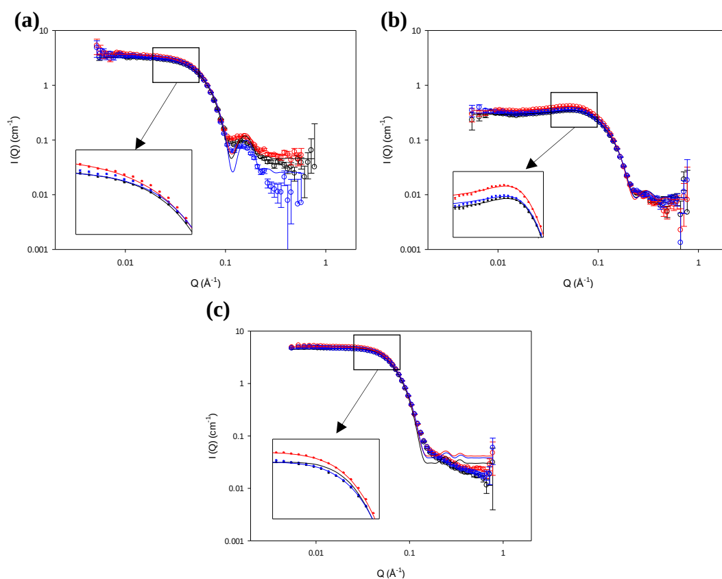
Figure 4. 27 SANS profiles for d-Tween 20 in H 2 O (a), d-Tween 20 in D 2 O (b) and h-Tween 20 (c) in D 2 O micelles alone (black), micelles in the presence of saturation amounts of 4-CHOL (red) and ADRENO (blue) at 3.5 wt %.
