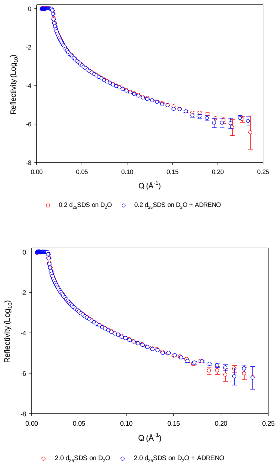
Figure 3. 9 NR profiles for d 25 SDS monolayers formed in the presence of adrenosterone on sub-phases of ACMW (previous page) and D 2 O (this page), with SDS concentrations below the CMC (upper panels) and above the CMC (lower panels).
