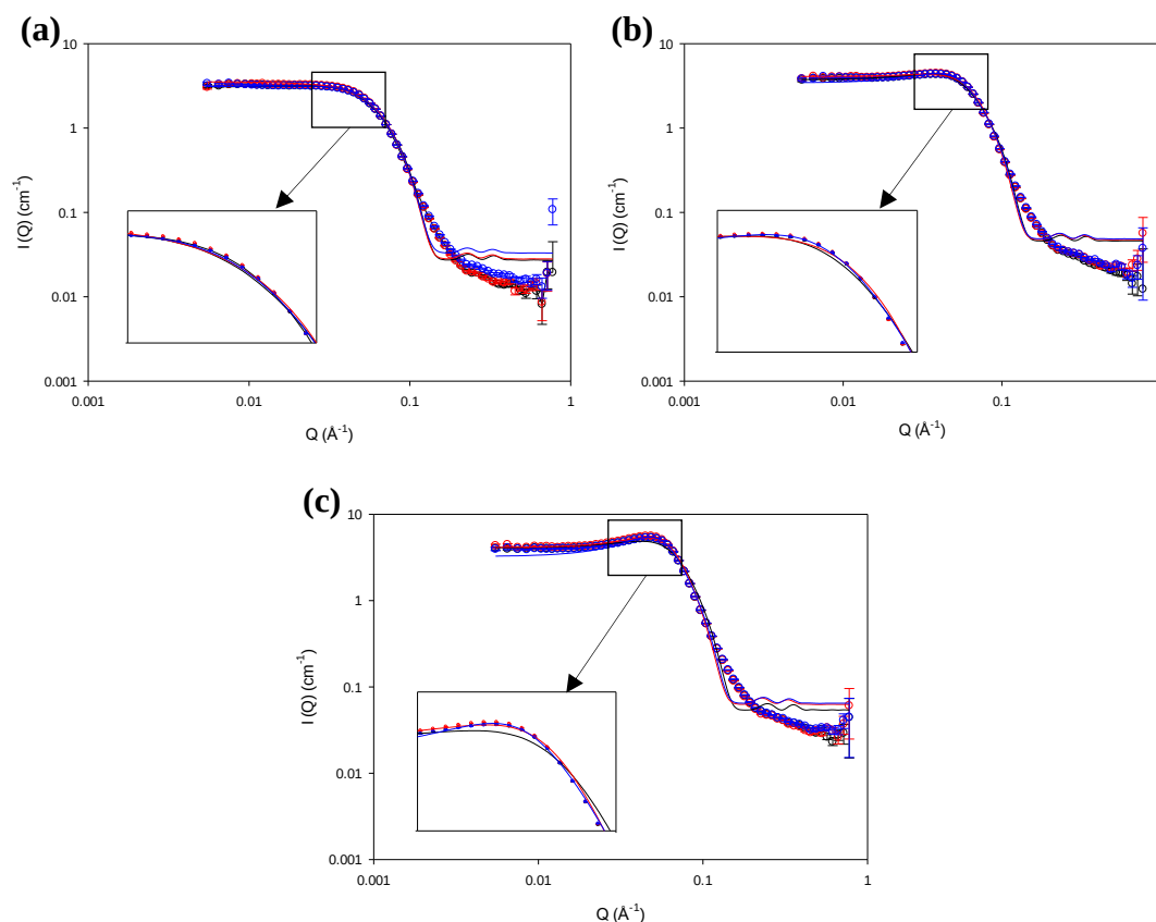
Figure 4. 29 SANS profiles and model fits (solid line) for 2 wt% (a), 3.5 wt% (b) and 5 wt% (c) of h_{25} Brij in D_2O in the absence (black) and in the presence of 4-CHOL (red) and ADRENO (blue).
