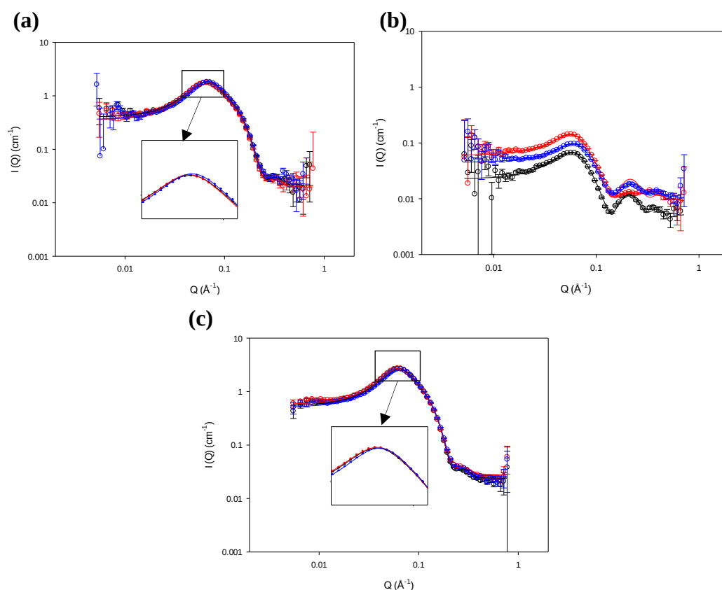
Figure 4. 5 SANS profiles and model fits (solid line) for d_{25} DTAB in \text{H}_2\text{O} (a), d_{25} DTAB in \text{D}_2\text{O} (b) and h_{25} DTAB (c) in \text{D}_2\text{O} micelles alone (black), micelles in the presence of saturation amounts of 4-CHOL (red) and ADRENO (blue) at 3 wt %
