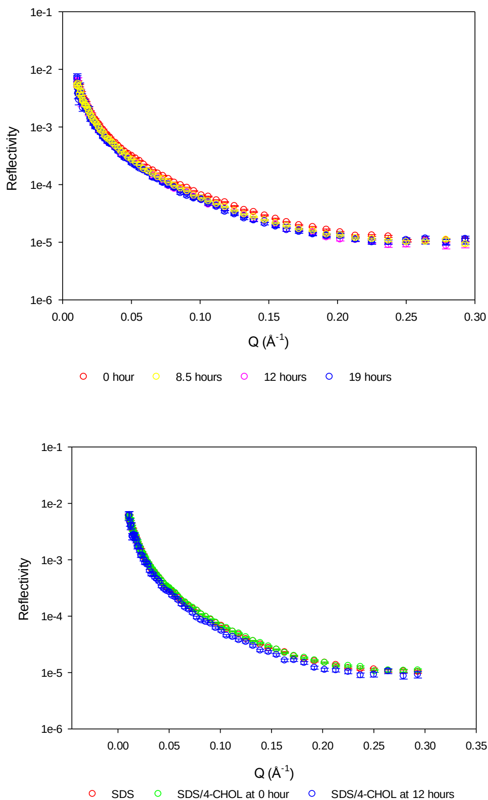
Figure 3. 14 NR profiles of d 25 SDS monolayer in ACMW in the presence of 4-cholesten-3-one at 2.0 x CMC
