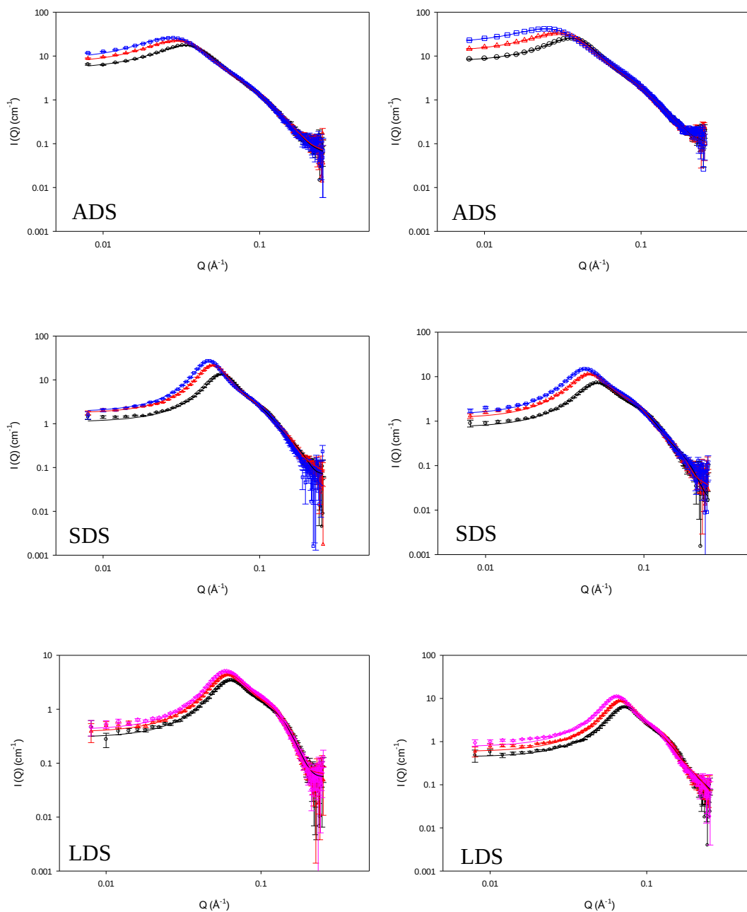
Figure 4. 30 SANS profiles and model fits (solid line) of dodecyl sulfate micelles in the presence of 4-CHOL at surfactant concentration 3 wt% (left column) and 5 wt% (right column) ○: 6 hours, △: 1 day, ◇: 5 days, □: 7 days
