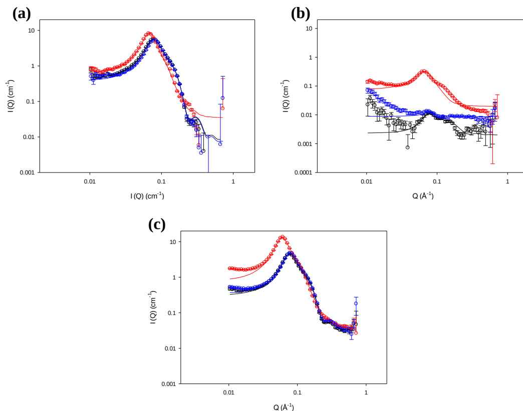
Figure 4. 12 SANS profiles and model fits (solid line) for d_{25} LDS in H_2O (a), d_{25} LDS in D_2O (b) and h_{25} LDS (c) in D_2O micelles alone (black), micelles in the presence of saturation amounts of 4-CHOL (red) and ADRENO (blue) at 5 wt %
