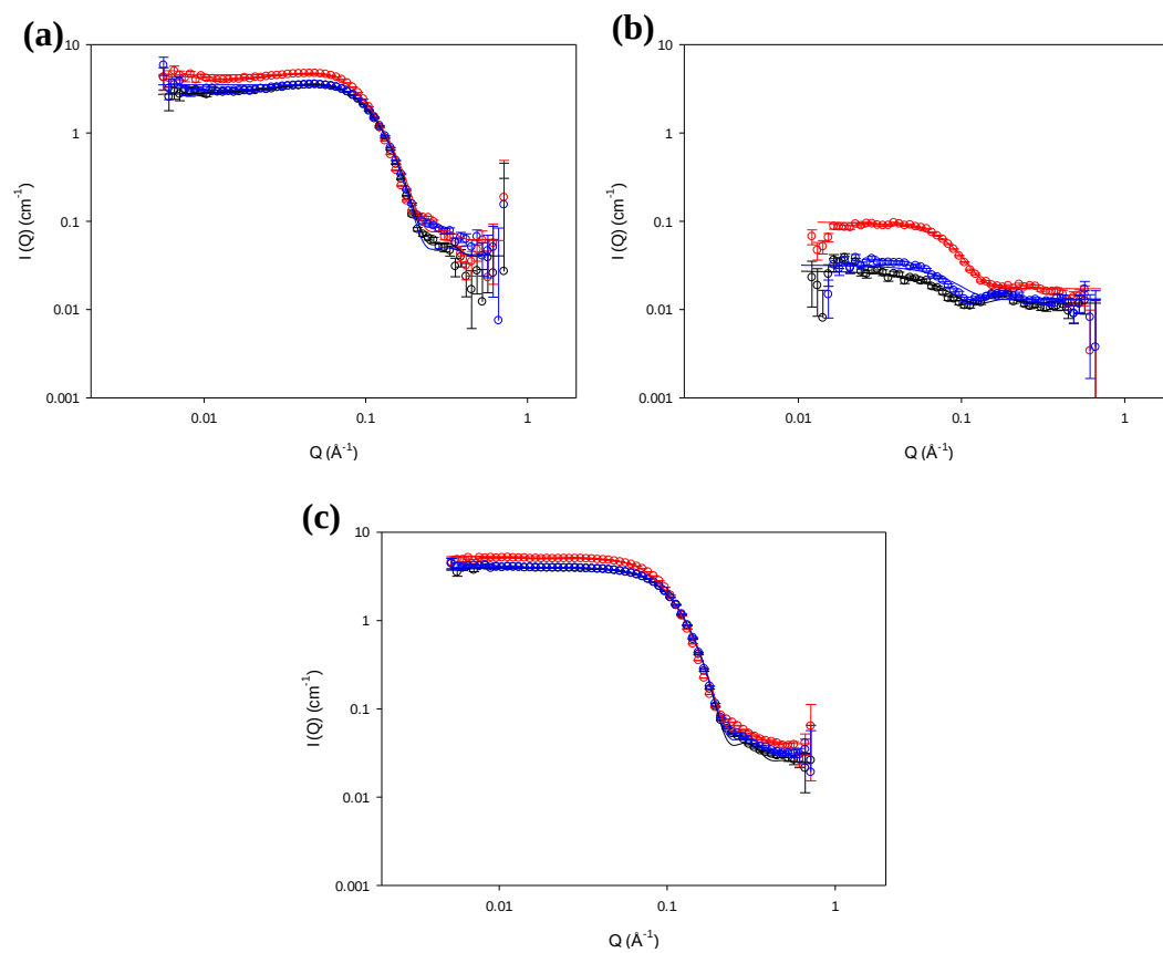
Figure 4. 21 SANS profiles and model fits (solid line) for d_{25} DDAO in \text{H}_2\text{O} (a), d_{25} DDAO in \text{D}_2\text{O} (b) and h_{25} DDAO in \text{D}_2\text{O} (c) micelles alone (black), micelles in the presence of saturation amounts of 4-CHOL (red) and ADRENO (blue) at 3.5 wt %.
