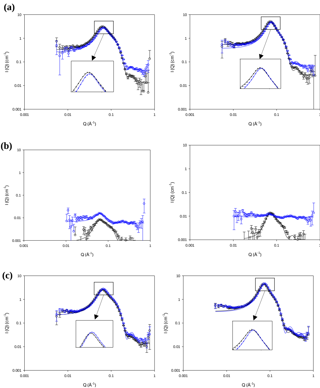
Figure 4. 9 SANS profiles model fits (solid line) for 3 wt % (left column) and 5 wt % (right column) d_{25} SDS in H_2O (a), d_{25} SDS in D_2O (b) and h_{25} SDS (c) in D_2O in the presence (blue) or absence (black) of ADRENO.
