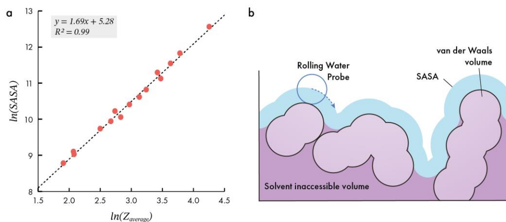
Figure 1.3. Relationship between charge from native MS and SASA. (a) Empirical relationship between the average observed charge state Z_{average} and SASA. Adapted from Hall & Robinson, 2012 13 . (b) SASA is defined as the surface area accessible by a water molecule (modelled by a spherical probe of radius 1.4 Å).
