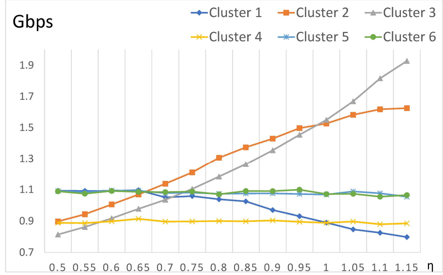
Figure 4.13: Channel Capacity of Each Mobile Patient When \eta is Changing.
