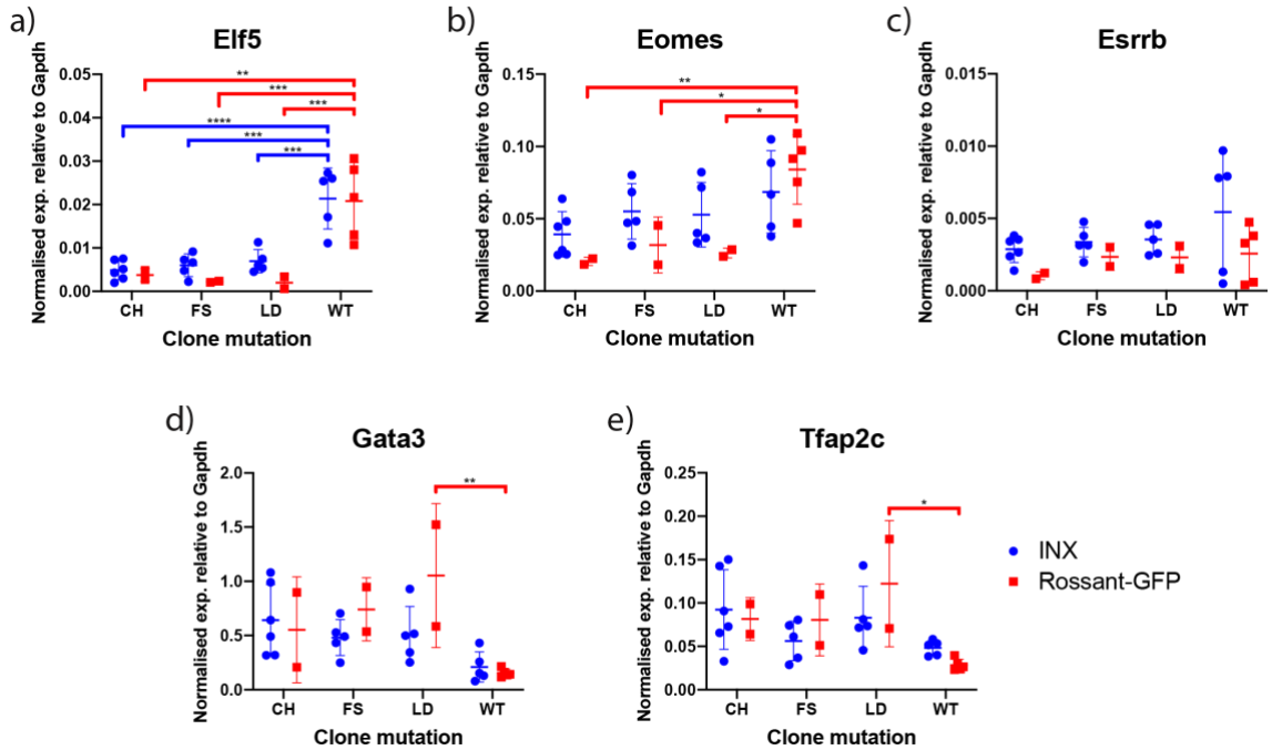
Figure 6.9: Trophoblast stem cell marker gene expression in Cdx2 -mutants. qRT-PCR analysis for TSC marker genes in compound heterozygous (CH), frameshift (FS) and large deletion (LD) Cdx2 -mutant clones and 5 wild-type (WT) control clones, outlined in Table 6.2. Each data point represents a single clone. Gene expression was normalised to Gapdh . Significance determined by two-way ANOVA test: * p ≤ 0.0332, ** p ≤ 0.0021, *** p ≤ 0.0002, **** p ≤ 0.0001. Error bars show SD.
