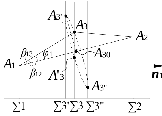
Figure 4-6 Location condition of constraint plane \Sigma 3
