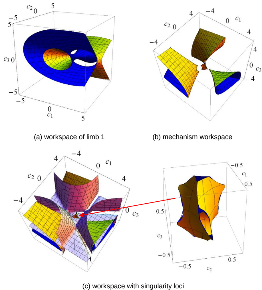
Figure 6-6 Workspace boundaries ( \alpha'_a=\pi/6 )
