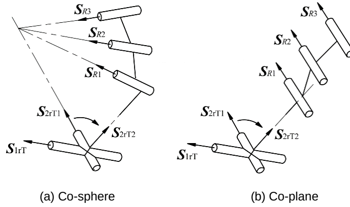
Figure 3-6 Co-spherical and co-planar order-change of the reconfigurable-limb twist system
