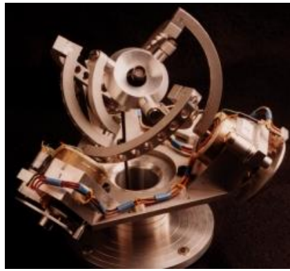
(a) The Agile eye [54]
