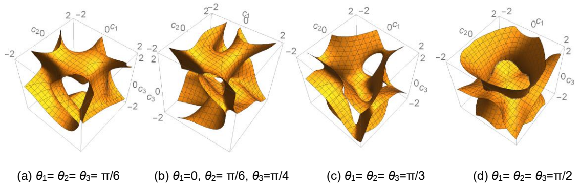
Figure 6-20 Singularity loci of topologies with 3R motion
