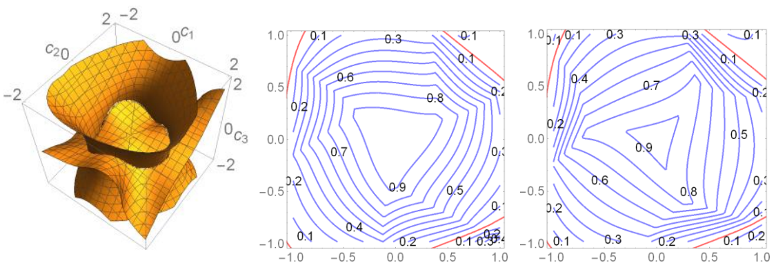
(d) \theta_1 = \theta_2 = \theta_3 = \pi/2 with 3R motion (left: singularity loci, middle: OTI at c_3 = 0.5 , right: CTI at c_3 = 0.5 )
