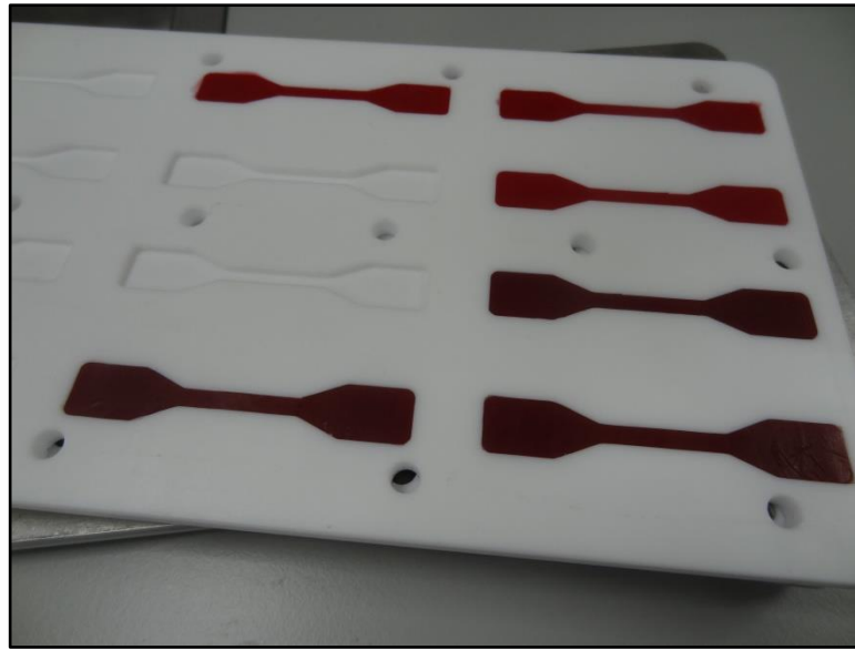
Fig. 4.2: PTFE lined mould for fabrication of dumbbell shaped tensile test specimens.
