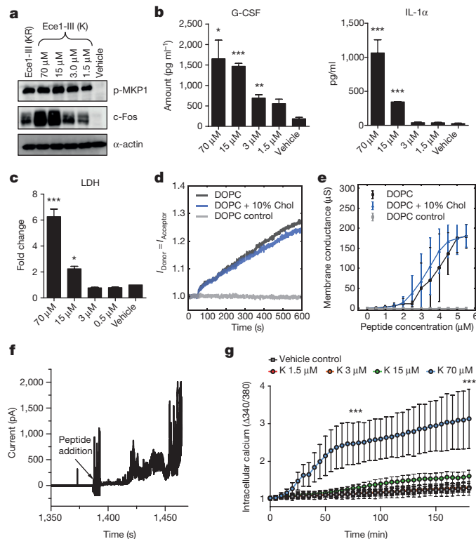
Figure 4 | Ece1-III 62-92K functions as a cytolytic peptide toxin that activates and damages epithelial cells. a–c , Induction of p-MKP-1 and c-Fos 2 h post-stimulation (p.s.) ( a ), secretion of G-CSF and IL-1-α 24 h p.s. ( b ), and LDH release 24 h p.s. of TR146 cells with Ece1-III 62-92K ( c ). d , Förster resonance energy transfer (FRET) showing intercalation of Ece1-III 62-92K (10 μM) into lipid liposomes. e , Average peptide concentration-dependent changes in conductance of tethered lipid membranes. f , Ece1-III 62-92K (4 μM) induced permeabilization of planar lipid membranes showing heterogeneous and transient lesions leading to membrane rupture. g , Intracellular calcium level kinetics in TR146 cells p.s. with Ece1-III 62-92K . Data shown are representative ( a , d , f ) or mean ( b , c , e , g ) of three biological replicates. Error bars show ± s.e.m. Data are analysed by one-way ANOVA ( b , c ). * P < 0.05, ** P < 0.01, *** P < 0.001 (compared with vehicle control). For gel image, see Supplementary Fig. 1.
