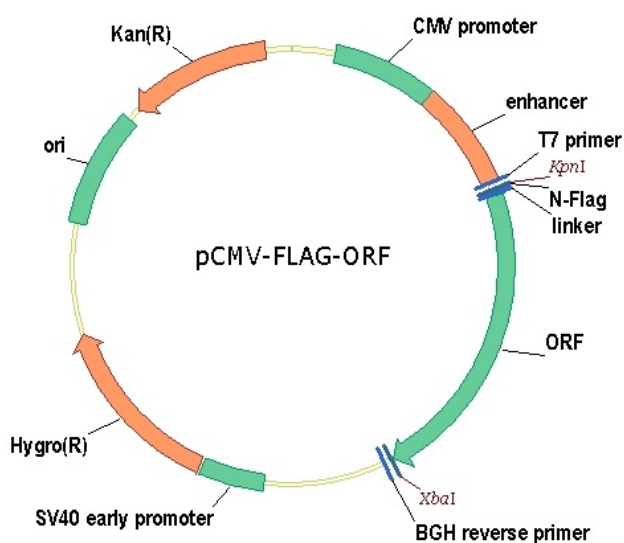
Figure 2.3 - pCMV-FLAG-ORF backbone map
