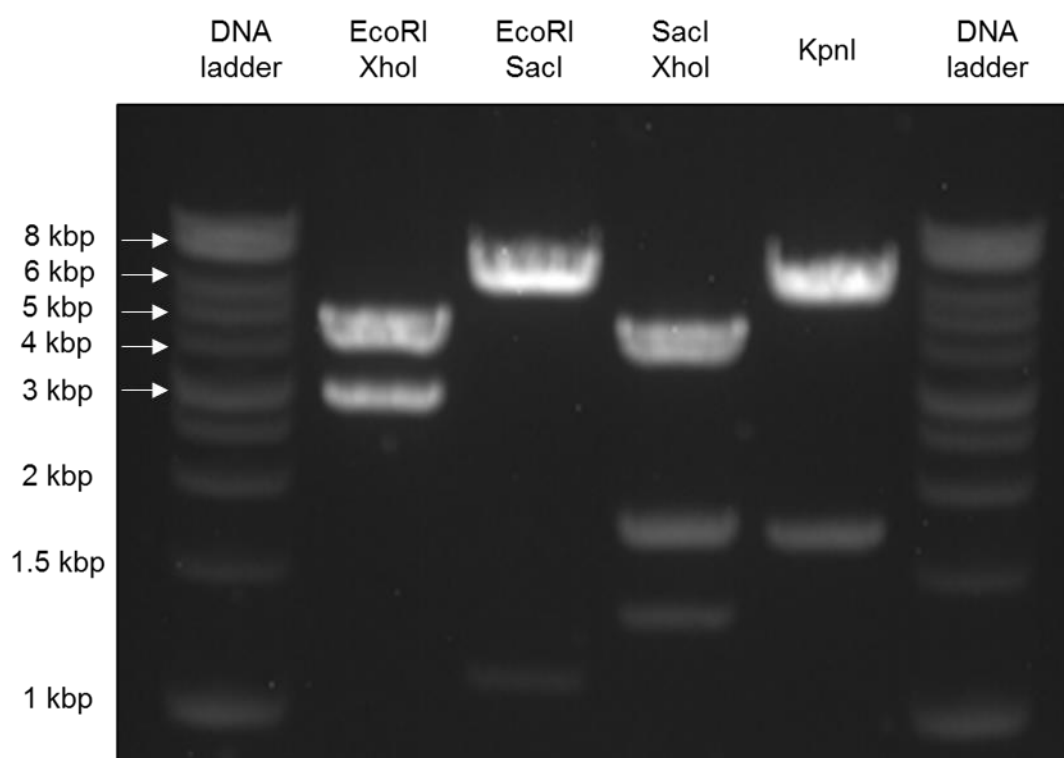
Figure 4.19: DNA gel electrophoresis of DNMT3A maxiprep sample.
