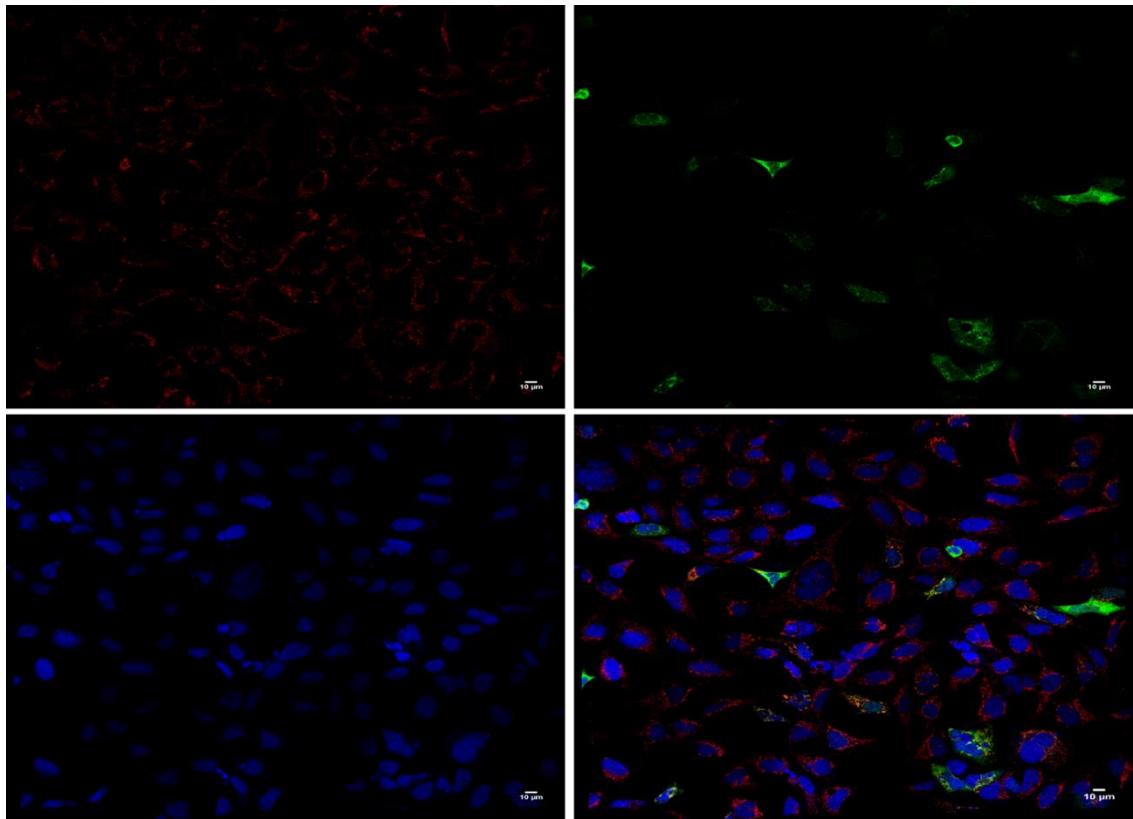
Figure 4.26: Immunocytochemistry of HEK293A cells transfected with pCMV-SPORT6-mitochondrial DNMT1 (big picture of 9 images). Cells have been stained for mitochondria (ATP synthase, top left), HA-tag (Alexafluor 488, top right) and nuclei (DAPI, bottom left). Bottom right is a merged image of all channels. Scale bar = 10 \mu m.
