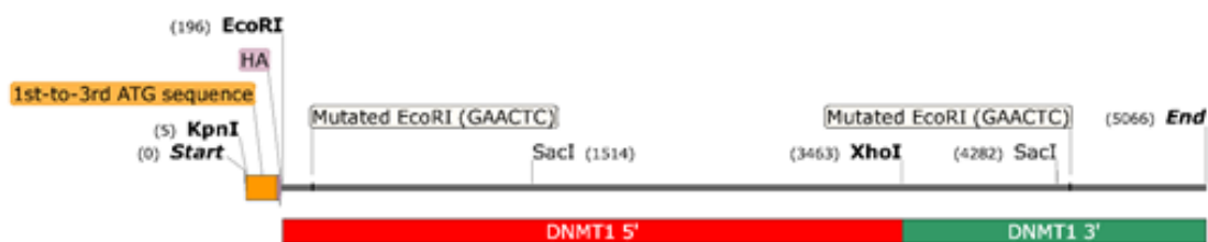
Figure 3.23: General scheme of DNMT1 digestion sites. Strategy #2 cDNA is shown.
