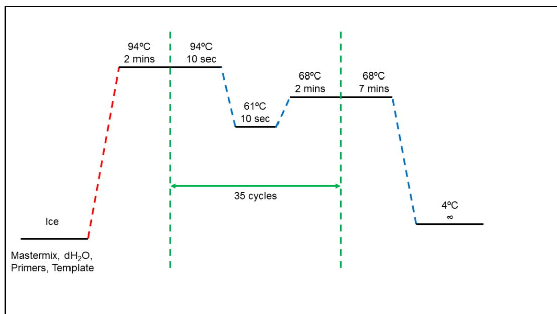
Figure 4.8: Conditions for de novo PCR synthesis of DNMT3A 3' fragment.
