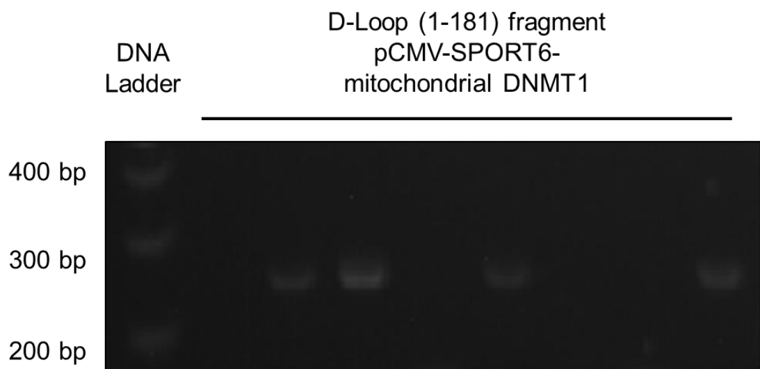
Figure 4.14: Representative DNA gel electrophoresis of TOPO-D-Loop (1-181) miniprep samples (pCMV-SPORT6-mitochondrial DNMT1-transfected DNA).
