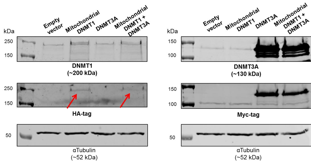
Figure 4.20: Western blotting after overexpression of mitochondrial DNMT1, DNMT3A, and both. αTubulin was used as housekeeping gene.
