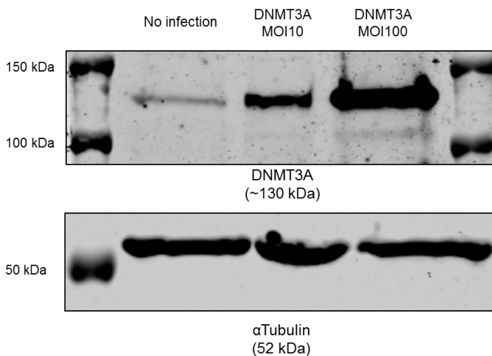
Figure 5.37: Western blotting of H9C2 cells samples infected with Adeno-DNMT3A. Two different multiplicities of infections were investigated. No infection was used as negative control. After infection, strong DNMT3A bands could be observed in all infected sample, especially in MOI 100 samples.
