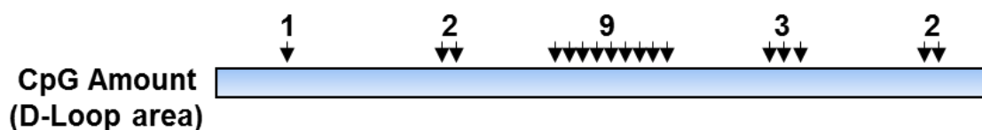
Figure 5.42: CpG amounts for D-Loop areas. Primer set #3 amplifies for the sequence with the highest amount of CpG motifs (9).
