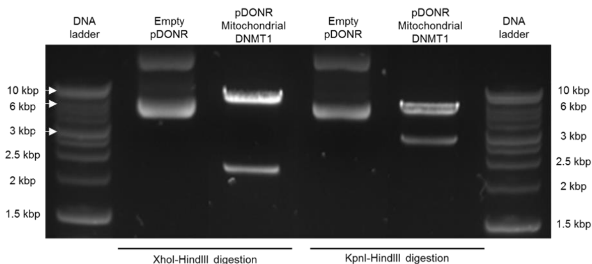
Figure 5.27: DNA gel electrophoresis of empty pDONOR and pDONR-Mitochondrial DNMT1 after BP reaction. After confirming the restriction pattern, the clone was used for LR clonease reaction.
