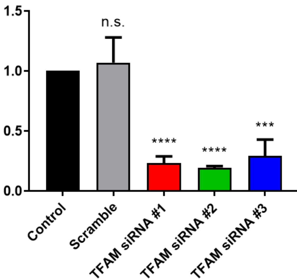
Figure 6.2: Western blot of MCEC samples after 48 hours TFAM knock-down.
