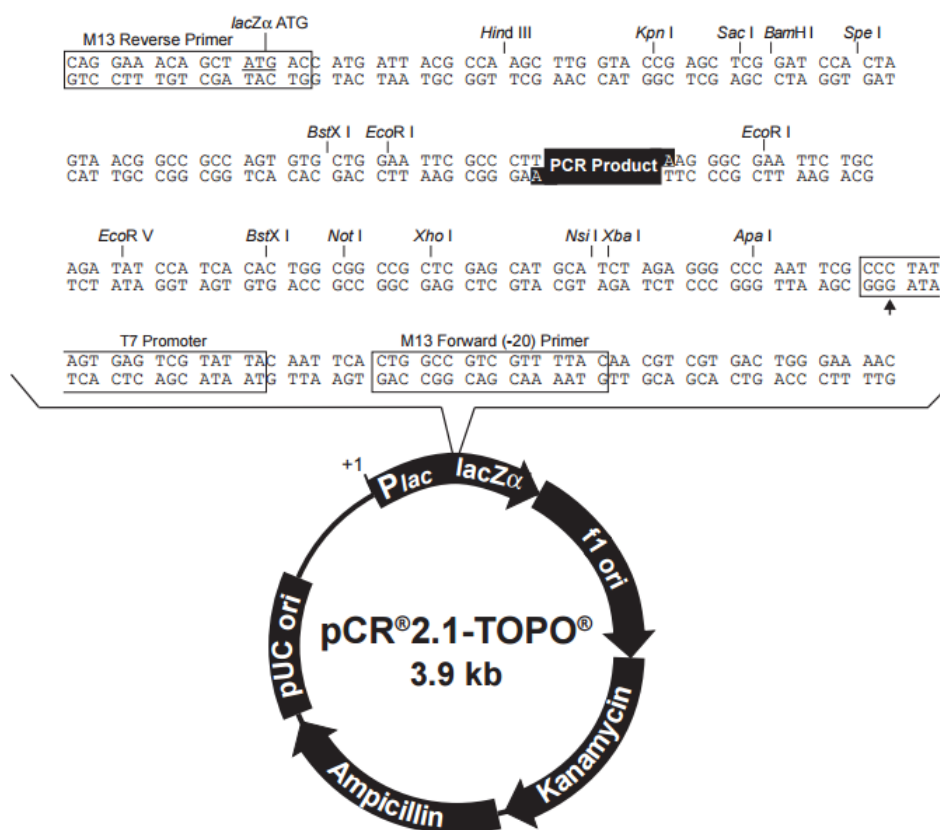
Figure 4.5: pCR 2.1-TOPO vector map. The vector contains sequences for Ampicillin as well as Kamanycin selection. The PCR product is inserted between 2 EcoRI restriction sites, and then sequenced using M13 reverse and forward primers. Taken from Thermo Fisher Scientific®.
