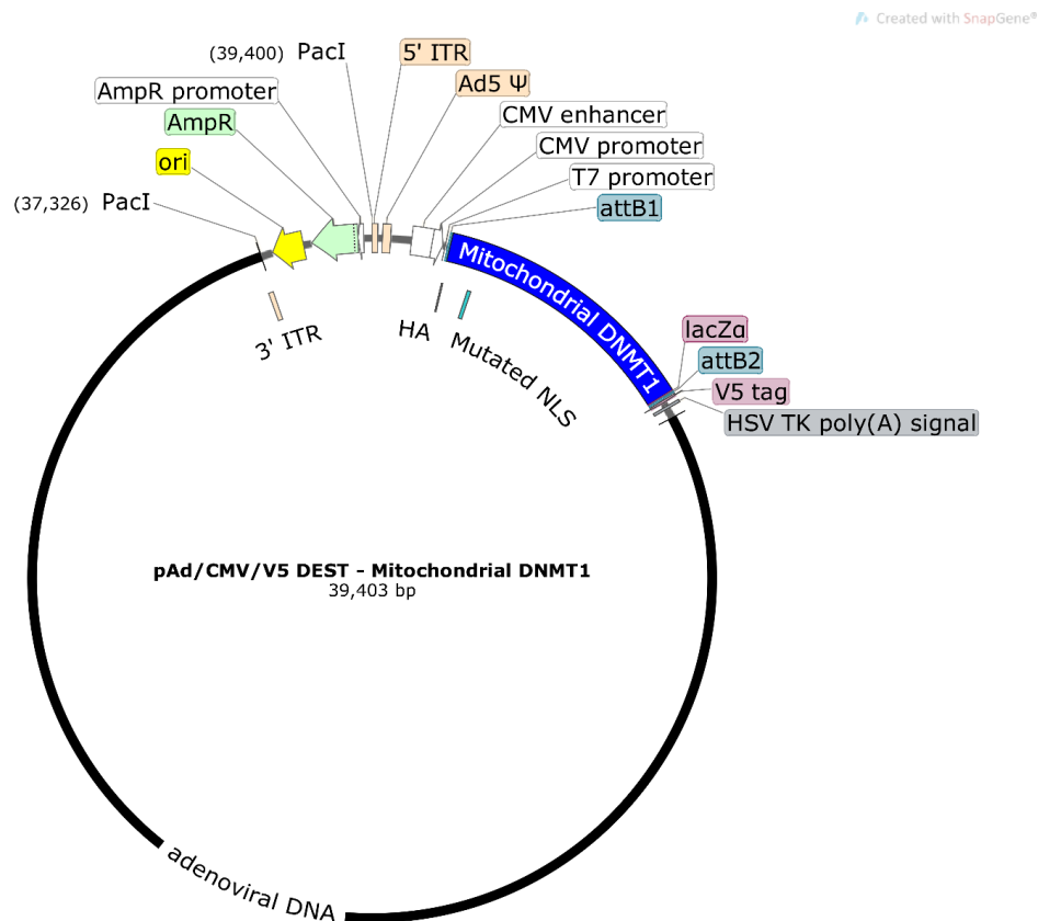
Figure 5.30: pAd/CMV/V5 DEST - Mitochondrial DNMT1 final clone.
