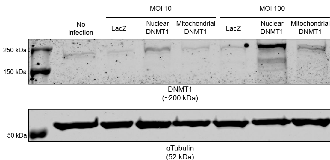
Figure 5.36: Western blotting of H9C2 cells samples infected with Adeno-Nuclear DNMT1 and Adeno-Mitochondrial DNMT1. No infection, as well as infection with Adeno-LacZ, were used as negative control. Two different multiplicities of infections were investigated. After infection, clear nuclear and mitochondrial DNMT1 bands could be observed in all infected sample, especially in MOI 100 samples.
