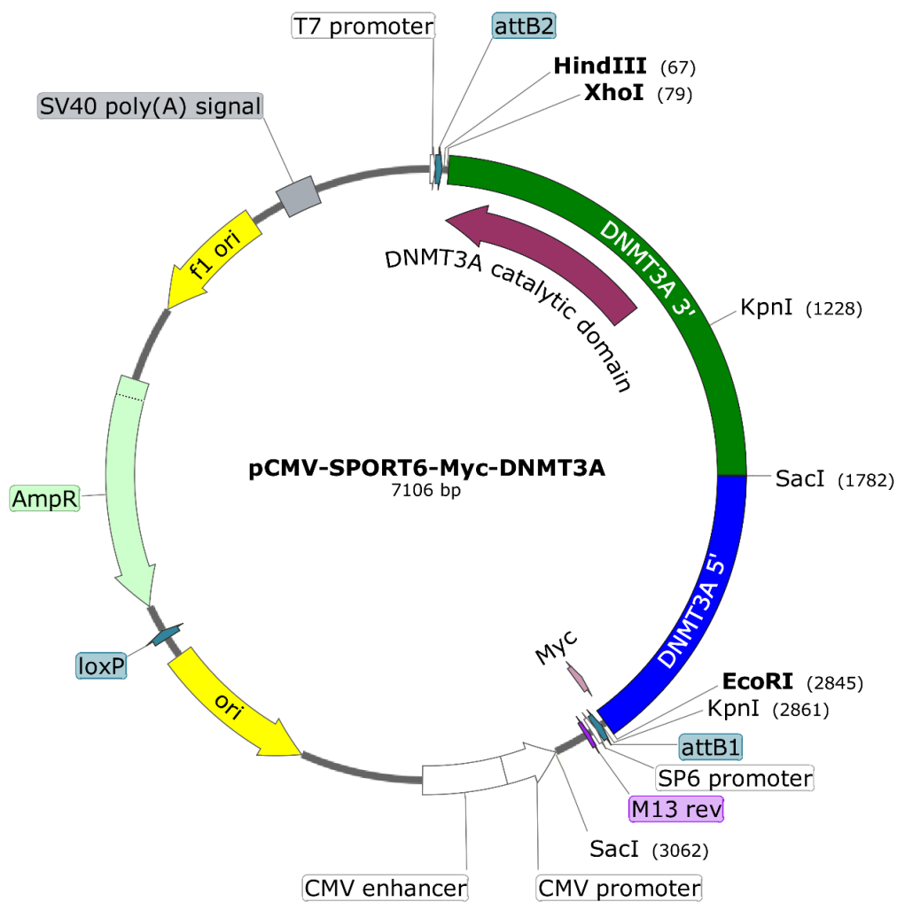
Figure 5.6: Final pCMV-SPORT6-DNMT3A plasmid.
