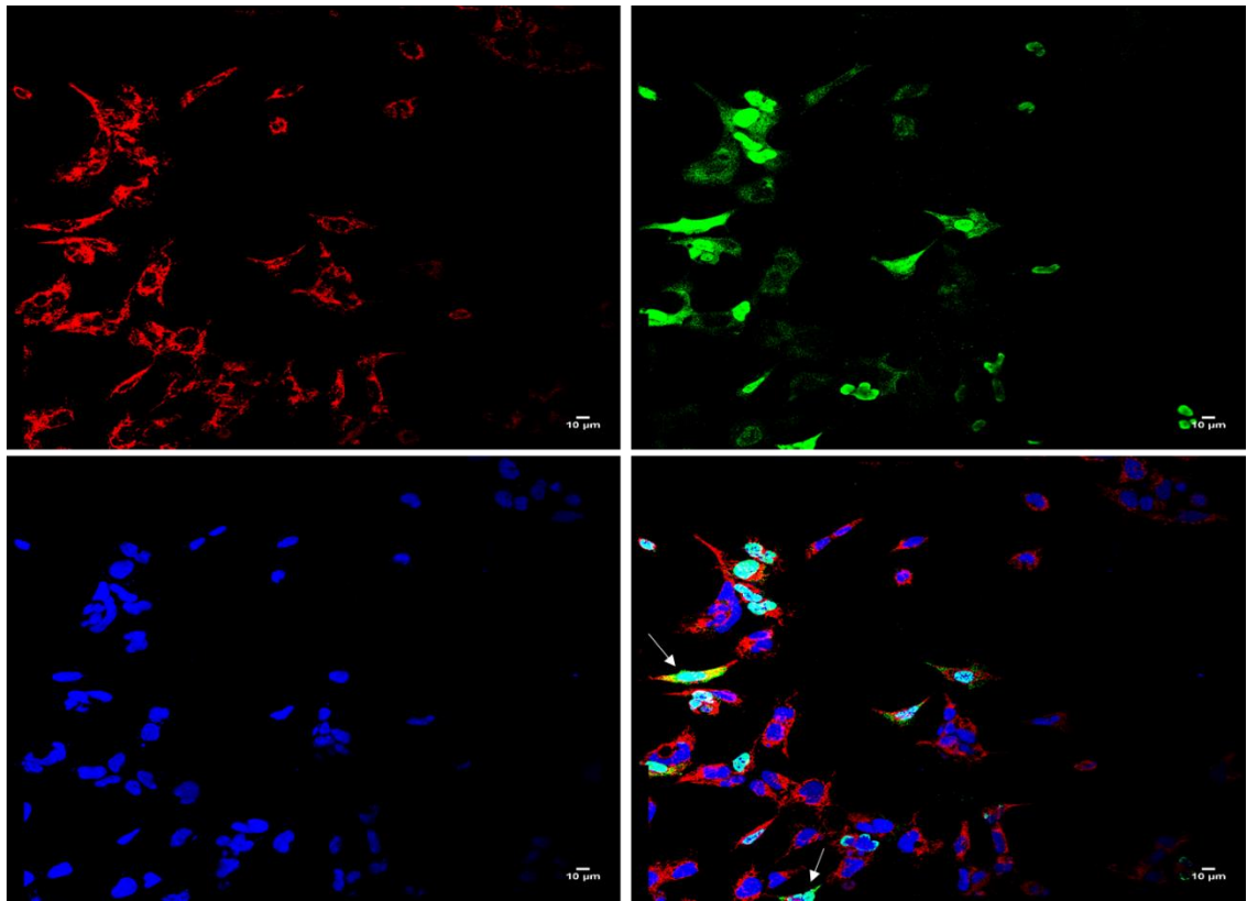
Figure 4.30: Immunocytochemistry of HEK293A cells transfected with pCMV-SPORT6-whole DNMT1 and pCMV-SPORT6-DNMT3A (big picture of 9 images) (DNMT3A staining). Cells have been stained for mitochondria (ATP synthase, top left), Myc-tag (Alexafluor 488, top right) and nuclei (DAPI, bottom left). Bottom right is a merged image of all channels. Scale bar = 10 \mu m.
