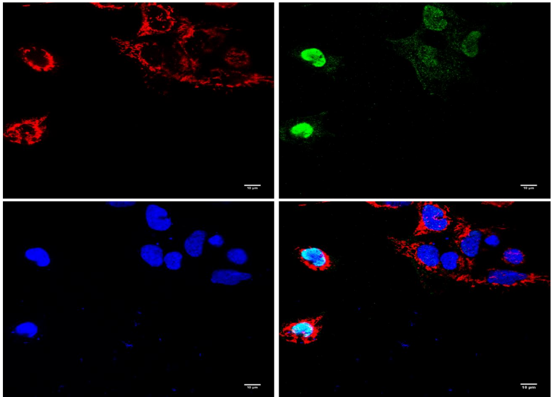
Figure 4.29: Immunocytochemistry of HEK293A cells transfected with pCMV-SPORT6-whole DNMT1 and pCMV-SPORT6-DNMT3A (DNMT3A staining). Cells have been stained for mitochondria (ATP synthase, top left), Myc-tag (Alexafluor 488, top right) and nuclei (DAPI, bottom left). Bottom right is a merged image of all channels. Scale bar = 10 \mu m.
