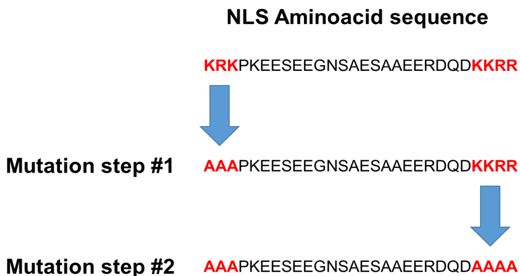
Figure 3.8: Changes in NLS amino acid sequence.
