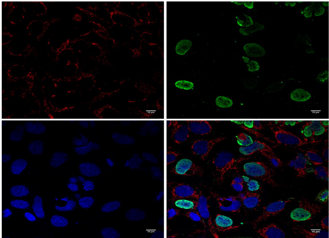
Figure 4.33: Immunocytochemistry of HEK293A cells transfected with pCMV-SPORT6-mitochondrial DNMT1 and pCMV-SPORT6-DNMT3A (DNMT3A staining). Cells have been stained for mitochondria (ATP synthase, top left), Myc-tag (Alexafluor 488, top right) and nuclei (DAPI, bottom left). Bottom right is a merged image of all channels. Scale bar = 10 \mu m.
