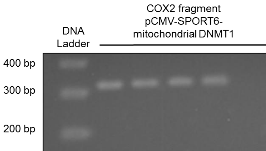
Figure 4.11: Representative DNA gel electrophoresis of TOPO-COX2 miniprep samples from pCMV-SPORT6-mitochondrial DNMT1 transfected DNA.
