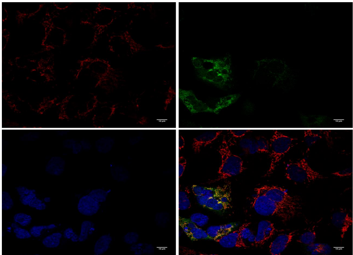
Figure 4.25: Immunocytochemistry of HEK293A cells transfected with pCMV-SPORT6-mitochondrial DNMT1. Cells have been stained for mitochondria (ATP synthase, top left), HA-tag (Alexafluor 488, top right) and nuclei (DAPI, bottom left). Bottom right is a merged image of all channels. Scale bar = 10 µm.
