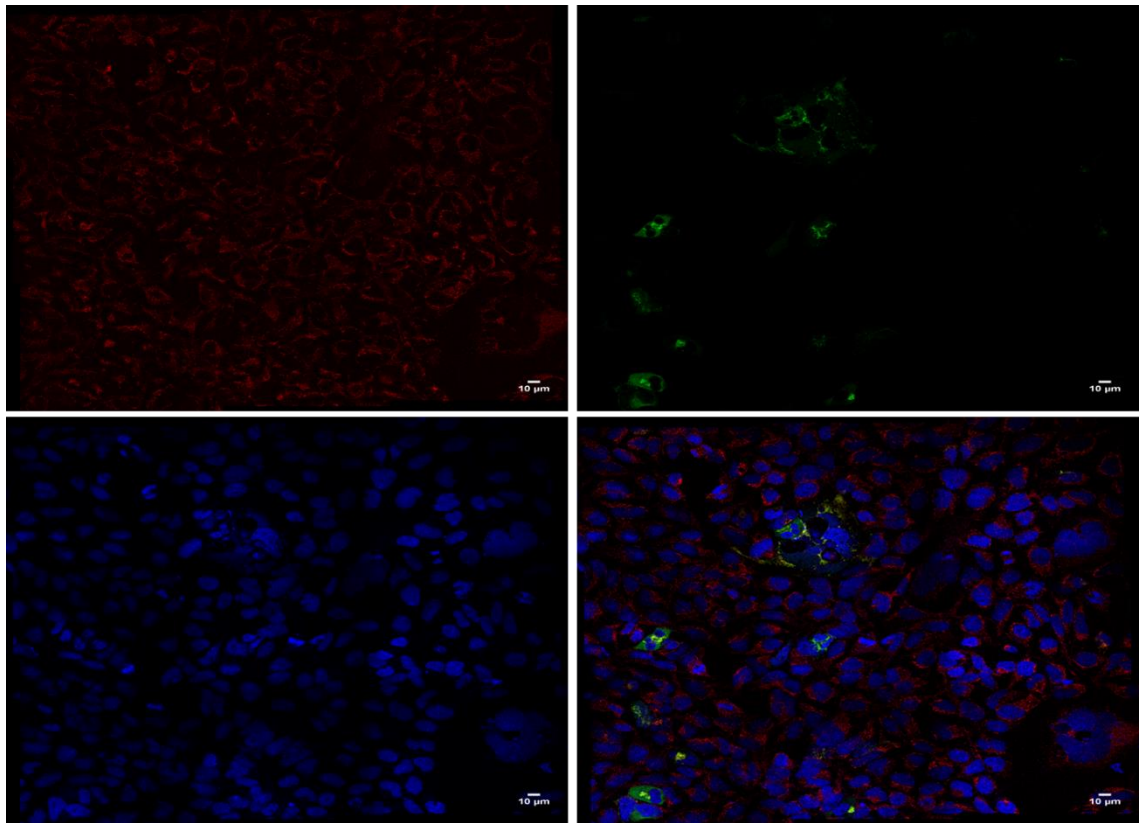
Figure 4.32: Immunocytochemistry of HEK293A cells transfected with pCMV-SPORT6-mitochondrial DNMT1 and pCMV-SPORT6-DNMT3A (big picture of 9 images) (DNMT1 staining). Cells have been stained for mitochondria (ATP synthase, top left), HA-tag (Alexafluor 488, top right) and nuclei (DAPI, bottom left). Bottom right is a merged image of all channels. Scale bar = 10 µm.
