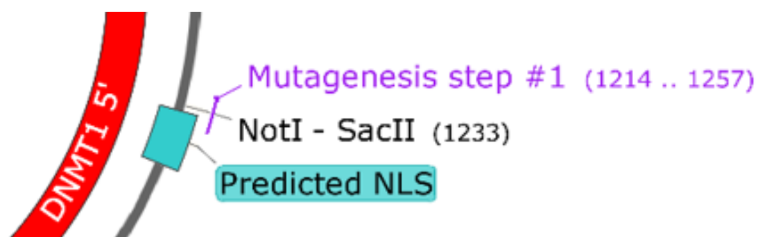
Figure 3.30: First step of NLS mutagenesis.
