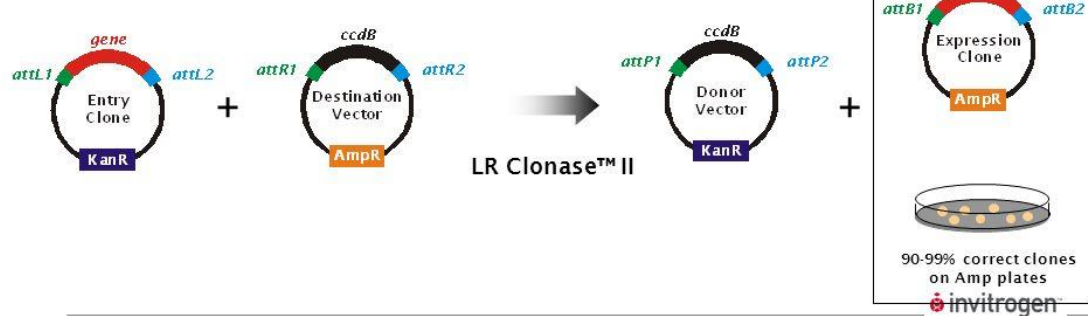
Figure 5.7: Gateway® workflow for creation of adenoviral vectors. The workflow is divided in 2 main steps: in the BP clonase step, the sequence of interest is inserted in an “entry clone” vector and amplified through miniprep. Then, the entry clone plasmid is used in the LR clonase step to obtain the final expression clone. The same workflow was applied for all constructs.
