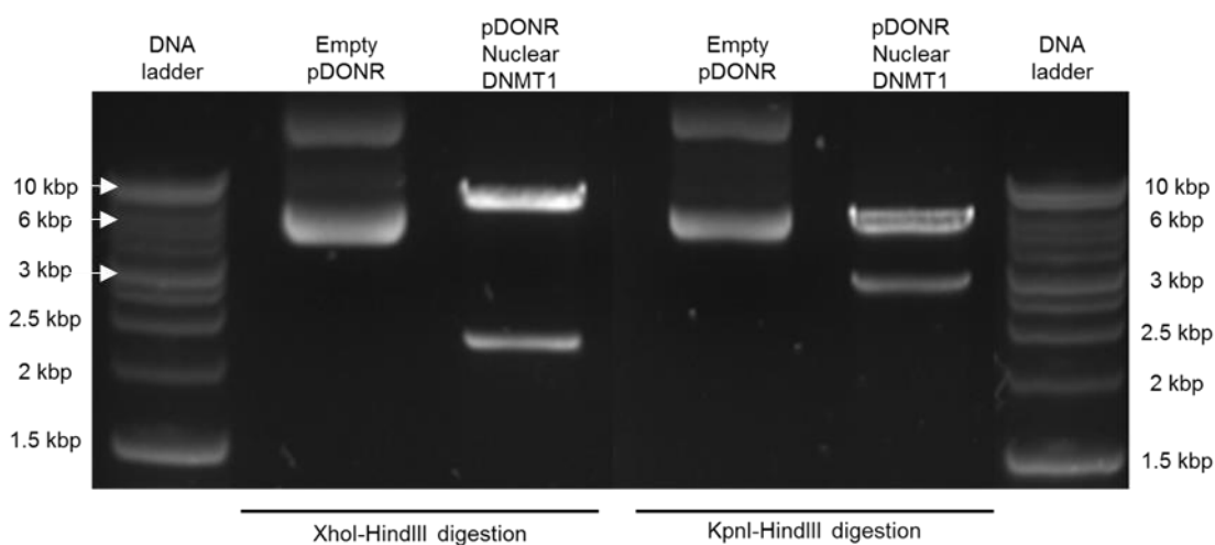
Figure 5.26: DNA gel electrophoresis of empty pDONOR and pDONR-Nuclear DNMT1 after BP reaction. After confirming the restriction pattern, the clone was used for LR clonease reaction.
