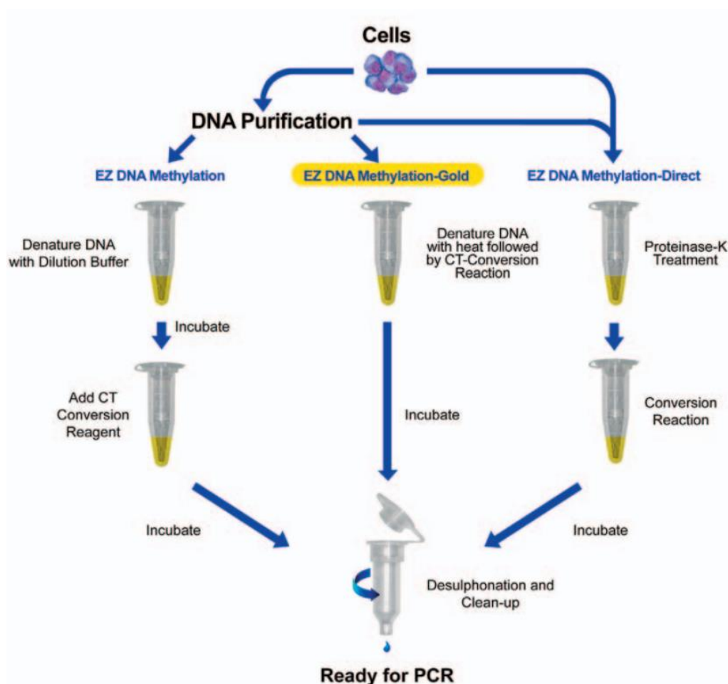
Figure 4.3: Bisulphite treatment workflow. For this project, the EZ DNA Methylation Gold Kit was used. Figure taken from Zymo Research®.
