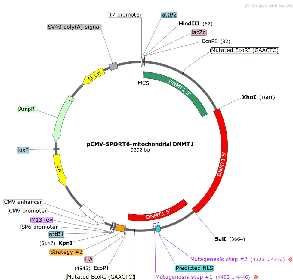
Figure 3.33: Insertion of 5' fragment with mutated NLS in pCMV-SPORT6.
