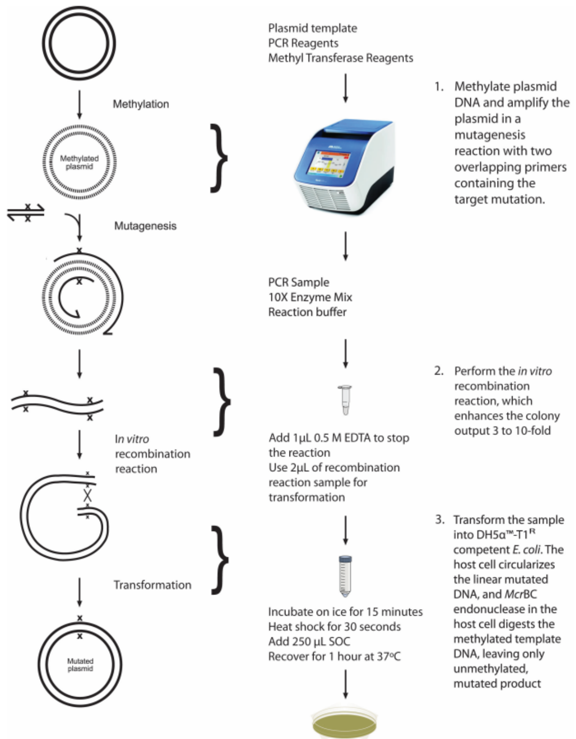
Figure 3.7: General workflow of Geneart site-directed mutagenesis kit. Figure taken from Invitrogen Life Sciences®.
