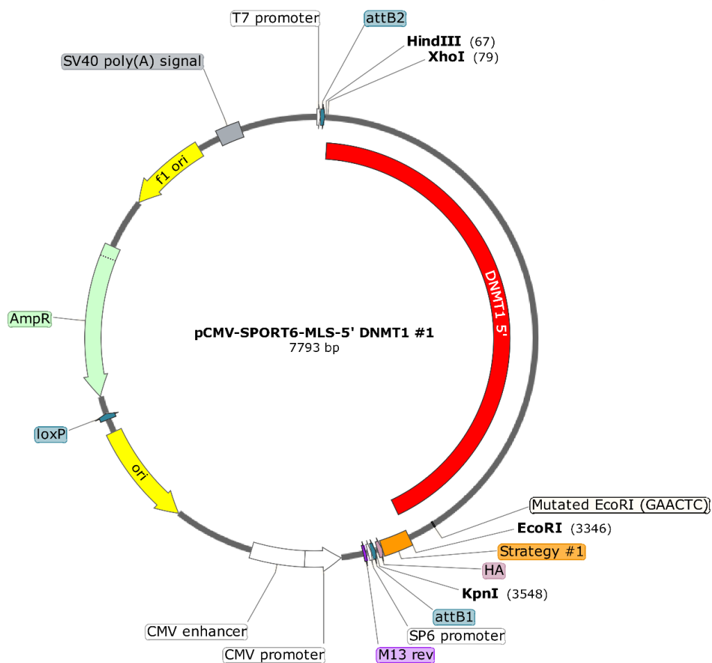
Figure 3.19: Insertion of the Strategy #1 PCR product in pCMV-SPORT6 vector carrying the 5' DNMT1 fragment.
