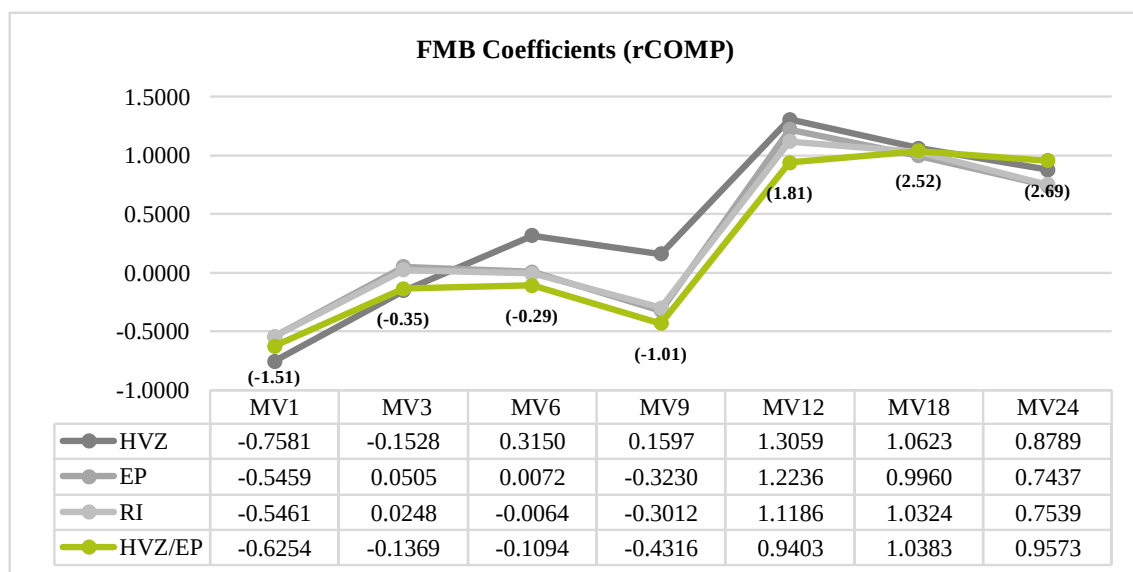
Figure 4.6: Fama-MacBeth Coefficients
