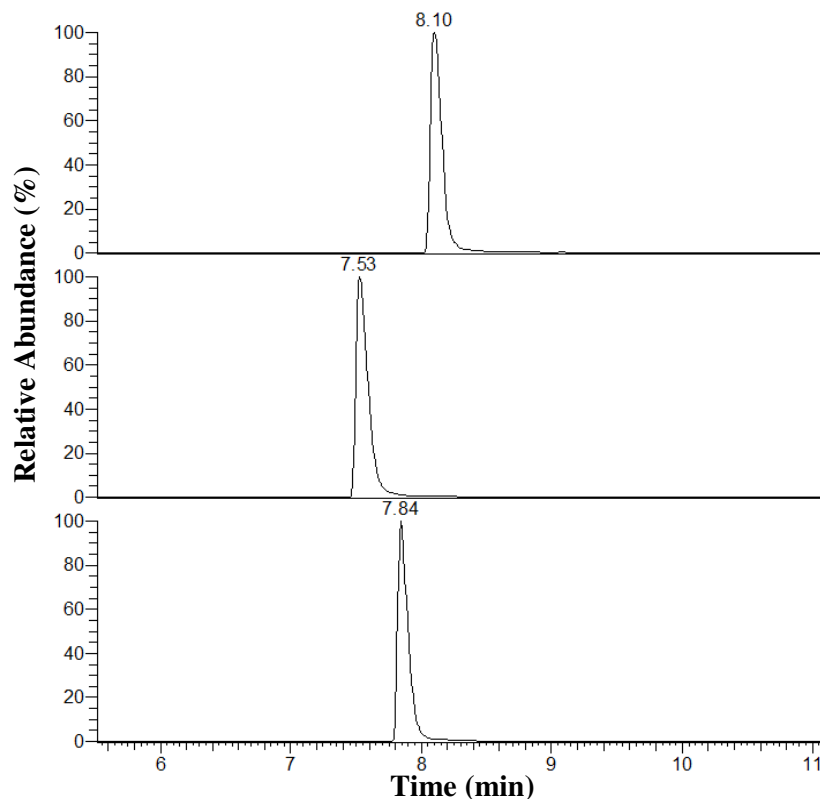
Figure 3.18 – Extracted ion chromatograms ( m/z 248.1641) for a) the patient urine sample, b) methoxetamine reference standard, and c) pethidine reference standard.
