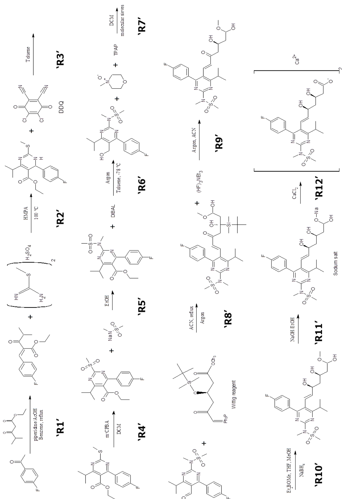
Figure 5.1: Reaction scheme for route synthesis of rosuvastatin calcium expanded to illustrate the reaction stages (R(#)) monitored by UPC 2 /MS and UPLC/MS
