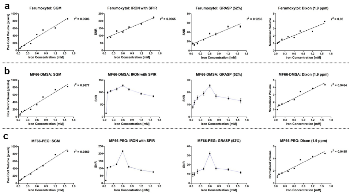
Figure 85: Relationship of positive contrast and SPION concentration for SGM, GRASP, IRON, and Dixon fat image for ferumoxytol (a), MF66-DMSA (b), and MF66-PEG (c). A linear relationship is observed for ferumoxytol whereas GRASP and IRON for MF66-DMSA and MF66-PEG behave in a non-linear fashion.
