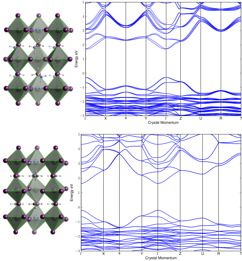
Figure 4.6: The unit cells and QSGW electronic band structures for tetragonal (top) and orthorhombic (bottom) MAPI phases (unit cell figures obtained from reference [132]).
