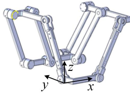
Figure 7.5 The motion branch II with two parallelograms and no connotative parallelograms
