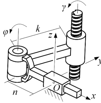
(b) PRH kinematic chain
