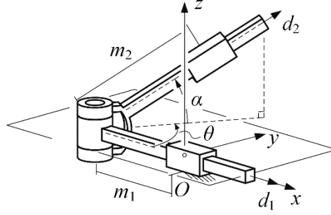
(a) PRP chain with a tilting angle \alpha
